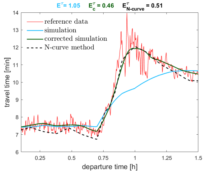
Figure 6.13: SUMO-2 . 1^{st} - Godu - \rho, \mathbf{L}^2 approach. \mathbf{E}_{GP}^\tau = 0.81 , \mathbf{E}_{baseline}^\tau = 0.62 . Travel time estimation results.
