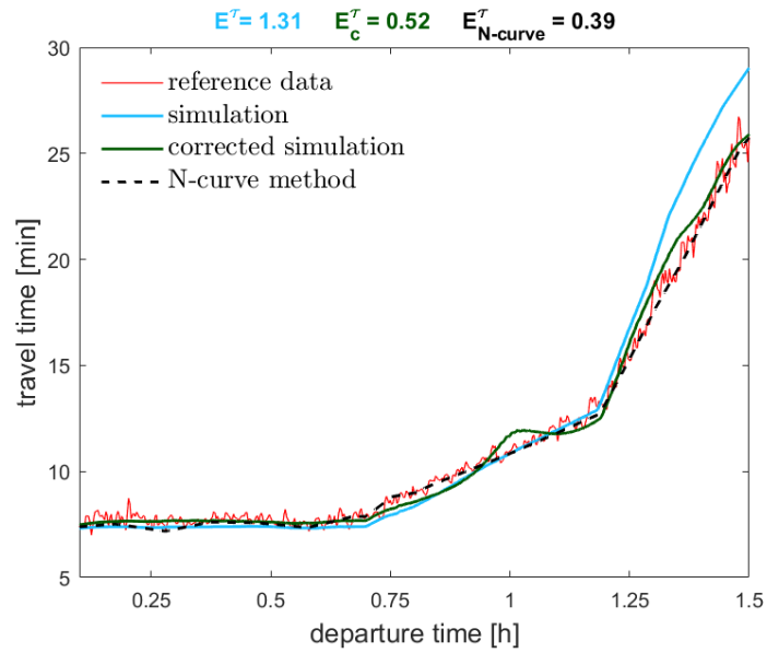
Figure 6.12: SUMO-1B . 1^{st} - Godu - \rho, \mathbf{L}^2 approach. \mathbf{E}_{GP}^\tau = 0.53 , \mathbf{E}_{baseline}^\tau = 0.67 . Travel time estimation results.
