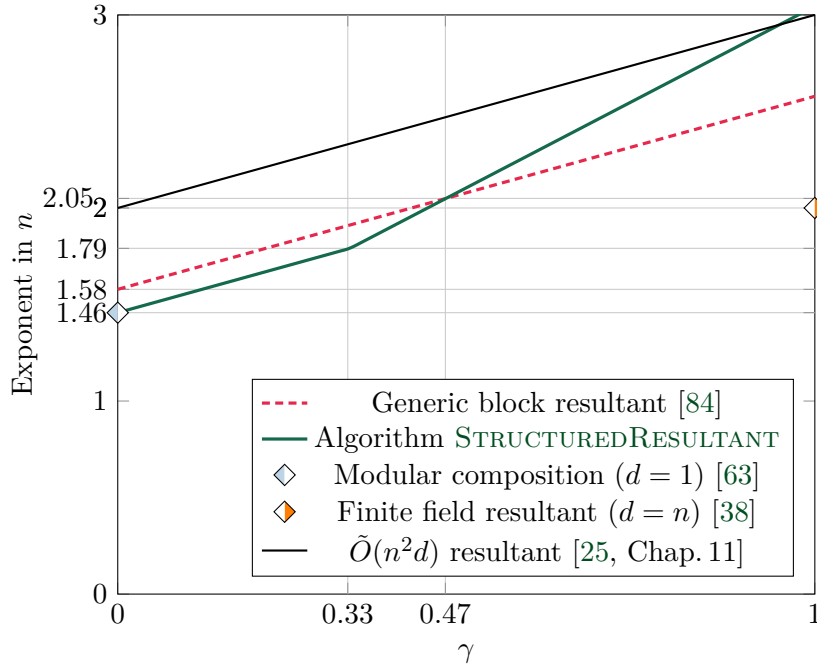
Figure 3.1: Comparison of known asymptotic cost bounds for the resultant of generic polynomials. Exponents in n with d = n^\gamma and \omega = 2.373 .
