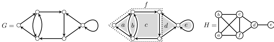
Figure 5.2: An example of a digraph G (left), the simple cycles on G (middle) and the corresponding hike dependency graph H (right).
