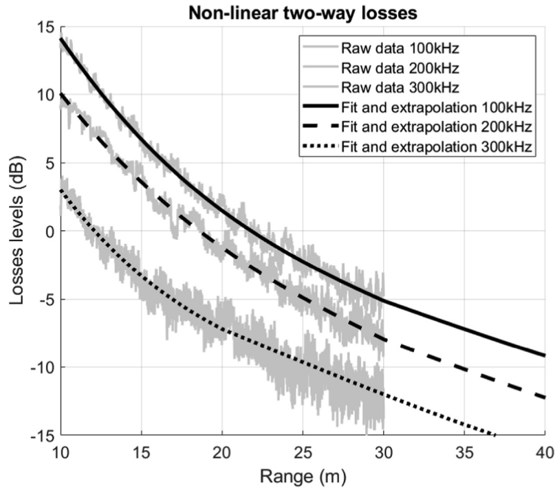
Fig. 5. Grey: measurements of G(f) + \mathcal{L}(f, r) in the large tank of Ifremer (sea water) according to the range from the echosounder in operational mode (i.e. with the maximum level at emission). Black: best-fitting curves used as look-up tables.
