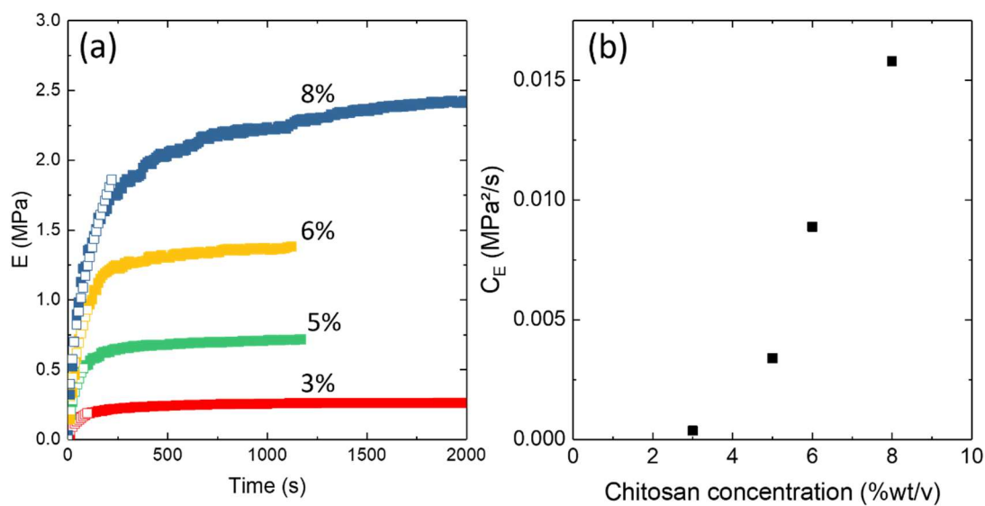
Figure III.9. (a) Comparison of the modulus as a function of time obtained experimentally (close points) and by interpolation (open points) up to 70% of the maximum modulus according to eq. III.2. (b) Coagulation coefficient C_E as a function of the chitosan concentration.
