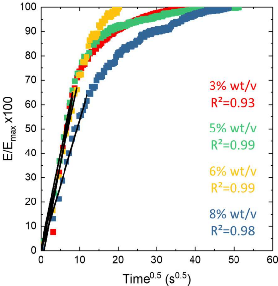
Figure III.7: Evolution of the normalized modulus as a function of time^{0.5} for all concentrations. The dark lines are the linear regressions of the curves up to 60% of the normalize modulus, the R^2 for each line is indicated on the graph.
