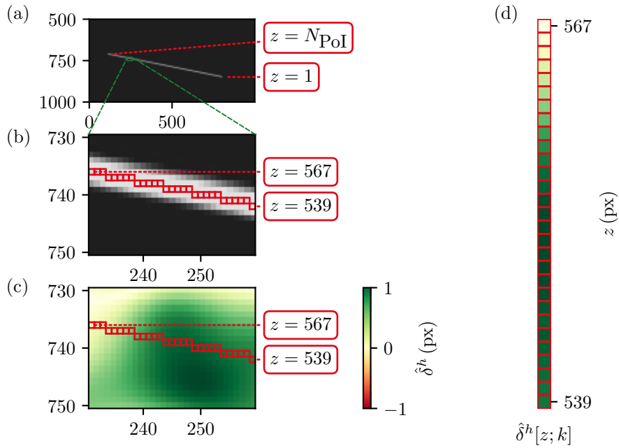
Figure 2.8: Motion extraction process of a cantilever beam. (a) Frame of a synthetic video. (b) Focus on pixels of interest in red with z \in [539, 567] . (c) Estimated motion \hat{\delta}^h[z; k] in the focus view. (d) Estimated motion \hat{\delta}^h[z; k] at the pixels of interest.
