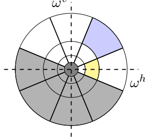
Figure 2.1: Ideal spatial frequency plane decomposition, with N_r = 3 scales and N_\theta = 4 orientations. The yellow and blue parts respectively correspond to the complex filters \hat{G}_{2,0} and \hat{G}_{1,\pi/4} amplitude supports. The bottom light gray part is redundant with the upper part and is thus not processed. The dark gray part is the low-frequency residual.
