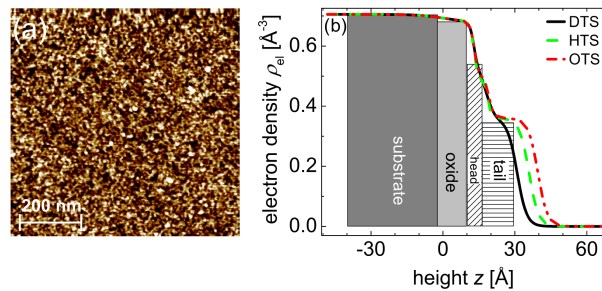
Figure 2.2: (a) AFM of an OTS SAM surface, with the color scale representing a total vertical range of 1 nm. (b) Electron density as a function of depth normal to the substrate-air interface for the SAMs indicated in the legend. Images from Ref. [74].
