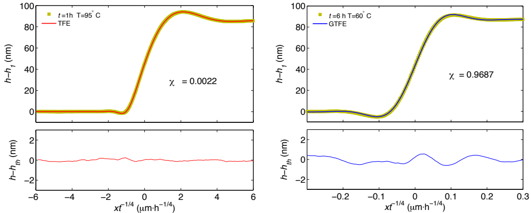
Figure 3.5: [left] Self-similar profile of a stepped film leveling above T_g = 70 \pm 3 °C (see legend) and with \{h_1, h_2\} = \{23, 90\} nm. The solid line is a fit to the TFE, Eq. 2.1. [right] A film with identical geometry yet annealed below T_g and fit using the integration of the GTFE Eq. 3.4. Reproduced from Ref. [157].
