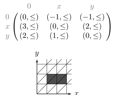
Figure 2.1: A DBM (above) representing the set 1 \leq x \leq 3 \wedge 1 \leq y \leq 2 , shown below.
