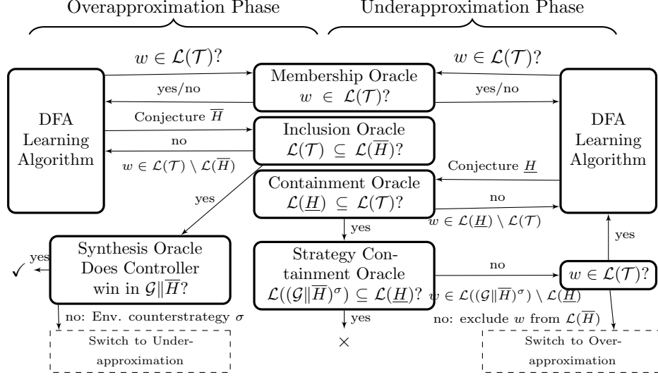
Figure 2.9: The learning-based compositional controller synthesis algorithm for the input timed game \mathcal{G}\|\mathcal{T} , with \mathcal{G} a Controller-silent finite game, and \mathcal{T} a label-deterministic timed automaton. Two automata learning algorithms run in parallel to learn under- and over-approximations \underline{H} and \overline{H} such that \underline{H} \subseteq \mathcal{L}(\mathcal{T}) \subseteq \overline{H} .
