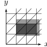
Figure 2.7: An IEDBM (above) representing the parametric set 1 \leq x \leq 3 + 2\delta \wedge 1 - \delta \leq y \leq 2 + 3\delta . The set is represented (below) for \delta = 0.15 .
