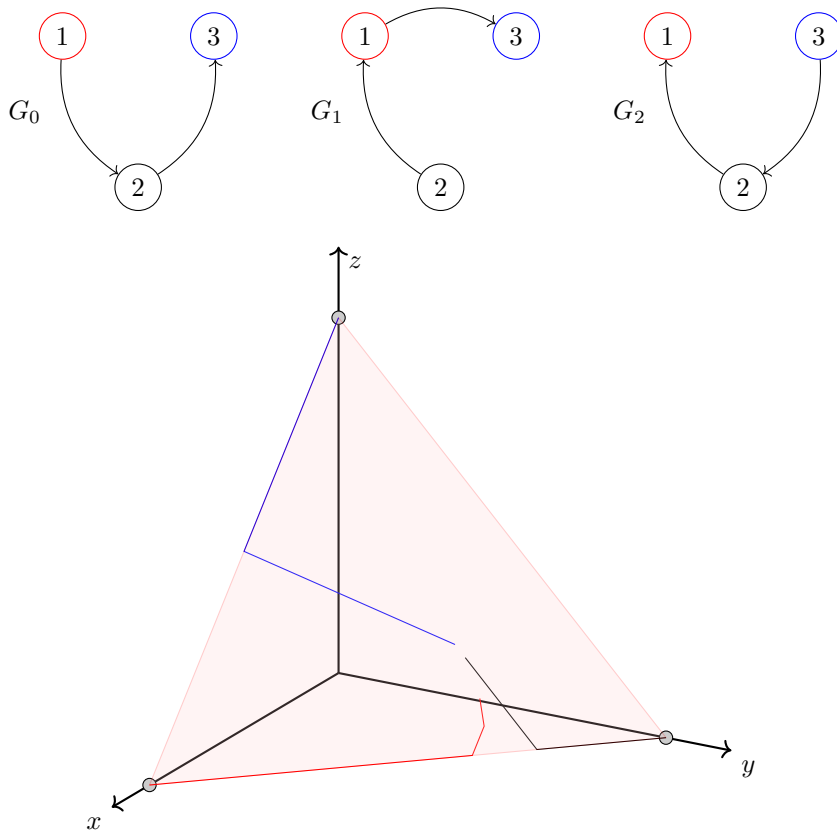
Figure 4.5: A system of N = 3 nodes with node states from dimension d = 3 . The figure shows the outputs of the three nodes during a prefix of an execution of the equal neighborhood algorithm for T = 5 rounds. The communication graphs were chosen uniformly at random from the network model shown at the top of the figure.
