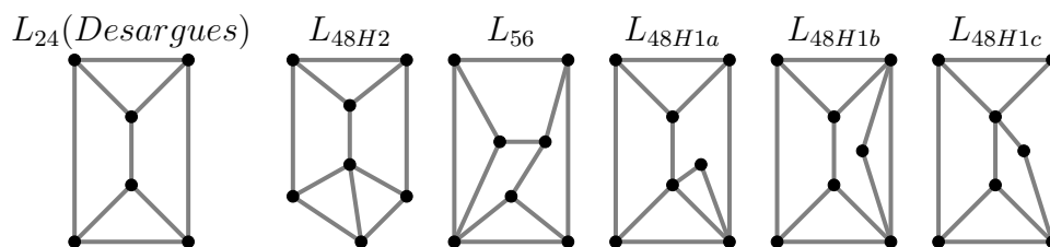
Figure 5.5: Laman graphs with maximal numbers of spherical embeddings with 6 vertices ( L_{24} - Desargues graph with 32 spherical embeddings) and 7 vertices ( L_{48H1a}, L_{48H1b}, L_{48H1c}, L_{48H2} and L_{56} - graphs with 64 spherical embeddings).
