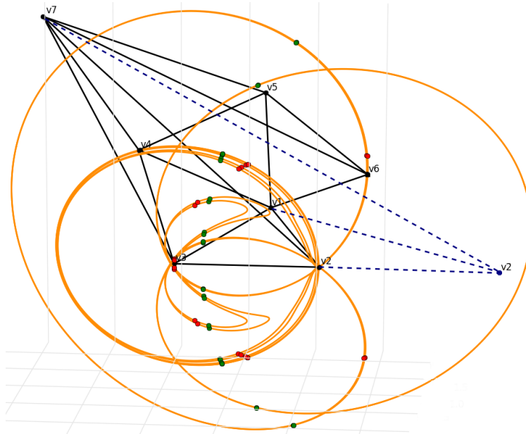
Figure 5.3: The coupler curve C_{v_6, \lambda} of G_{48} with the edge v_2v_6 removed. The 28 red points are intersections of C_{v_6, \lambda} with the sphere centered at v_2 with the edge lengths \lambda , whereas the 32 green ones are for the adjusted edge lengths (illustrated by blue dashed lines).
