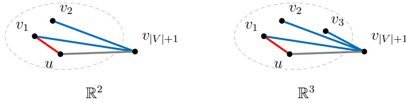
Figure 2.2: J_{|V|+1} is constructed by an H1 step applied to J_{|V|} (blue edges), extended with the edge (u, v_{|V|+1}) . This is equivalent with applying an H2 step and adding the deleted edge (u, v_{|V|+1}) .
