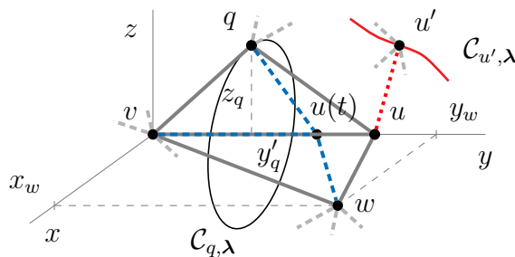
Figure 5.2: Since the lengths of \lambda_{u,q} and \lambda_{u,w} are changed accordingly to the length of (u, v) (blued dashed edges), the coupler curves C_{q, \lambda'(t)} and C_{u', \lambda'(t)} are independent of t . The red dashed edge (u, u') is removed from G .
