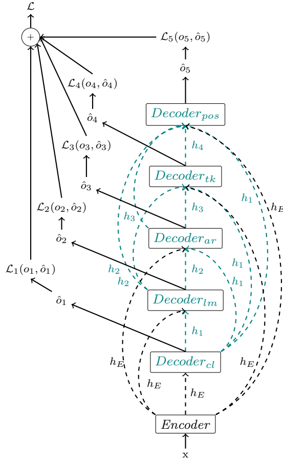
Figure 3.1: A high-level schema of our architecture
