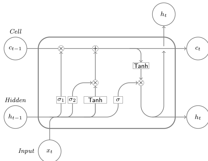
Figure 2.3: Long Short-Term Memory (LSTM) cell.
