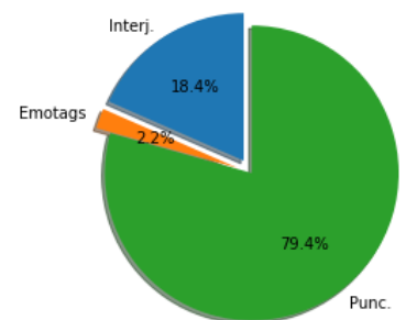
Figure 4.13: Blog
