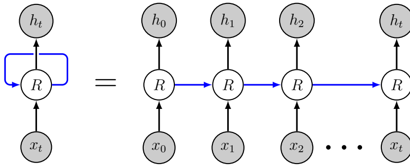
Figure 2.2: Recurrent Network unfolding graph.
