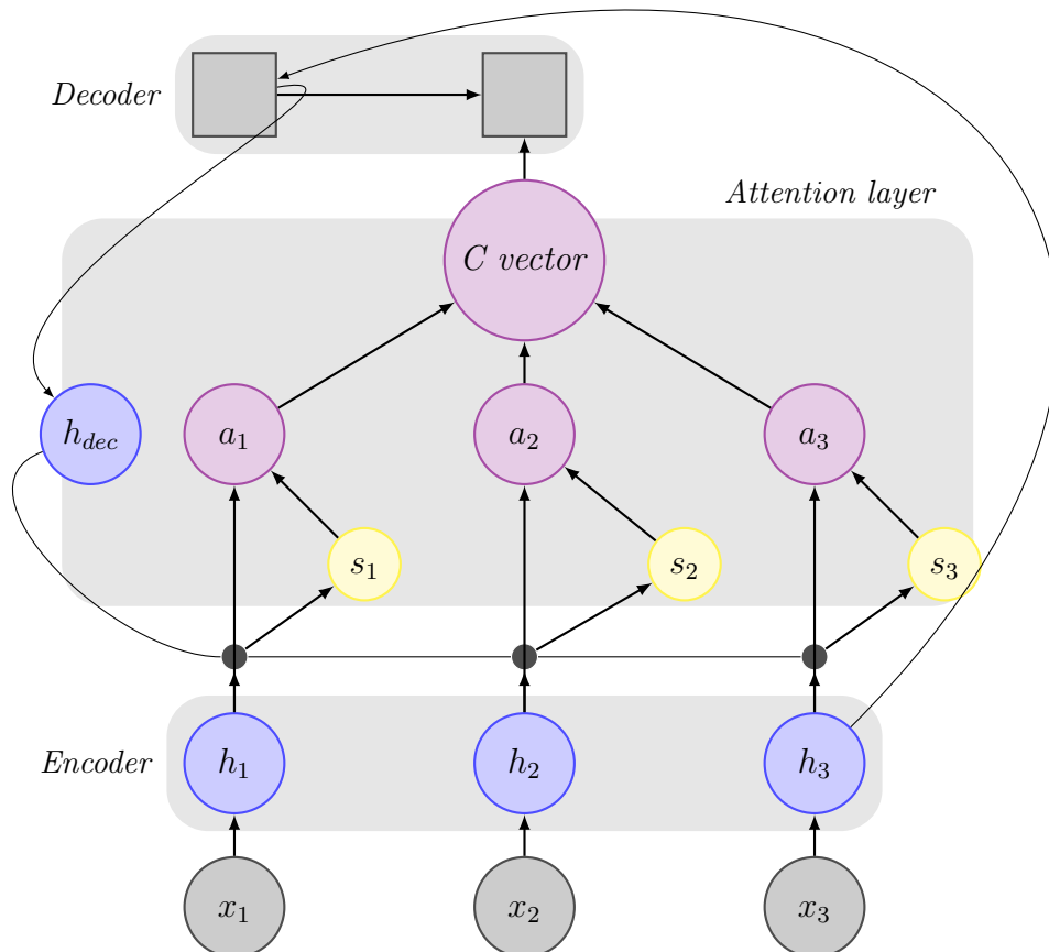
Figure 2.5: Attention mechanism system.
