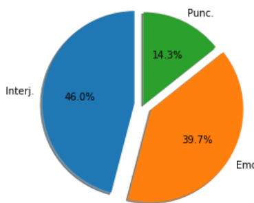
Figure 4.11: Social Net.
