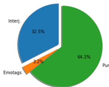
Figure 4.12: Forum
