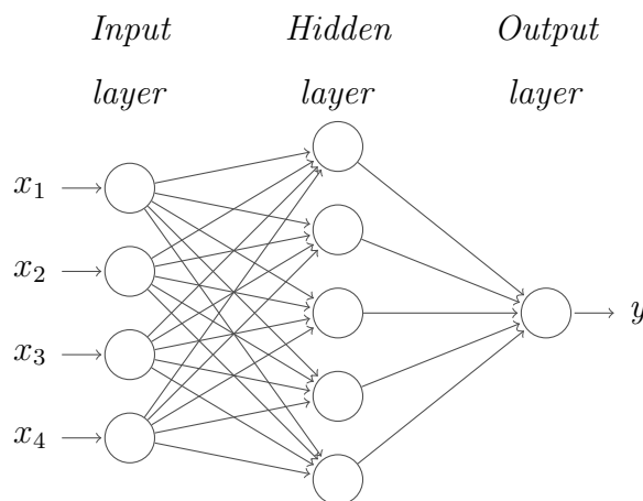
Figure 2.1: Feedforward Network.
