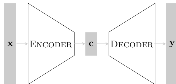
Figure 2.4: Encoder-decoder model.
