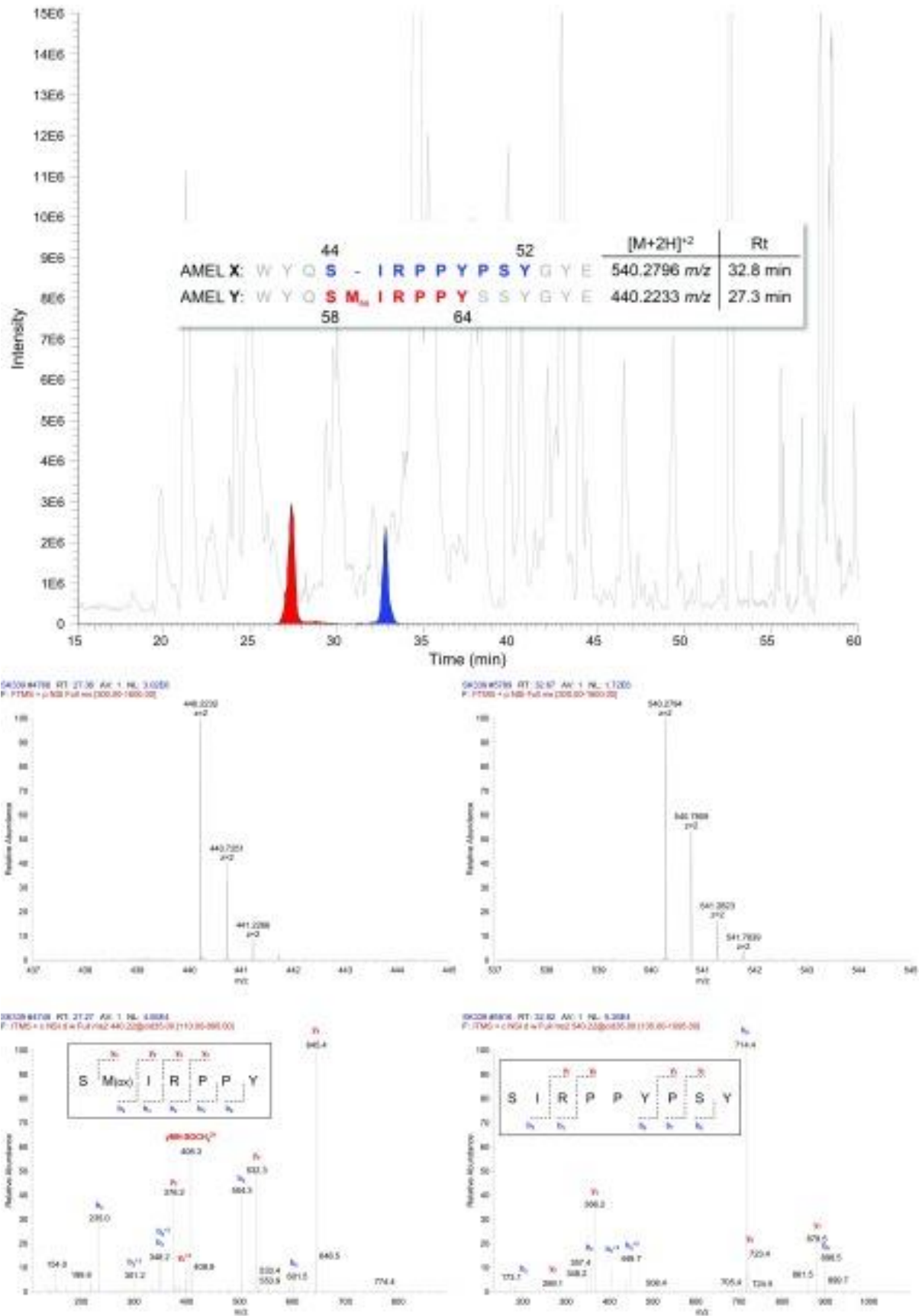
Figure 3. A base peak chromatogram (300–1600 m/z) with two marked peptides of amelogenin: AMELY-[58–64] and AMELX-[44–52]. The reconstructed ion chromatograms (to 4 ppm) for each are shown in
