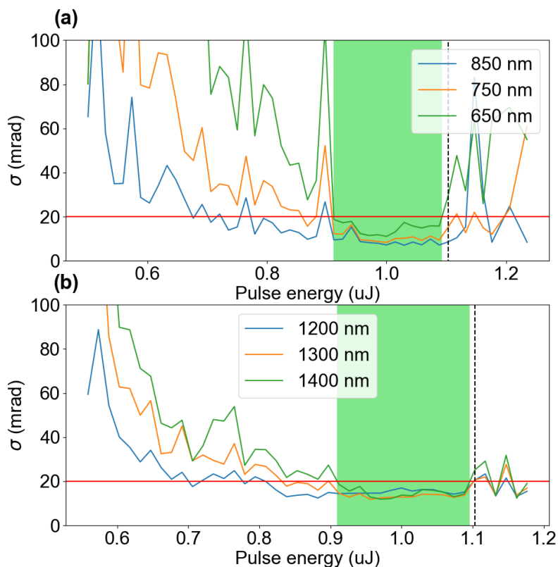
FIGURE 5.11 – Phase standard deviation as a function of seed pulse energy in the short (a) and long (b) wavelength ranges for z = 1.5 mm. The energy axis starts at the onset of filamentation. The dotted black line refers to the onset of double-filamentation. The green areas refer to the stable operating zone.
