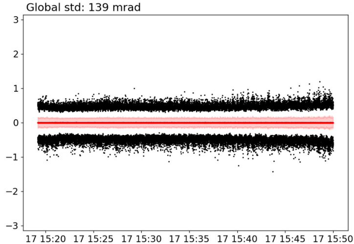
FIGURE 3.14 – CEP of output 2b over 30 seconds with active stabilization.
