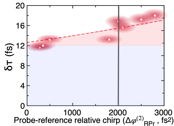
FIGURE 2.12 – \tau_{RP,r} as a function of the chirp difference between the reference and pump/probe pulses, \Delta\varphi_{RP,r}^{(2)} , with fixed input chirp \varphi_p^{(2)} = 5000 \pm 500 \text{ fs}^2 . The colored area refers to 2BC (blue) and frequency-shift (red) contributions.
