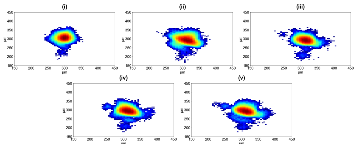
FIGURE 5.18 – Experimental far fields in the center of the measurement range measured with a camera for the five aberrations in logarithmic scale.
