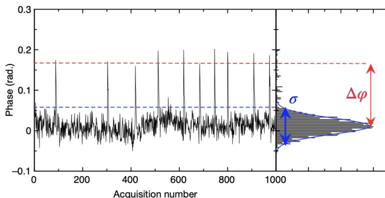
FIGURE 5.9 – Illustration of the significant quantities extracted from the acquisitions : the phase is calculated by Fourier transform for an arbitrarily chosen wavelength as a function of acquisition time for each acquired spectrum. The blue dashed line indicates the threshold applied to filter out the effect of laser overshoots. \sigma is the standard deviation of the measured phase noise, and \Delta\varphi is the phase jump induced by laser overshoots. The process is repeated for each wavelength.
