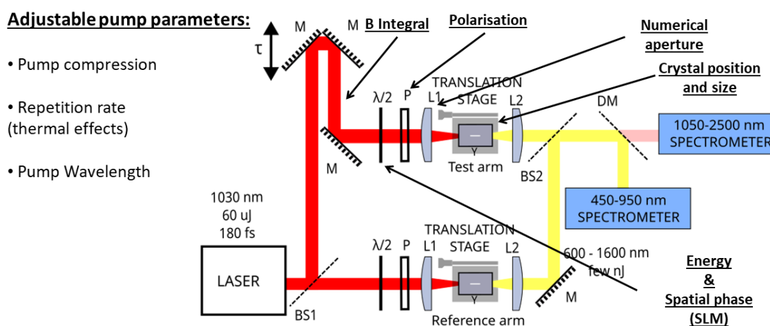
FIGURE 5.1 – Interferometer layout with an array of possible parameters to investigate for the WLG. Parameters to be tuned on the pump laser itself are indicated on the left. Parameters to be tuned on the beam on the test arm itself are underlined around the interferometer.
