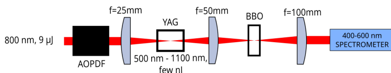
FIGURE 3.13 – Diagram of the f - 2f interferometer.
