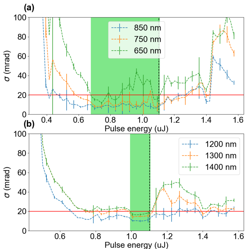
FIGURE 5.10 – Phase standard deviation as a function of seed pulse energy in the short (a) and long (b) wavelength ranges for z = -1.5 mm. The energy axis starts at the onset of filamentation. The dotted black line refers to the onset of double-filamentation. The green areas refer to the stable operating zone.
