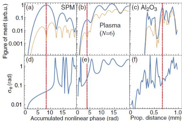
FIGURE 4.1 – Numerical simulations of the intrapulse coherence of supercontinuum pulses. Simulations are based on an ensemble of 1000 input pulses with 10 fs duration and 1% energy standard deviation. (a)–(c) Mean value (thick blue line) and standard deviation (thin orange line) of the FOM. The first maximum of the FOM has been marked by a dashed red line. (d)–(f) Standard deviation of \Delta\varphi . (a), (d) Symmetric spectral broadening due to self-phase modulation. (b), (e) Asymmetric spectral broadening due to plasma generation driven by a multiphoton process of the order of 6. (c), (f) Full simulation of nonlinear propagation in sapphire according to [261].
