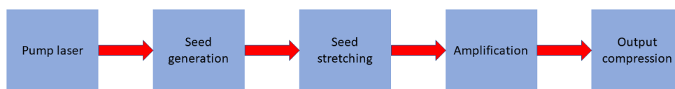
FIGURE 3.5 – Diagram of a typical OPCPA
