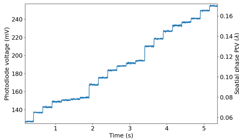
FIGURE 5.22 – Photodiode measurement of the blue writing beam as a function of time showing the increments performed by the DLP unit. The right axis shows the corresponding spatial phase PtV in configuration (ii).
