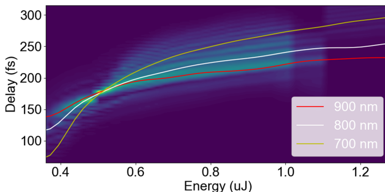
FIGURE 5.14 – Delay curves for three different wavelengths in the short-wavelength range as a function of the pulse energy. The delay curves are plotted on top of a color map representing the first delay peak of the Fourier transform.
