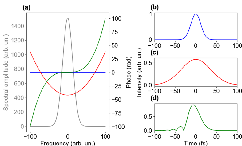
FIGURE 1.3 – (a) : spectral amplitude of the example pulse in grey with three different spectral phases : flat phase in blue, quadratic phase in red and third order phase in green. (b) : temporal envelope of the pulse with a flat phase. (c) : temporal envelope of the pulse with a quadratic phase. (d) : temporal envelope of the pulse with third order phase.
