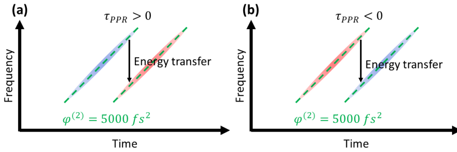
FIGURE 2.3 – Wigner-Ville representations of the probe and pump pulses. The probe pulse is represented in blue and the pump pulse in red. The slope of each pulse is equal to their respective chirp ( 5000 \text{ fs}^2 ). In figure (a) the pump-probe delay is positive resulting in an energy exchange from pump to probe whereas in figure (b) the pump-probe delay is negative resulting in an energy exchange from probe to pump.
