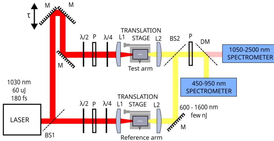
FIGURE D.4 – Experimental setup with the addition of a quarter-wave plate in each arm and a polarizer after the recombining beam splitter.
