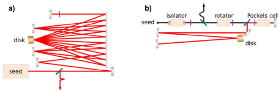
FIGURE 3.7 – Figure from [235]. Schematics of a thin-disk laser amplifier. (a) Multi-pass amplifier and (b) regenerative amplifier.
