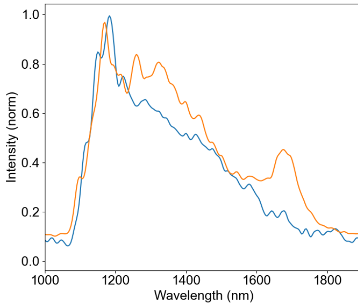
FIGURE 5.2 – Comparison of the infrared spectra of the WL generated in 6 mm-long (blue curve) and 10 mm-long (orange curve) YAG crystals. The 10 mm crystal shows a broader spectrum with a cutoff wavelength at 20% of the maximum intensity of 1720 nm compared to 1580 nm for the 6 mm-long crystal.
