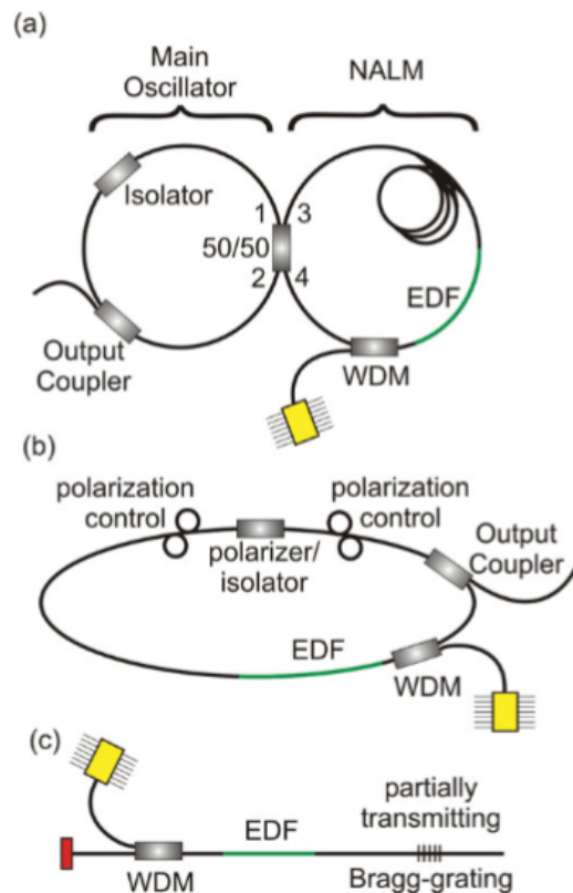
FIGURE 3.2 – Figure from [199]. Different oscillator designs. (a) figure-of-eight laser, (b) ring resonator, and (c) linear oscillator. The mode-locking mechanism in (a) and (b) is usually based on nonlinear phase shift, whereas in (c) a saturable absorber mirror is used. LD : laser diode, WDM : wavelength division multiplexer. EDF : erbium-doped fiber. SMF : standard single mode fiber
