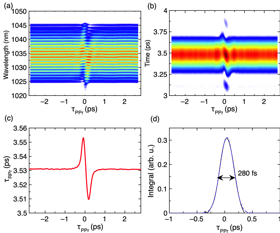
FIGURE 2.15 – Figure from [134]. Typical single-shot experimental data (LC sample). The nonlinear phase shift accumulated by the probe is estimated to be 500 mrad. (a) Interferogram of the probe and reference pulses as a function of pump-probe delay. (b) AC peak of the Fourier transform of the interferograms. (c) Relative optical group delay between reference and probe pulses ( \tau_{RPr} ) as a function of pump-probe delay ( \tau_{PPr} ). (d) Correlation profile of the pump pulse obtained from integration of the signal in (c).
