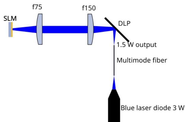
FIGURE C.2 – Beam shapin setup of the blue writing beam.
