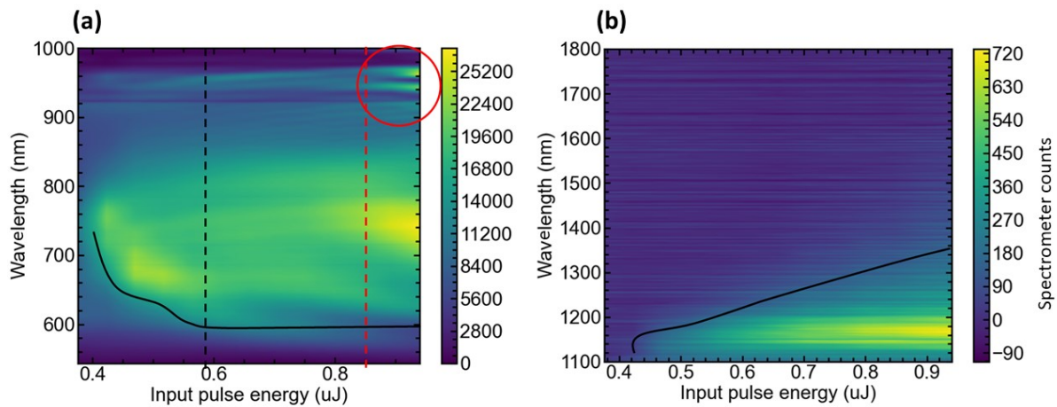
FIGURE 4.3 – (a) : Colormap of the WLG spectra as a function of pulse energy when the input interface of the YAG crystal is before the beam waist ( z = -1.5 mm) in the short-wavelength range. The color bar is in spectrometer counts. The continuous black line shows the spectral broadening by following the low wavelength edge of the continuum as a function of energy. The black vertical dotted line shows the energy at which the broadening stops. The red vertical dotted line shows the double filamentation threshold. The red circle shows the interference between the two filaments after the onset of double filamentation. (b) : Colormap of the WLG spectra as a function of pulse energy when the input interface of the YAG crystal is before the beam waist ( z = -1.5 mm) in the long-wavelength range. The color bar is in spectrometer counts. The continuous black line shows the spectral broadening by following the high wavelength edge of the continuum as a function of energy.
