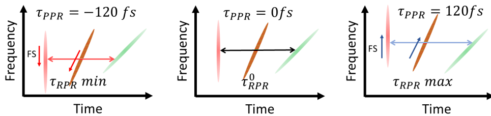
FIGURE 2.7 – Wigner–Ville distribution of the probe–reference electric fields for three different pump–probe delays \tau_{PPr} . For each sub–plot, the reference pulse is on the right (green) and the (delayed) probe pulse is on the left (red). The reference pulse is chirped and exhibits a time–dependent instantaneous frequency. The two pulses are chirped differently, and the slopes of the individual representations differ. In between the two pulses appears the interferometric component. The large arrow indicates the reference–probe group delay \tau_{RPr} . For \tau_{PPr} \leq 0 , the nonlinear phase induces a red shift of the transmitted probe (red arrow), which increases \tau_{RPr} . Symmetrically, for \tau_{PPr} \geq 0 , a blue shift decreases \tau_{RPr} . For \tau_{PPr} = 0 , there is no spectral shift and \tau_{RPr} = \tau_{RPr}^0 . FS stands for frequency shift.
