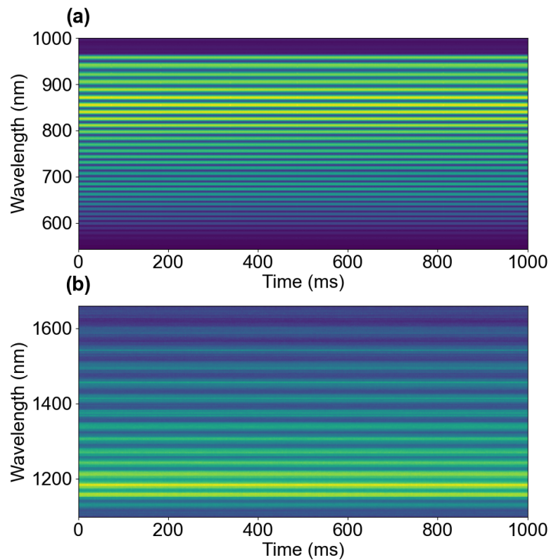
FIGURE 4.10 – Spectrograms in the short-wavelength range (a) and long-wavelength range (b) over 1000 single shot acquisitions when the WLG is optimized for the short-wavelength range.
