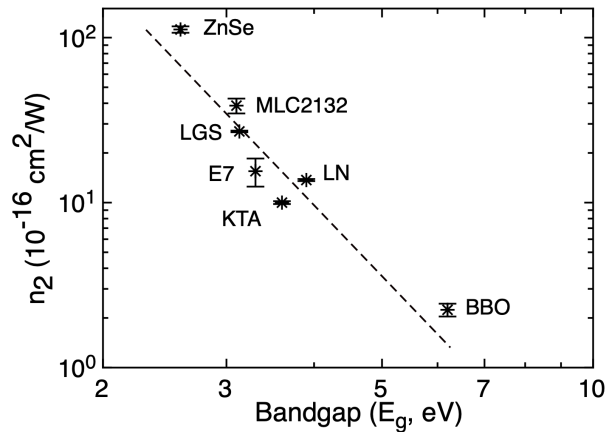
FIGURE 2.16 – Figure from [134]. Nonlinear index dependence versus bandgap for the tested samples in log-log scale. The dashed line indicates a E_g^{-4} dependence.
