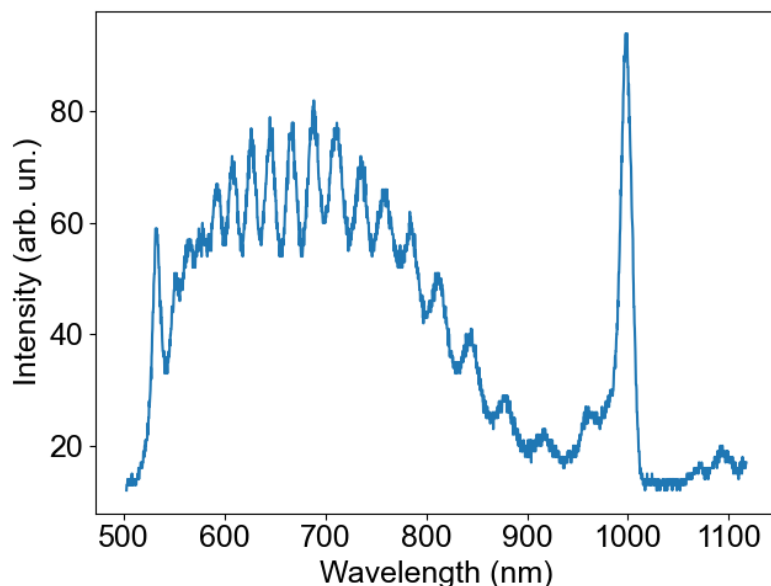
FIGURE 4.15 – Spectrum of a single WL generated with the DIRA500 pump laser.
