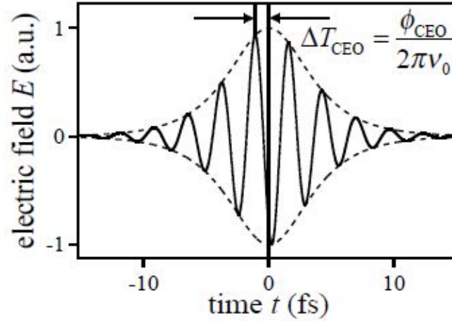
FIGURE 2 – [3] figure 1 :5-fs pulse with sech-shaped field envelope. The pulse-to-pulse carrier-envelope offset phase, \Phi_{CEO} , is proportional to the round trip delay of the central fringe, \Delta T_{CEO} , and the carrier frequency, \nu_0 . \Phi_{CEO} is defined as the phase angle at the pulse center.
