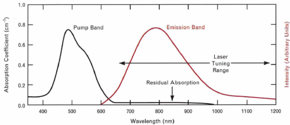
FIGURE 3.6 – Figure from [23]. Emission and absorption bands of Ti :Sa.
