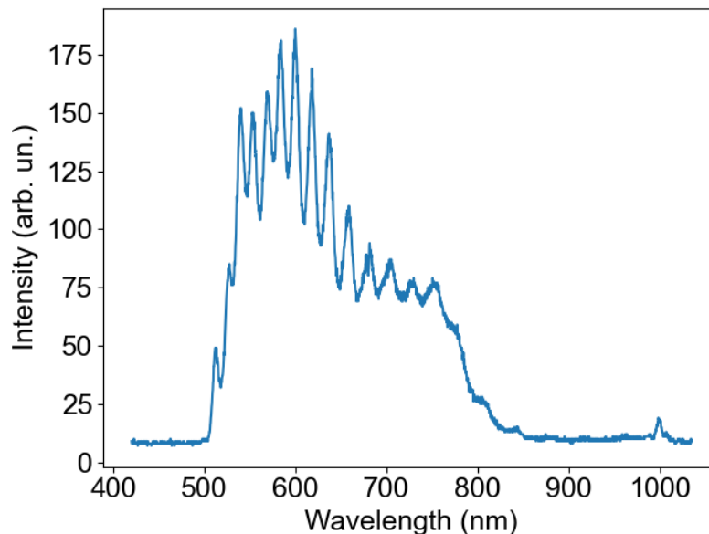
FIGURE 4.13 – Spectrum of a WL generated with the 3102 pump laser.
