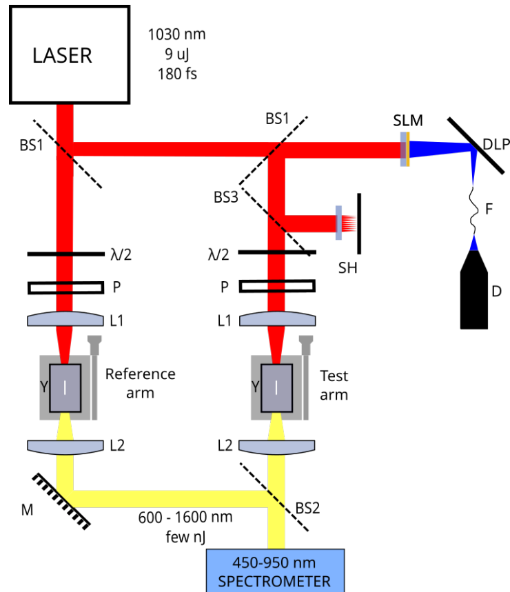
FIGURE 5.15 – Diagram of the interferometer with the addition of SLM : Spatial Light Modulator, DLP : Digital Light Processing unit, F : Square multimode optical fiber at 1030 nm, D : Blue laser diode, BS3 : 1030 nm 99/1% beam splitter, SH : Shack-Hartmann wavefront sensor.
