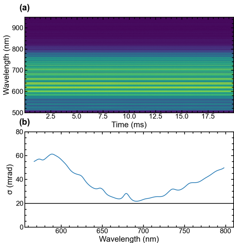
FIGURE 4.14 – Spectrogram acquired with the Amphos@3102 laser (a) and the associated phase noise (b). The black line is the reference stability of the Pharos laser at 20 mrad rms.
