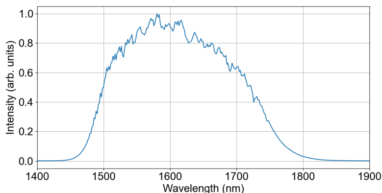
FIGURE 3.12 – Spectrum at the output of OPA 2a.
