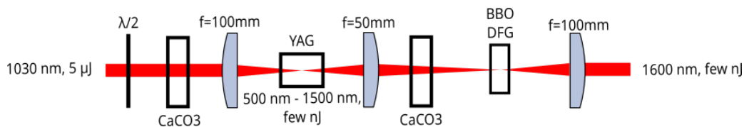
FIGURE 3.10 – Diagram of the seed generation box. \lambda/2 is a half-wave plate, \text{CaCO}_3 are calcite plates, YAG is the WLG crystal and BBO DFG is the DFG crystal.
