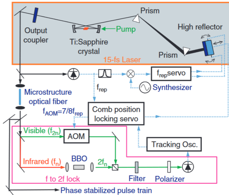
FIGURE 3.4 – Figure from [214]. Experimental setup for locking the carrier-envelope relative phase. The fs laser is located inside the shaded box. Solid lines are optical paths and dashed lines are electrical paths. The high reflector mirror is mounted on a transducer to provide both tilt and translation. AOM—acoustic-optic modulator; APD—avalanche photodiode; BBO— \beta -barium-borate doubling crystal.
