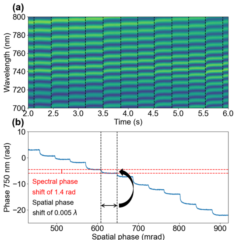
FIGURE 5.24 – a : Spectrogram around 750 \text{ nm} in the case of aberration (ii). The vertical dashed black lines represent an increment in the spatial phase (see text). b : Extracted phase at 750 \text{ nm} from figure (a).
