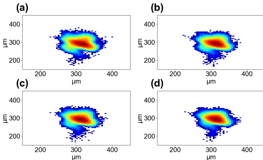
FIGURE 5.23 – Far field profile of the beam in the test arm at the minimum (a), maximum (b) and center (c) and (d) of the measurement range with respective PtV phases of 0.056 , 0.17 , 0.113 and 0.119 \lambda in logarithmic scale for aberration (ii).
