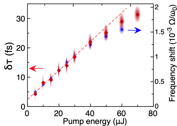
FIGURE 2.13 – Figure from [133]. \delta\tau (red) and normalized frequency shift ( \Omega/\omega_0 , blue) as a function of the pump energy for the chirp values indicated by the gray lines in figures 2.11 and 2.12.
