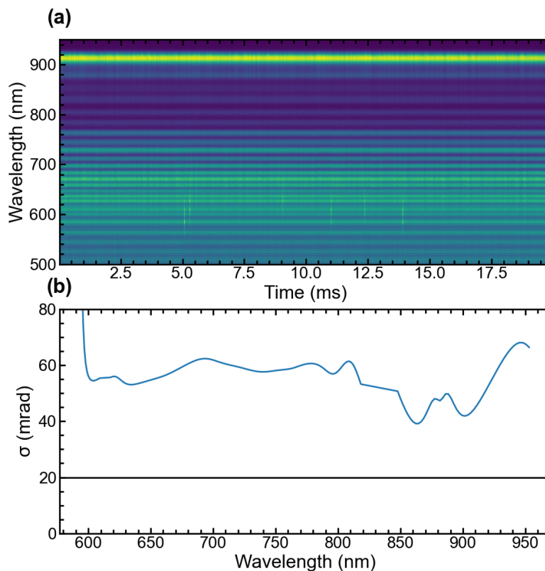
FIGURE 4.16 – Spectrogram acquired with the DIRA500 laser (a) and the associated phase noise (b). The black line is the reference stability of the Pharos-driven WL at 20 mrad rms.
