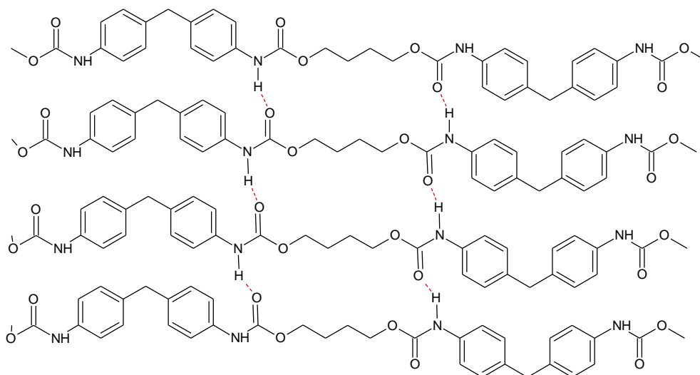
Figure 1.8: Schematic representation of the hydrogen bonding between hard segments composed of 4,4'-diphenylmethane diisocyanate and 1,4-butanediol
