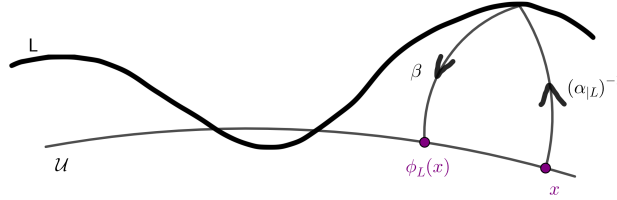
Figure 2.2: The diffeomorphism \varphi_L induced by a bi-section L of \mathcal{W}
