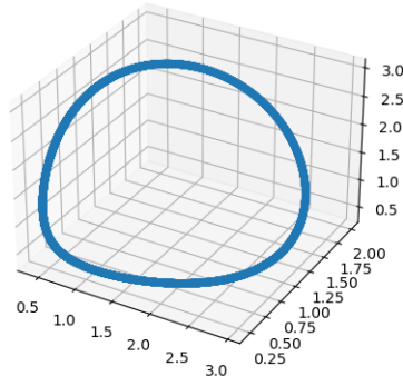
Figure 1.2: Hamiltonian Poisson method at order 1 for equation (1.2)
