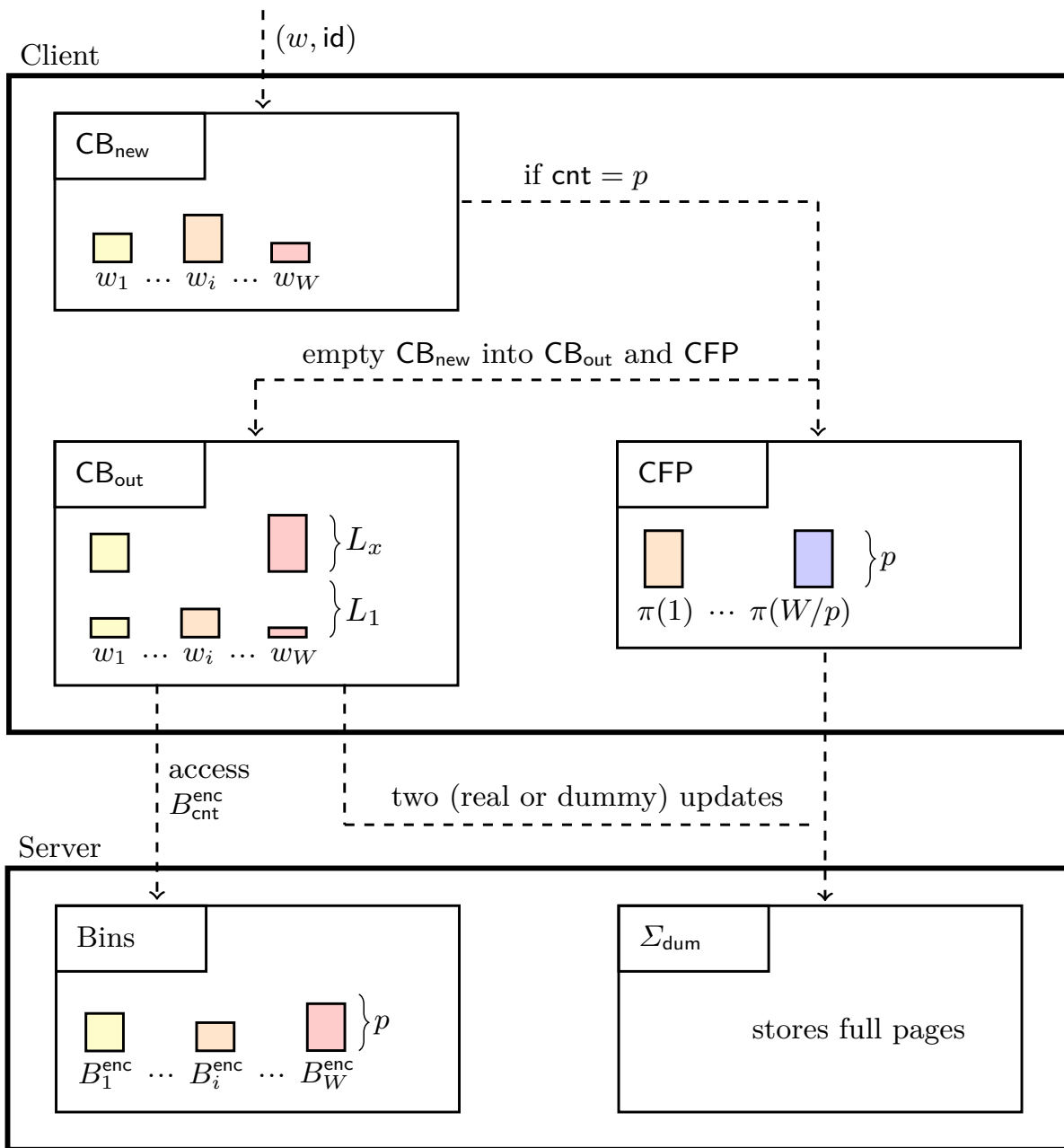
Figure 6.1: Sketch of the update schedule of BigHermes 1 . (The data structure T_{len} are omitted for clarity.) Each update, the variable cnt is incremented and the dotted lines are executed. See Algorithm 10 for pseudo-code.
