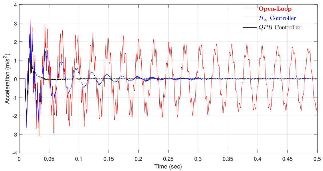
Figure 6.9. Impulse response to a perturbation w = 1 \text{ m/sec}^2 to the flexible beam's synthesis model. The open-loop (red), the \mathcal{H}_\infty LMI-based controller (blue) and the QPB controller (black).
