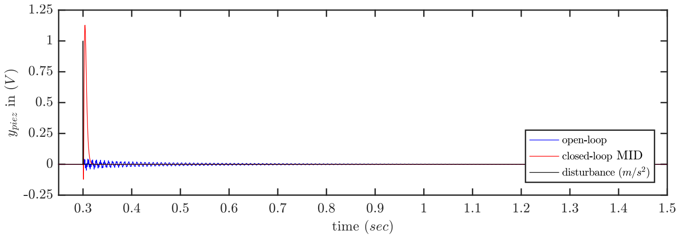
Figure 5.6. Time response of the measured output y_{piez}(t) .
