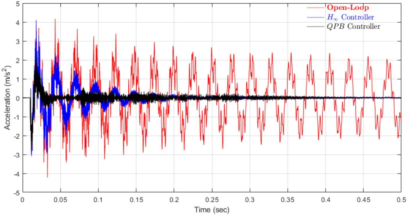
Figure 6.10. Impulse response to a perturbation w = 1 \text{ m/sec}^2 to the flexible beam's analysis model. The open-loop (red), the \mathcal{H}_\infty LMI-based controller (blue) and the QPB controller (black).
