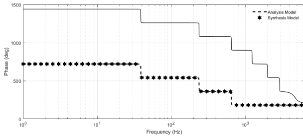
(a) Bode diagram from w to z_a .
