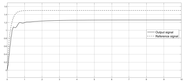
(b) Output response for the PMD-controller.
