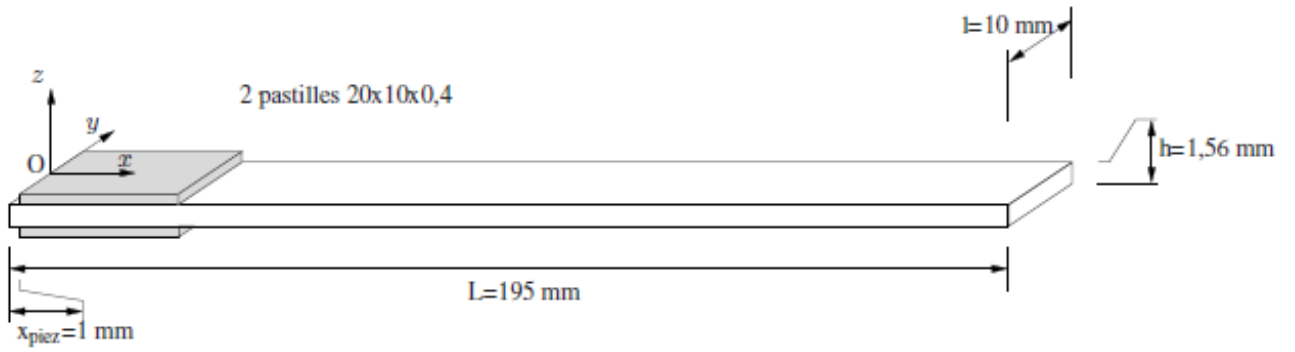
Figure 3.4. Flexible beam.
