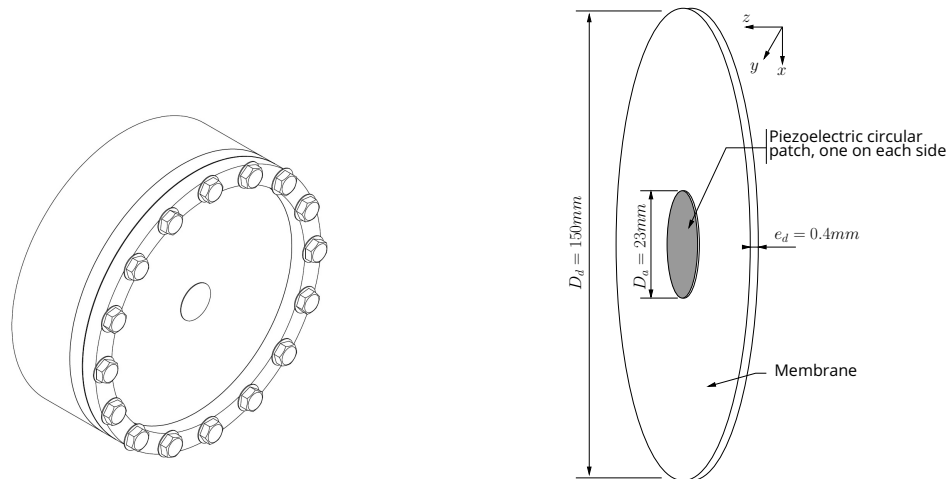
Figure 3.10. Flexible axisymmetric membrane (dimensions on the right) inserted in the device which is subjected to vibrations (Computer Aided Design figure on the left)
