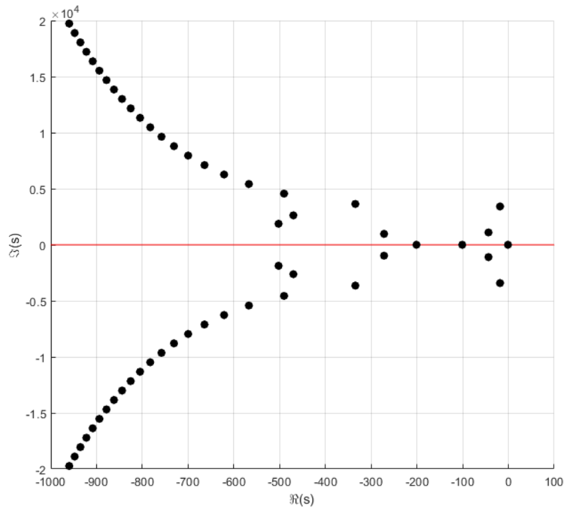
Figure 5.3. Three coexisting real roots of the flexible beam's infinite-dimensional characteristic quasipolynomial in closed-loop with the QPB controller. The parameters' values chosen are p_0 \approx 3.14258 , p_{r0} \approx 1.07203 \times 10^{-1} , q_0 \approx 33.6443 , q_{r0} \approx 1.68338 and \tau \approx 7.47849 \times 10^{-3} sec.
