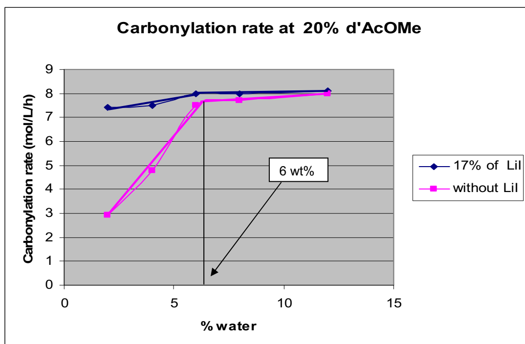
Figure 1 : Carbonylation rate at 20% methylacetate remaining
