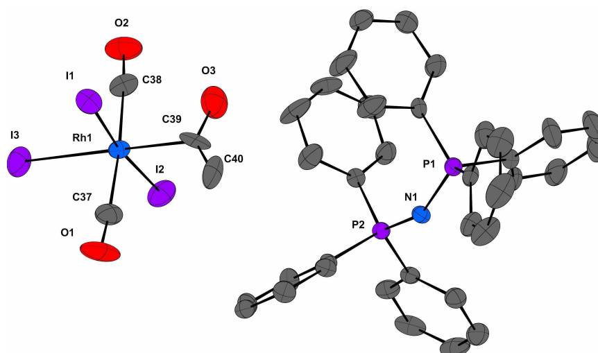
Scheme 13 : X-ray structure of [PPN][Rh 3 (COMe)(CO) 2 ] 4 .
