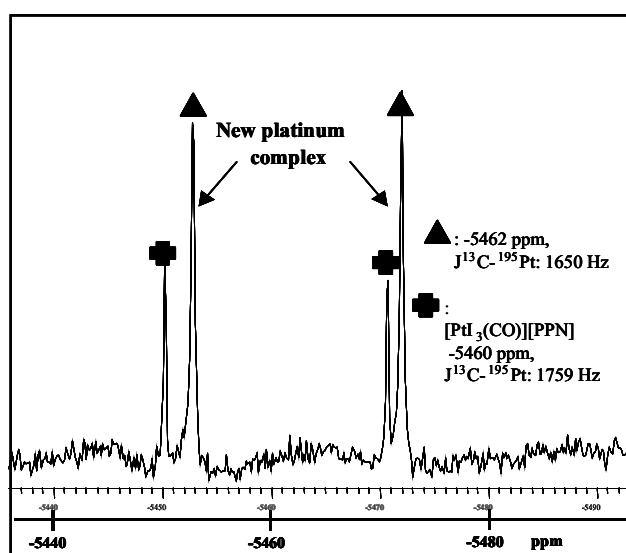
Figure 26 : ^{195}\text{Pt} NMR spectra at -30^\circ\text{C} on the products from the reaction of [\text{PPN}][\text{Ir}_3(\text{CH}_3)(^{13}\text{CO})_2] 6 with 0.3 eq of [\text{PtI}_2(\text{CO})]_2 .
