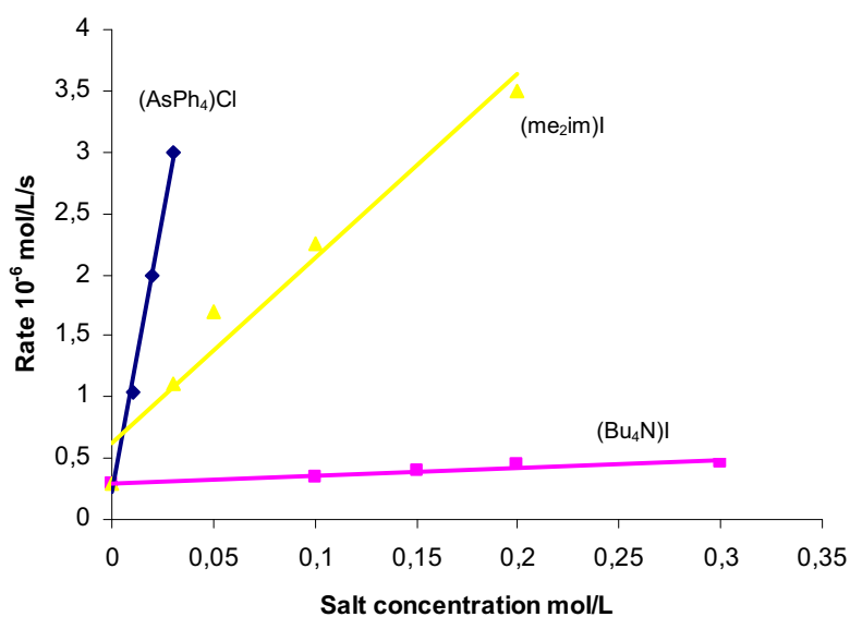
Figure 2 : Variation of rates of oxidative addition of \text{CH}_3\text{I} to [\text{AsPh}_4][\text{RhI}_2(\text{CO})_2] ( 5 \cdot 10^{-3} mol. L -1 ) in dichloromethane in the presence of various salts.
