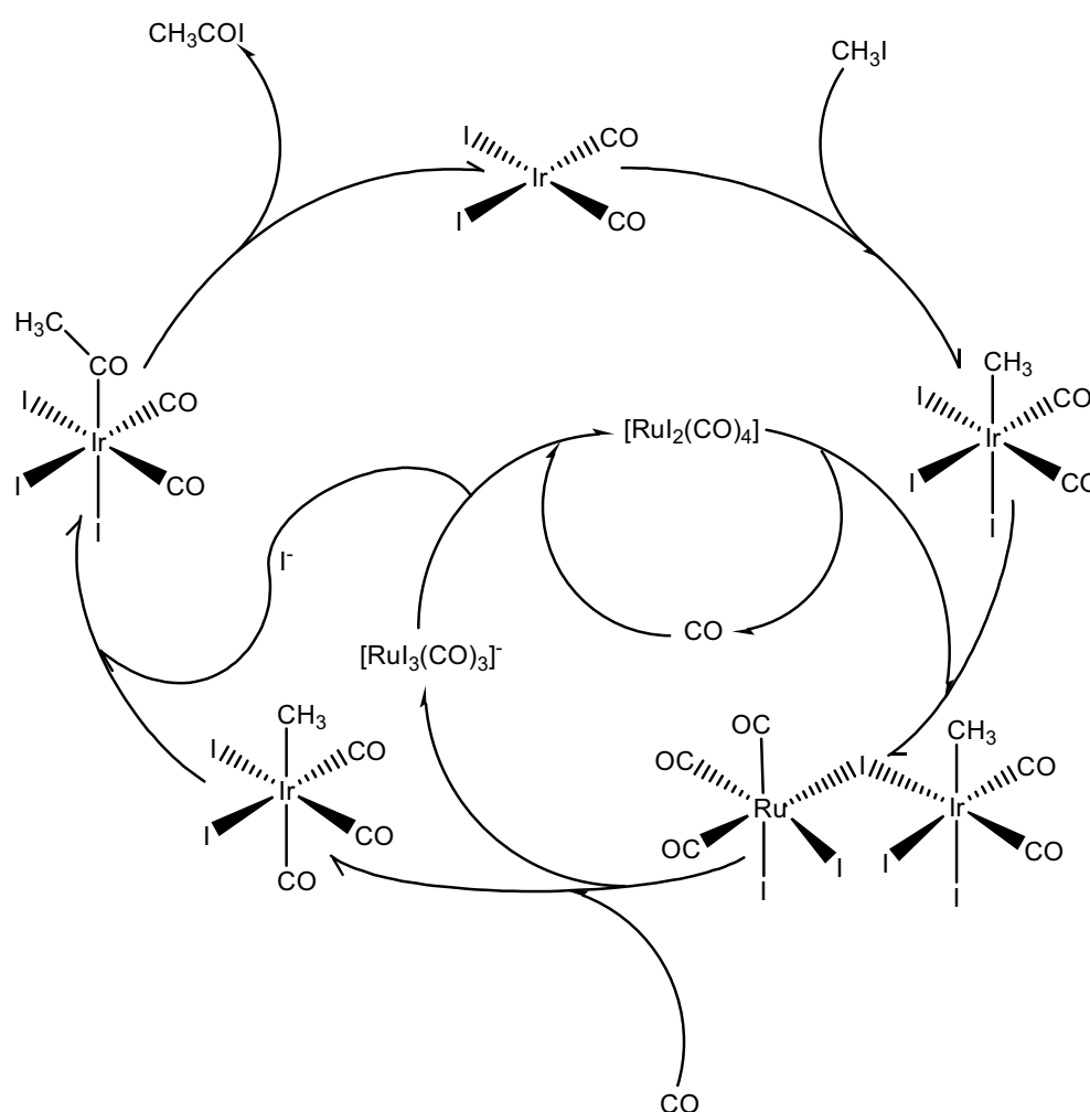
Scheme 6 : Proposed reaction mechanism for the Cativa process.
