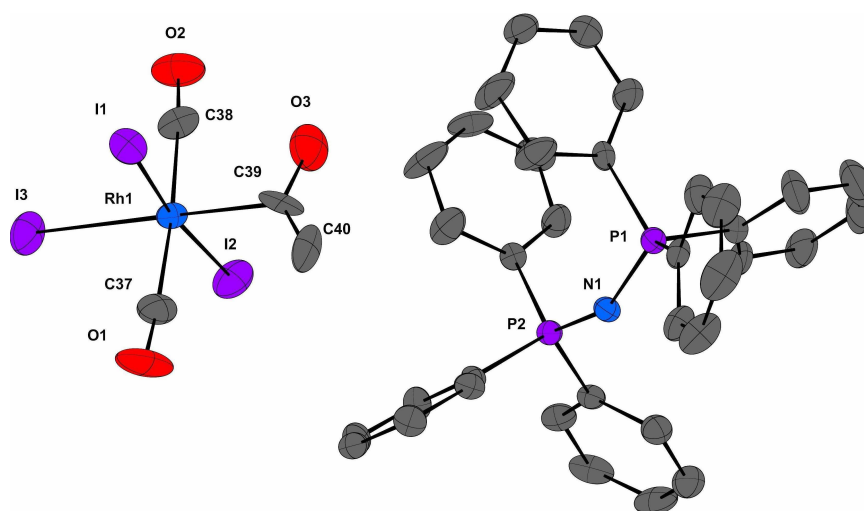
Scheme 13 : X-ray structure of [PPN][Rh 3 (COMe)(CO) 2 ] 4 .
