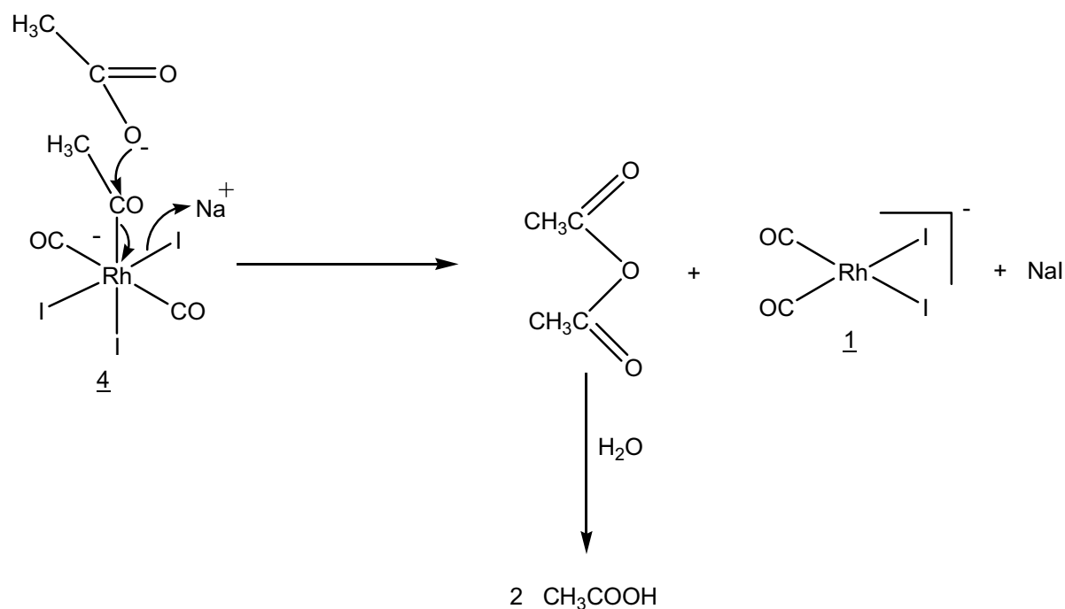
Scheme 8 : Proposed mechanistic pathway for the reaction between complex 4 and the acetate anions.
