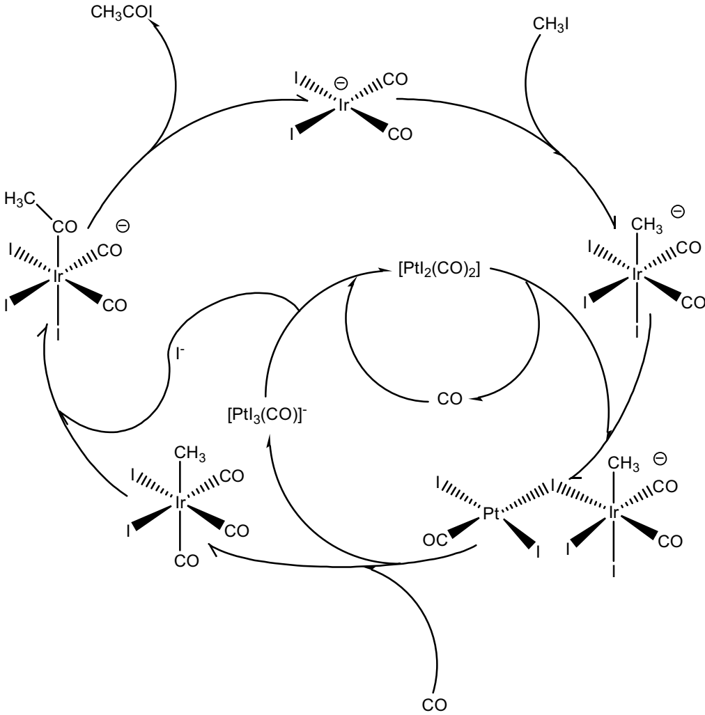
Scheme 8 : Proposed catalytic cycle for the iridium/platinum system.
