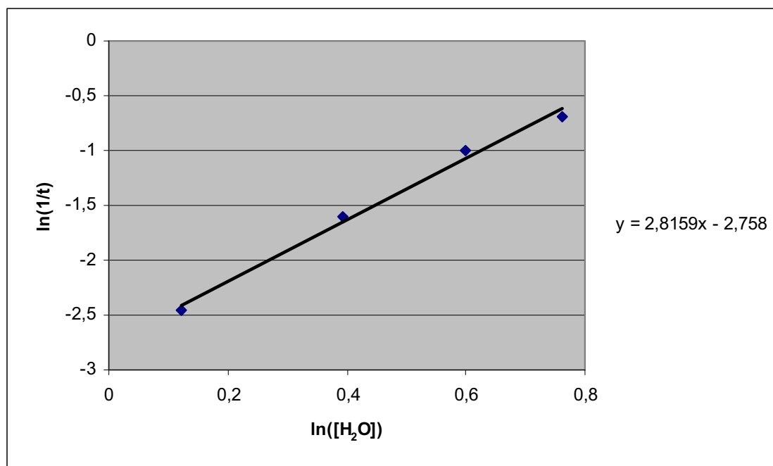
Figure 29 : Plot of \ln(1/t) as function of \ln([H_2O]) .
