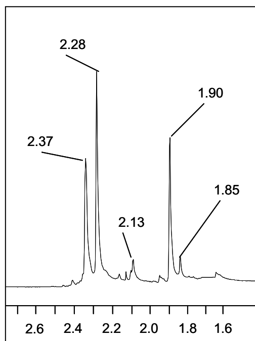
Figure 27 : ^1\text{H} NMR spectra at -30^\circ\text{C} on the products from the reaction between [\text{PPN}][\text{Ir}_3(\text{CH}_3)(^{13}\text{CO})_2] 6 and 0.3 eq of [\text{PtI}_2(\text{CO})]_2 .
