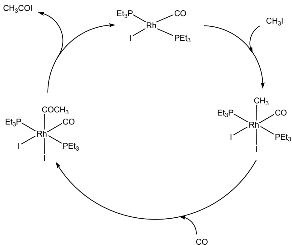
Scheme 14 : Catalytic cycle of the methanol carbonylation catalyzed by the neutral complex [\text{RhI}(\text{PEt}_3)_2(\text{CO})]
