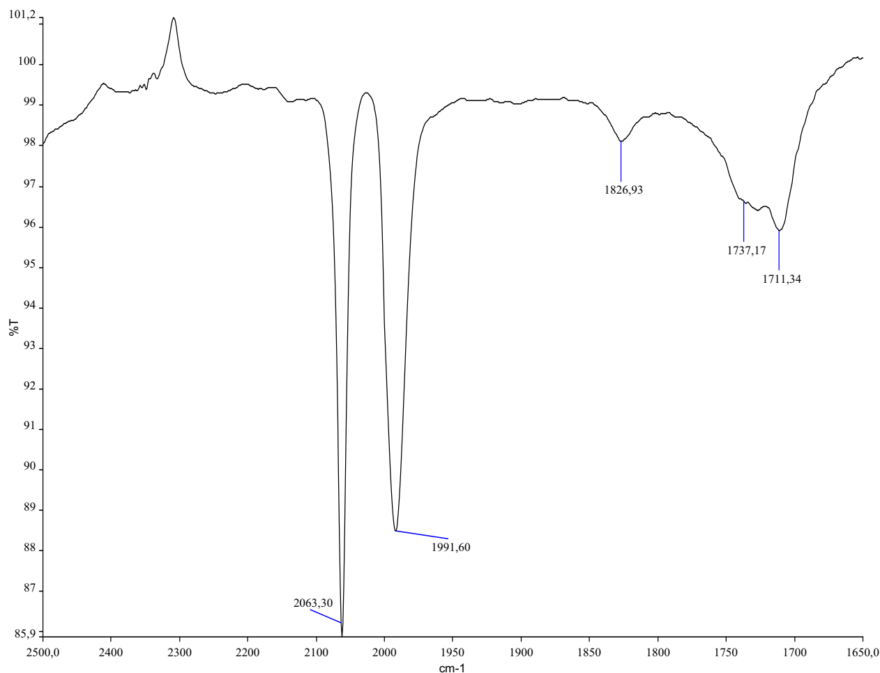
Figure 15 : IR spectrum of the reaction between complex 4 and sodium acetate ions in methanol/CH 2 Cl 2 mixture
