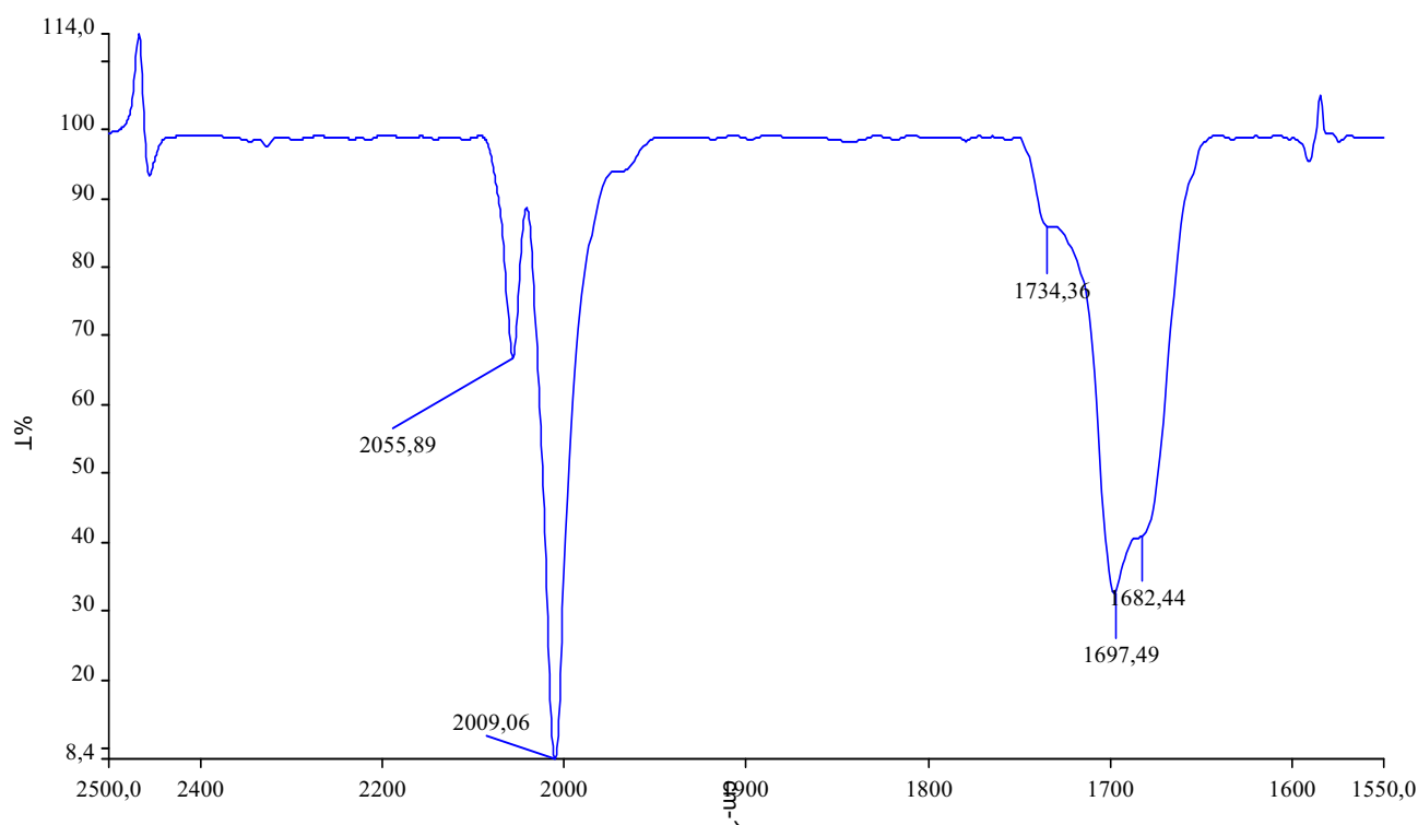
Figure 5 : IR spectrum of [\text{Rh}_3(^{13}\text{COCH}_3)(^{13}\text{CO})]_2^- 3 in \text{CD}_2\text{Cl}_2 , r.t.
