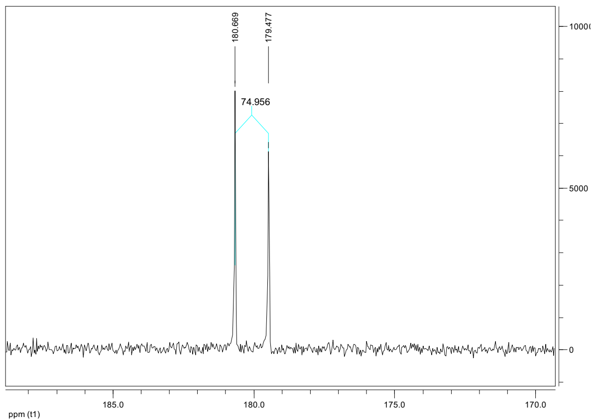
Figure 31 : ^{13}\text{C} NMR spectrum of [\text{Rh}(\text{}^{13}\text{CO})_2]_2 in \text{CD}_2\text{Cl}_2 , r.t.
