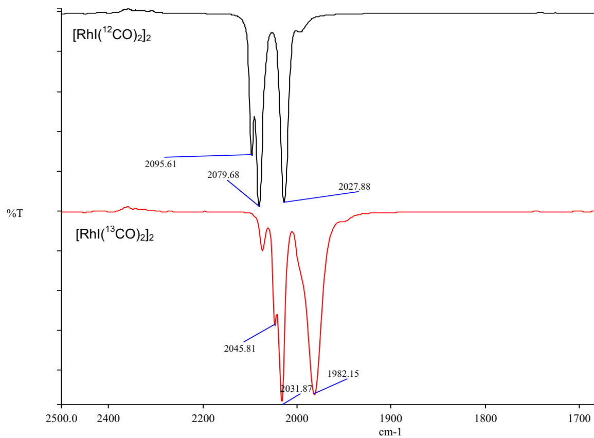
Figure 30 : Infrared spectra of [\text{Rh}(\text{CO})_2]_2 and [\text{Rh}(\text{}^{13}\text{CO})_2]_2 in \text{CH}_2\text{Cl}_2 .
