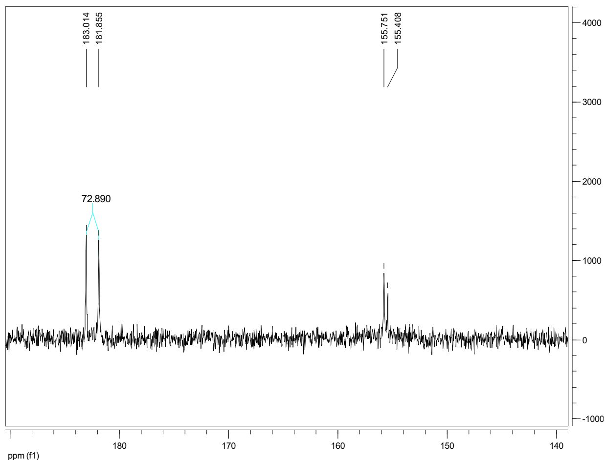
Figure 32 : ^{13}\text{C} NMR spectrum of the products from the reaction between [\text{Rh}(\text{}^{13}\text{CO})_2]_2 10 and [\text{PPN}][\text{Ir}_3(\text{CH}_3)(\text{}^{13}\text{CO})_2] 6 Rh/Ir = 1/1 in \text{CD}_2\text{Cl}_2 , r.t.
