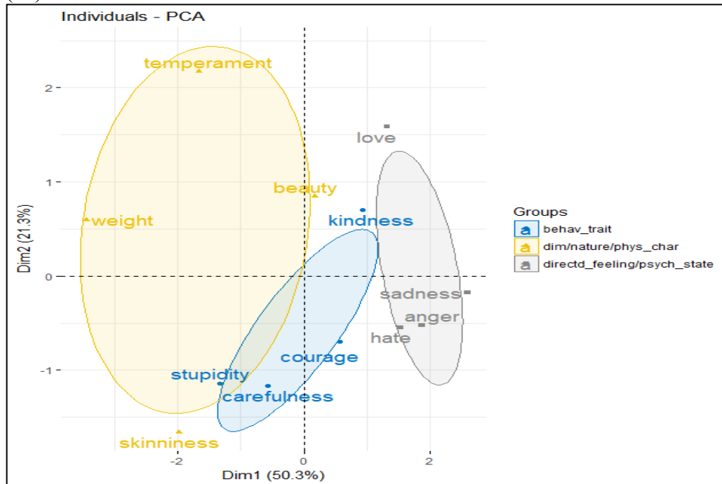
Figure 4. Graph of 12 English HPNs, based on a principal component analysis, with 95% confidence ellipses for mean values of groups
