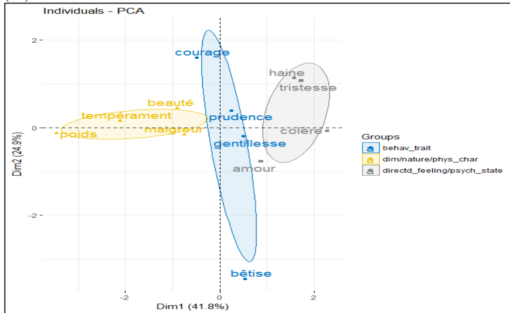
Figure 2. Graph of 12 French HPNs, based on a principal component analysis, with 95% confidence ellipses for mean values of groups
