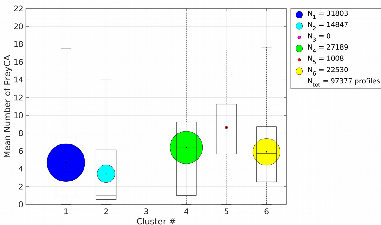
Figure II.9: Number of SES prey capture attempts per grid point for each bioregion. Each black box represents the distribution of the SES data for the corresponding bioregion. The horizontal black line inside each box represents the median. The top and bottom limits of each box are the 25 th and 75 th percentiles, respectively. The vertical dashed black lines extending above and below each box represent the full range of non-outlier observations. Black dots in the center of colored circles represent the mean. The color of each circle refers to the colors used in Figure II.1. The size of colored circles is proportional to the number of data points (SES profiles). The number of data points used to compute the distribution of the data in each cluster is indicated in the top-right inset. N_i is the number of data points available in cluster i ( i = 1, 2, \dots, 6 ). N_{tot} is the total number of SES profiles used to compute number of SES prey capture attempts (PCA) per grid point.
