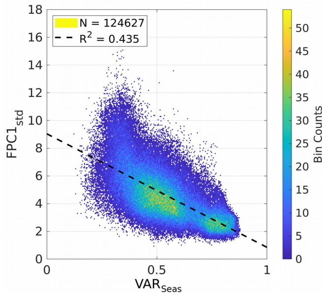
Figure I.15: Scatter plot of FPC1_{STD} versus climatological mean VAR_{Seas}
