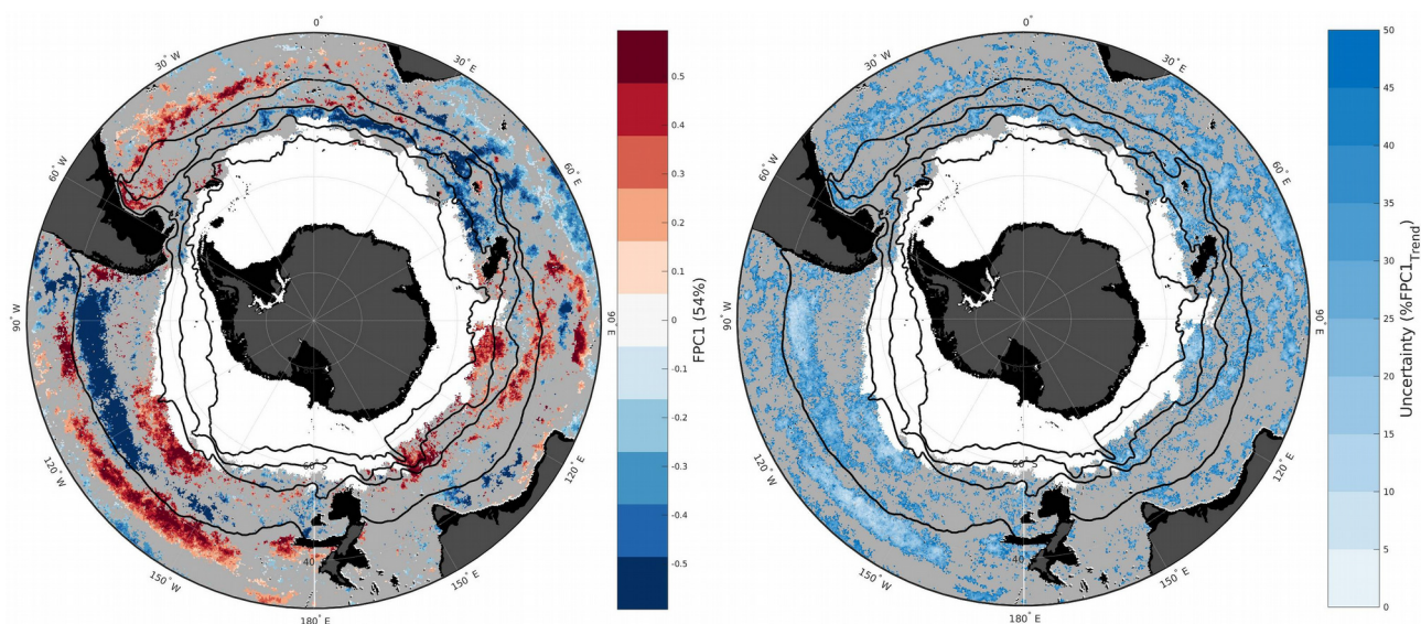
Figure I.6. Spatial distribution of (left panel) FPC1 trend estimates and (right panel) their uncertainties (width of 95% confidence interval) for the 1998-2022 GlobColour CHL record. Light gray regions indicate that the trend is not statistically different from zero. Black lines represent the major fronts of the SO defined in Section I.2.c (from north to south): Subtropical Front (STF), Subantarctic Front (SAF), Polar Front (PF) and Southern ACC Front (SACCF). The areas filled with gray color are land areas. The areas filled with black color depict marine areas with bathymetry shallower than -1000 meters. Pixels with less than 50% valid CHL values in the 1998-2022 time series (see Section I.2.d) are represented in white (white area around Antarctica, south of \sim 60^{\circ}\text{S} ).
