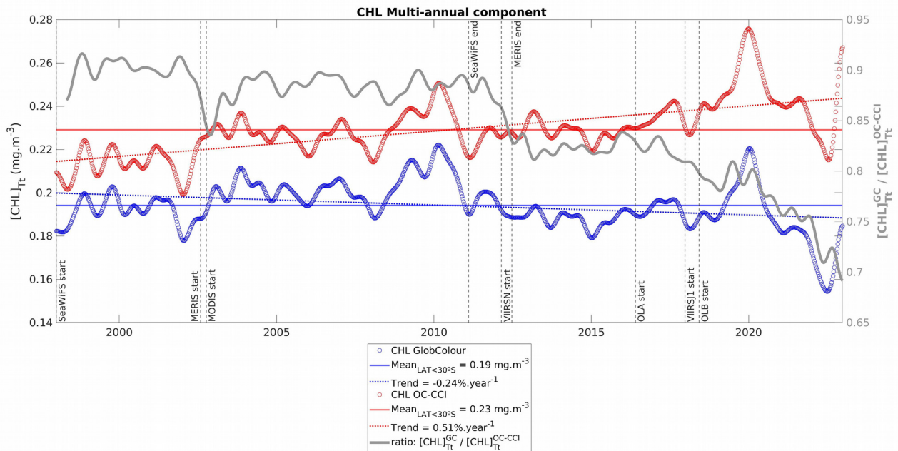
Figure I.1. Assessment of long term changes in CHL biomass. Comparison of the multi-annual component (see details in Section I.3.a) of two analogous ocean-colour CHL products, namely the products distributed by Copernicus Marine Service GlobColour (blue circles) and the European Space Agency Ocean Color Climate Change Initiative (OC-CCI, red circles) (see details in Section I.2.d). Continuous lines show climatological 1998-2022 value and dashed lines show long-term trends, with same color code as circles. Continuous gray line shows the ratio between CHL from GlobColour and CHL from OC-CCI. At each date, the data displayed in Figure I.1 corresponds to the mean value computed for the study zone (Southern Ocean, south of 30°S). Trends in CHL biomass are estimated as differences in CHL per year and were only displayed for qualitative appreciation of diverging trends (no absolute values of trends were provided).
