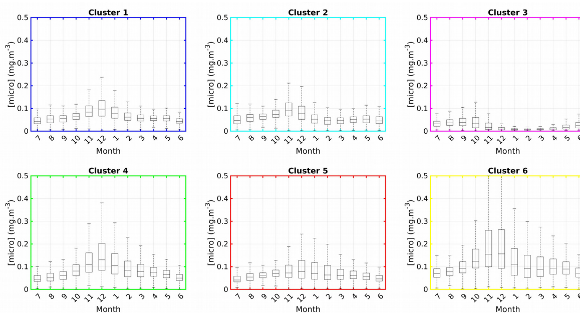
Figure II.18: Concentration of microphytoplankton per bioregion and per month. Cluster number (bioregion) is displayed above each panel and the color of each panel refers to the colors used in Figure II.1. Concentration of microphytoplankton ([micro]) is given in \text{mg.m}^{-3} . Months in the abscissa are displayed with annual cycle centered on Austral summer (i.e. month of December, number 12). Each black box represents the distribution of the PSC data for the corresponding month of the year. The horizontal black line inside each box represents the median. The top and bottom limits of each box are the 25 th and 75 th percentiles, respectively. The vertical dashed black lines extending above and below each box represent the full range of non-outlier observations.
