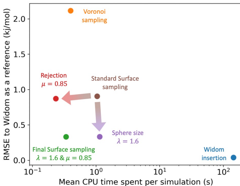
Figure 3.13 – Comparison of the RMSE to the reference Widom insertion and the average computation time for different types of enthalpy calculation methods. The surface sampling calculation was all done with 2k sampling points on each sphere and the Widom simulations were done using 12k cycles. These values correspond to the value at the convergence identified using Figure 3.8.
