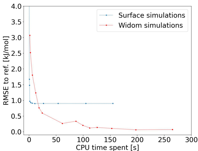
Figure 3.8 – Convergence plot of the RMSE on the adsorption enthalpy for the RAESS algorithm (blue) compared to a 100k-step Widom insertion simulation (red) for xenon adsorption in all structures of the CoRE MOF 2019 database.
