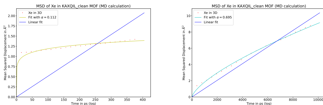
Figure 5.6 – Plots of the MSD at the last two timescales considered in Figure 5.5. On the left, the timescale between 0.01 ns and 0.4 ns is considered. The MSD is fitted using a power function with the same previously determined exponent, and a linear fit is provided to demonstrate its incompatibility with the diffusion equation. On the right, a similar approach is employed for the timescale between 0.4 ns and 9 ns.
