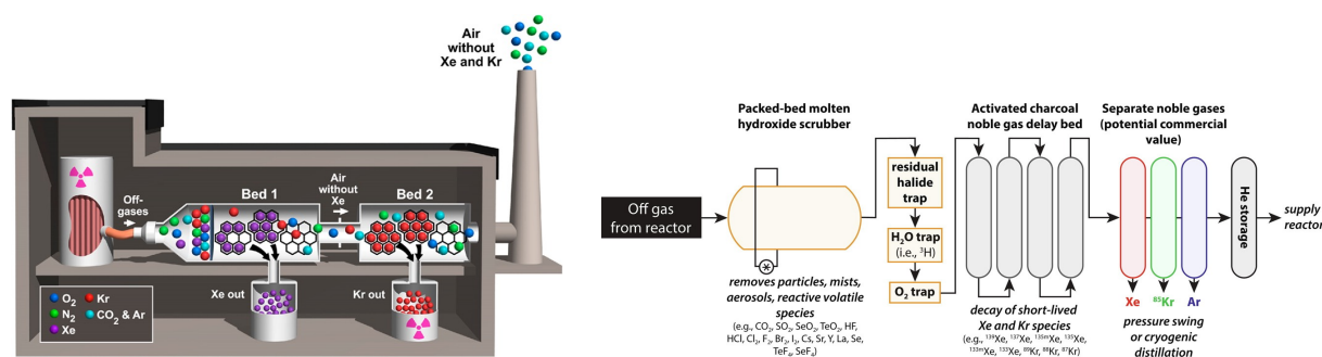
Figure 1.10 – Representation of xenon/krypton separation process using porous materials in a nuclear fuel reprocessing plant (left panel) and in a molten salt reactor (right panel). Reprinted with permission from Ref. [2] copyright © 2014 American Chemical Society and Ref. [175] copyright © 2019 Elsevier.
