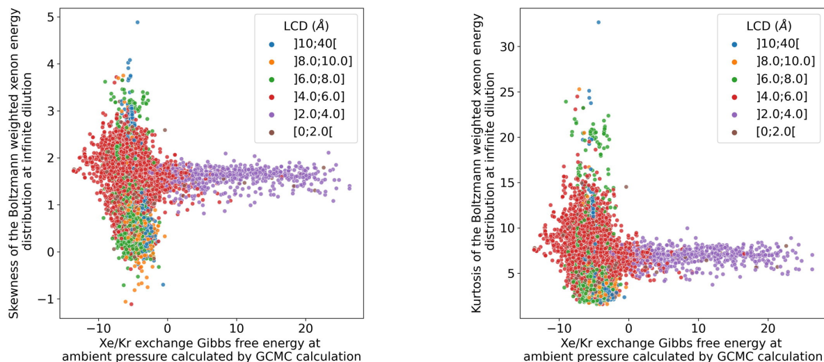
Figure 3.35 – Comparison of the ambient-pressure Xe/Kr exchange Gibbs free energy calculated by GCMC simulations of RASPA2 with 100,000 cycles and the skewness (left) and the kurtosis (right) of the Boltzmann weighted energy distribution of xenon calculated by the GrAED algorithm at 298 K.
