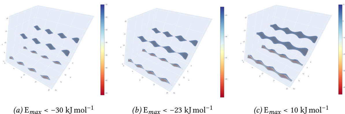
Figure 5.22 – 3D visualization of channels within KAXQIL using different energy thresholds E_{\text{max}} . Depending on the maximum value of energy allowed, the channel is either composed of unconnected basins (a), or they are fully connected (b) and (c). This illustrates the principle of the energy barrier detection.
