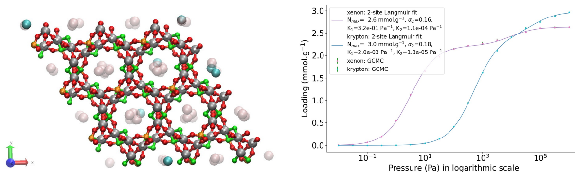
Figure 2.32 – MISQIQ: Representation of a chiral open-framework fluoro-aluminophosphate [C_4N_3H_{16}].[Al_6P_3O_{12}F_6(OH)_6] also denoted ALPO-JU89, which has been loaded with xenon and krypton in a GCMC simulation, on the left side. 216 Color code: Al in silver, P in orange, O in red, H in white and F in green for the framework; Xe in transparent pink and Kr in cyan for the adsorbates. The pure-component isotherms fitted with a 2-site Langmuir model (equation 2.34) for both xenon and krypton at 298 K on the right side.
