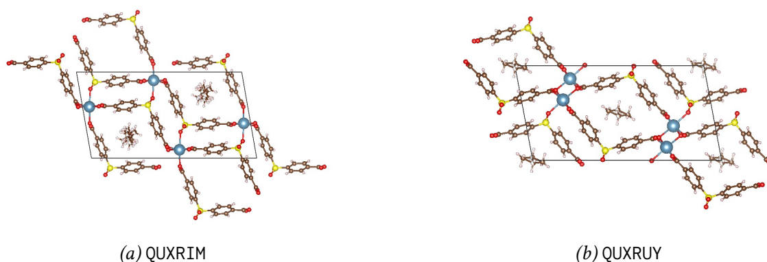
Figure 6.3 – An illustration of the effect of the orientation of hexane inside a SBMOF-1-like material. In QUXRIM (a), the carbon atoms are oriented towards the S atoms, whereas in QUXRUY (b) they are oriented towards the Ca atoms. This difference in the orientation could explain the different structural properties of the materials reported in Table 6.2. Color code: brown for C, white for H, red for O, cyan for Ca, yellow for S. The structure visualizations are generated using the VESTA software. 55
