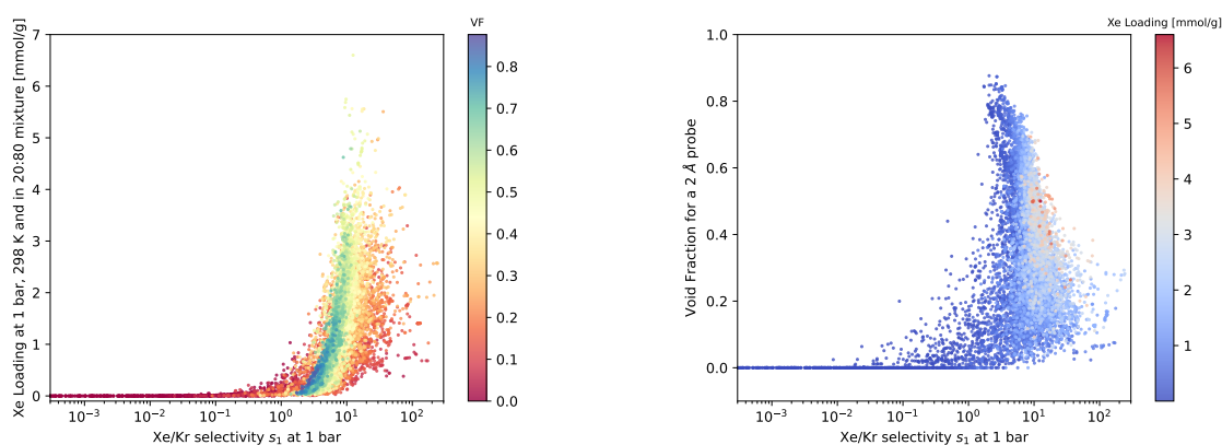
Figure 2.7 – On the left: scatterplot of the xenon uptake as a function of the selectivity and labeled by the values of the void fraction. On the right: scatterplot of the selectivity and the void fraction labeled by the quantity of xenon adsorbed. The selectivity and uptake are calculated by a GCMC simulation of a 20:80 Xe/Kr mixture.
