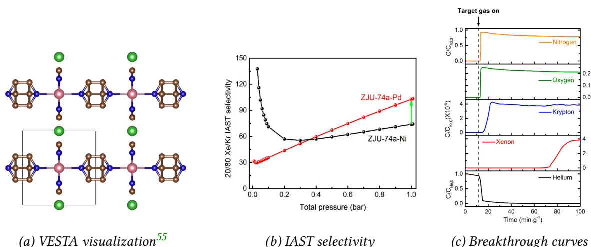
Figure 6.7 – (a) Representation of the ZJU-74a-Ni structure with the color code: brown for C, white for H, red for O, pink for Co, green for Ni. We can see the open metal sites or coordinatively unsaturated nickel metals that could interact with an adsorbate in the center of the pore. (b) Selectivity values at different pressure conditions for a 20:80 Xe/Kr binary mixture calculated by the IAST theory. (c) Experimental breakthrough curves of a gas mixture with 400 ppm Xe and 40 ppm Kr balanced with dry air in ZJU-74a-Pd. Reprinted with permission from Ref. [8] copyright © 2022 American Chemical Society.
