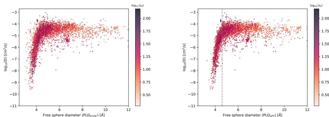
Figure 5.8 – Xenon diffusion coefficient at infinite dilution as a function of the pore limiting diameter (PLD). The diameter of the largest free sphere is defined using two different radius systems: the standard CCDC-based PLD (on the left), and the one defined using the UFF forcefield (on the right) 51 – as defined in Chapter 2.
