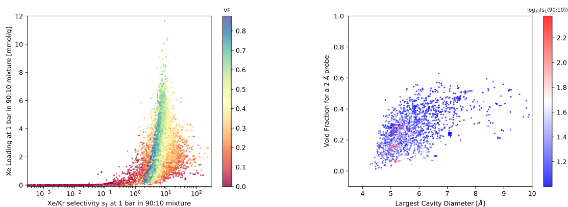
Figure 2.11 – Illustration of the effect of the composition by representing the same figures as in 2.7 and 2.9 but for a 90:10 composition. On the left: scatterplot of the xenon uptake as a function of the selectivity ( s_1(90 : 10) ) and labeled by the values of the void fraction. On the right: scatterplots of the void fraction as a function of the LCD_{UFF} and labeled by the selectivity ( s_1(90 : 10) ) values superior to 10 in log-scale.
