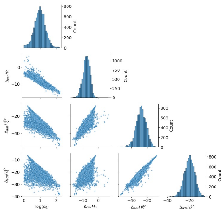
Figure 2.13 – For 8 401 MOFs with favorable thermodynamic Xe/Kr selectivity ( s_0 > 1 ), pair plots of \log(s_0) , \Delta_{\text{exc}}H_0 , \Delta_{\text{ads}}H_0^{\text{Xe}} and \Delta_{\text{ads}}H_0^{\text{Kr}} (the enthalpies are in \text{kJ mol}^{-1} ) in the off-diagonal subplots and the distribution of each quantity is on the diagonal.
