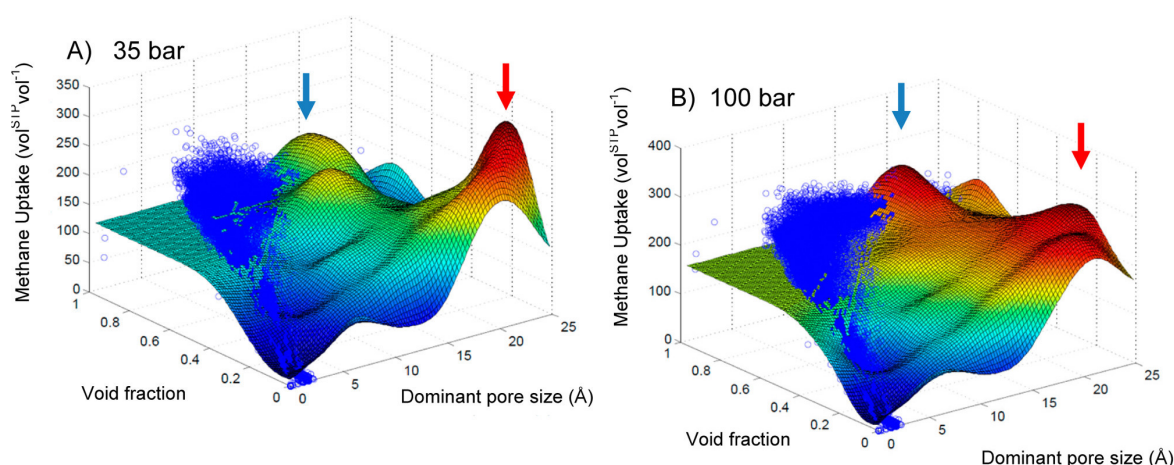
Figure 1.8 – Two-dimensional response surfaces of the support vector machine (SVM) models trained by Fernandez et al. for methane storage at (A) 35 bar and (B) 100 bar using void fraction and dominant pore size. The blue dots represent the GCMC simulated uptake values. The color of the surface represents the methane storage value, from blue (the lowest values) to red (the highest values). Blue and red arrows indicate maxima on the response surface. Reprinted with permission from Ref. [17]. Copyright © 2013 American Chemical Society.
