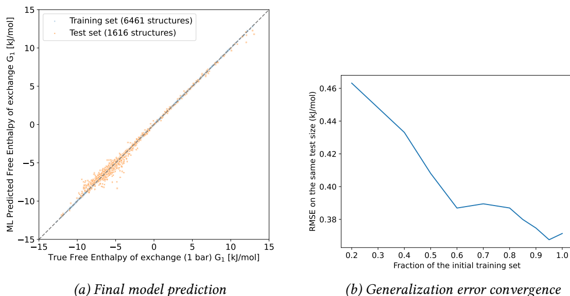
Figure 4.8 – (a) Scatterplot of the exchange free energy predicted by the model. There is a good agreement between the predicted and true values. On the test set, there is an RMSE of 0.37 \text{ kJ mol}^{-1} and an MAE of 0.21 \text{ kJ mol}^{-1} . This plot is equivalent to the scatterplot between the logarithm of the ambient-pressure selectivity (Figure 4.9). (b) Root mean squared errors on the same test set (20% of all data) as a function of the fraction of the training set used to train smaller models. The error decreases as the amount of data increases.
