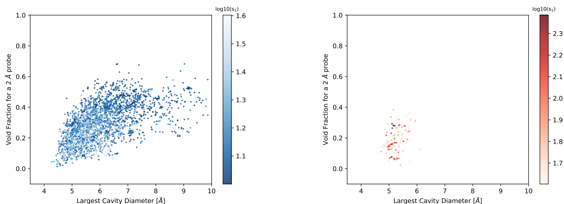
Figure 2.9 – Scatterplots of the void fraction as a function of the LCD_{UFF} and labeled by the \log_{10} of the selectivity values. On the left, only the materials with a selectivity between 10 and 40 are considered; and on the right, selectivity values over 40.
