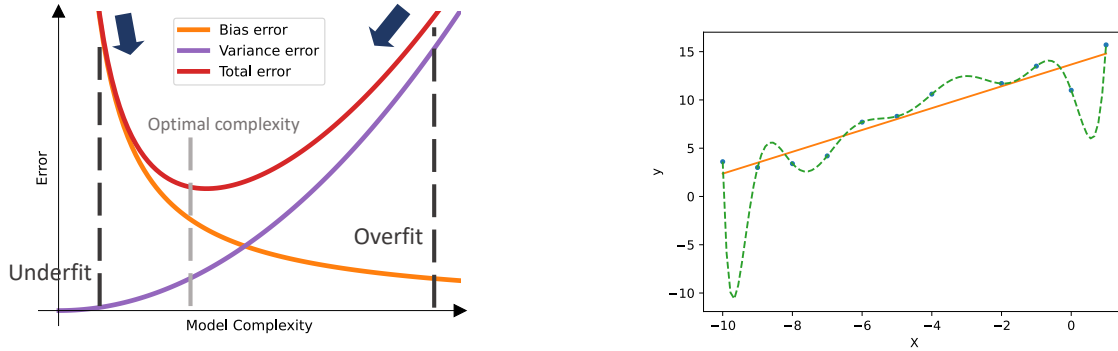
Figure 4.3 – On the left, theoretical relation between the bias, variance and total errors and the model complexity. The overfit case is illustrated on the right plot when considering polynomial fits. The lower degree linear function is more generalizable than the biased high degree polynomial that fits perfectly the data.
