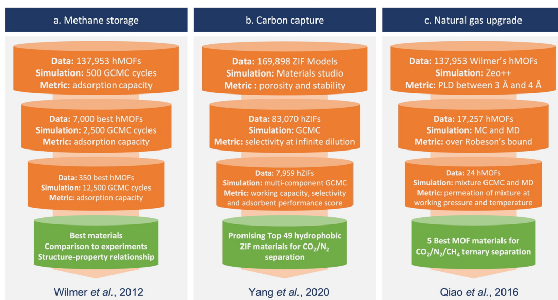
Figure 1.3 – Simplified representation of typical funnel-type screening procedures, exemplified on three different applications from the published literature. (a) Wilmer et al. 12 used a series of bi-component Grand Canonical Monte Carlo (GCMC) calculations at different levels of complexity to screen a large dataset of hypothetical MOFs for methane storage application. (b) Yang et al. 16 used simulations at infinite dilution to prescreen the dataset before using computationally demanding simulations and multiple metrics to find the most promising ZIFs for carbon capture. (c) In Qiao et al., 15 transport properties were screened along standard adsorption properties to find the best materials for the targeted CO 2 /N 2 /CH 4 ternary separation; similarly, cheaper calculations at infinite dilution were carried out in a first step, before using more expensive calculations at working pressure and temperature.
