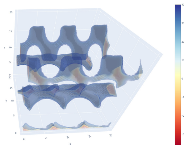
Figure 5.17 – Snapshot of a 3D visualization of the xenon interaction energy inside the channels of the OQESAF 288 material. Two distinct unidimensional channels can be observed in the visualization. In an MD simulation of a single xenon per box, in this study, all possible initial positions were not tested out.
