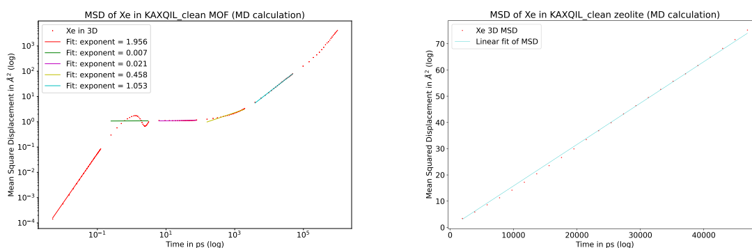
Figure 5.7 – On the left panel, the MSD in log-log scale and a fit to the relation MSD(\tau) = K_{\alpha} \tau^{\alpha} using an MD simulation of a 5 fs-time step and 500 million steps are shown. A better linear fit is obtained with this new configuration of the MD simulation compared to Figure 5.5, as more timescales are explored while utilizing the same computational resources. On the right panel, the MSD on the timescale of the diffusion regime is presented. The linear fit demonstrates improved performance compared to the previous Figure 5.6.
