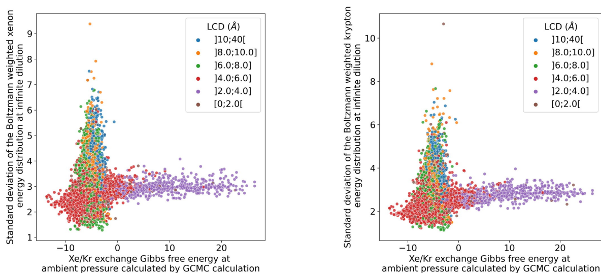
Figure 3.34 – Comparison of the ambient-pressure Xe/Kr exchange Gibbs free energy calculated by GCMC simulations of RASPA2 with 100,000 cycles and the standard deviations of the Boltzmann weighted energy distribution of xenon (left) and krypton (right) calculated by the GrAED algorithm at 298 K.
