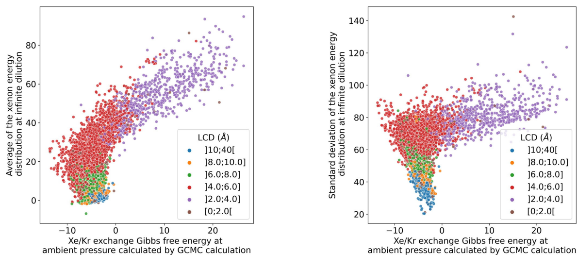
Figure 3.36 – Comparison of the ambient-pressure Xe/Kr exchange Gibbs free energy calculated by GCMC simulations of RASPA2 with 100,000 cycles and the mean values (left) and the standard deviation (right) of the uniformly weighted energy distribution of xenon calculated by the GraED algorithm at 298 K.
