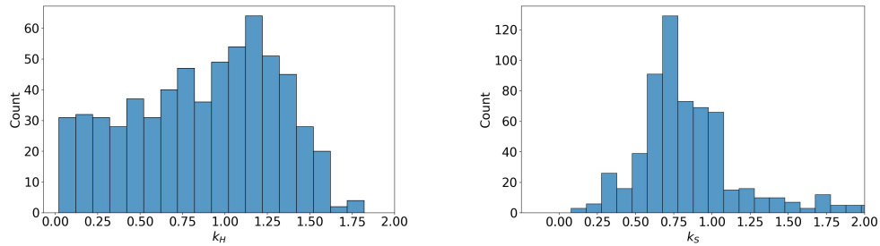
Figure 2.25 – Distribution of the enthalpic k_H and entropic k_S contributions to the change of selectivity from low to ambient pressure for the 630 materials with s_0 > 30 . k_H has a rather broad and uniform distribution, whereas k_S has a bell-like distribution.
