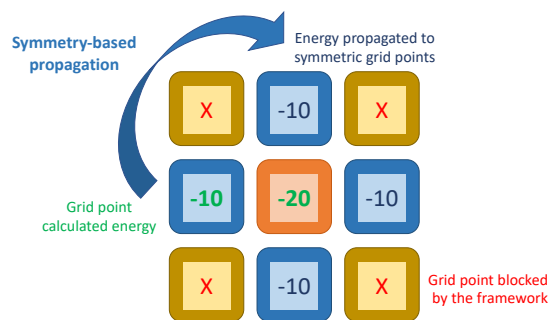
Figure 3.21 – Principle of the energy sampling on a symmetry-based grid. On the 9 grid points, 4 points are blocked because they are too close to the framework atoms, 2 points are really calculated using the LJ potential and 3 points are propagated using the inner symmetry of the framework.
