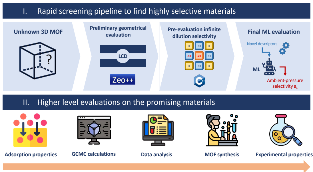
Figure 4.10 – An illustration of the screening procedure that could be used to find highly selective materials. The adsorption properties can be rapidly evaluated using structural and energetic conditions on the structure and by confirming it with the ML model. The structures chosen this way can then be tested with higher-level calculations and experiments.
