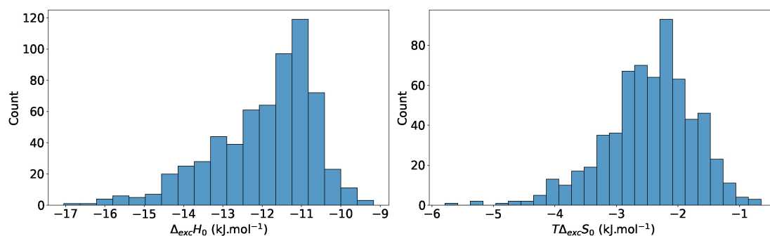
Figure 2.15 – Distribution of the enthalpy \Delta_{exc}H_0 and entropy T\Delta_{exc}S_0 of exchange at low pressure on the 630 most selective structures
