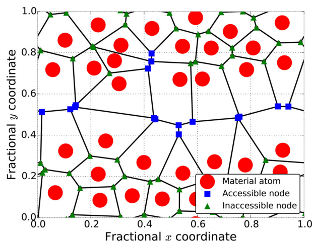
Figure 3.2 – Voronoi network model of void space (2D representation). The unit cell of a toy material is shown. Red circles represent atoms of the material; accessible and inaccessible Voronoi nodes are blue squares and green triangles, respectively. The black lines are the edges in the periodic Voronoi graph that model the void space. Reprinted with permission from Ref. [18]. Copyright 2015 American Chemical Society.
