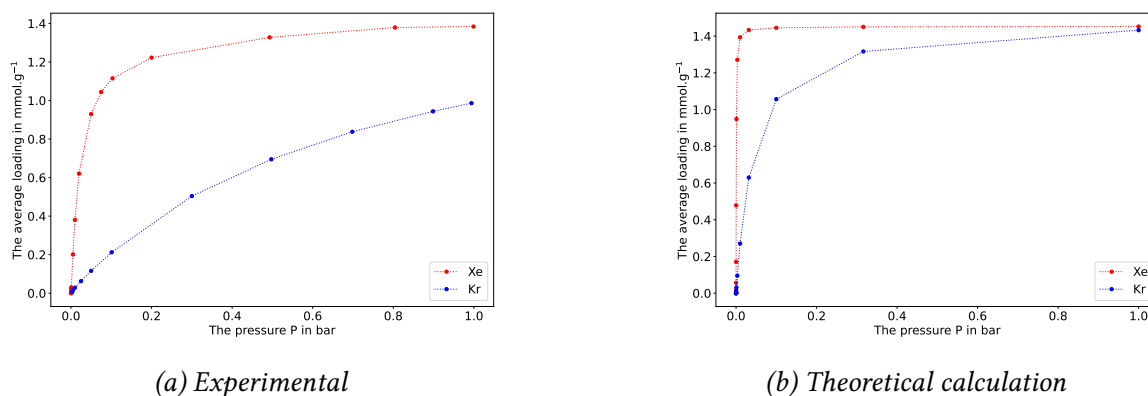
Figure 1.1 – Illustration of monocomponent adsorption isotherms of Xe and Kr obtained experimentally (a) and through GCMC calculations (b). The experimental data are made available 1 by the authors of the Ref. [41].
