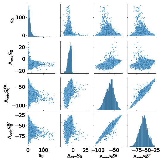
Figure 2.14 – For 8 401 MOFs with favorable thermodynamic Xe/Kr selectivity ( s_0 > 1 ), pair plots of s_0 , \Delta_{exc}S_0 , \Delta_{ads}S_0^{Xe} and \Delta_{ads}S_0^{Kr} in the off-diagonal subplots and the distribution of each quantity are on the diagonal.
