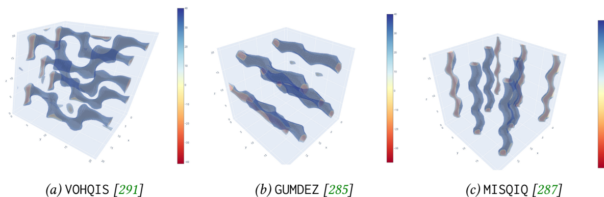
Figure 5.21 – 3D volume plot of the xenon interaction energy values inside materials with tortuous unidirectional channels calculated using an energy grid as previously described.
