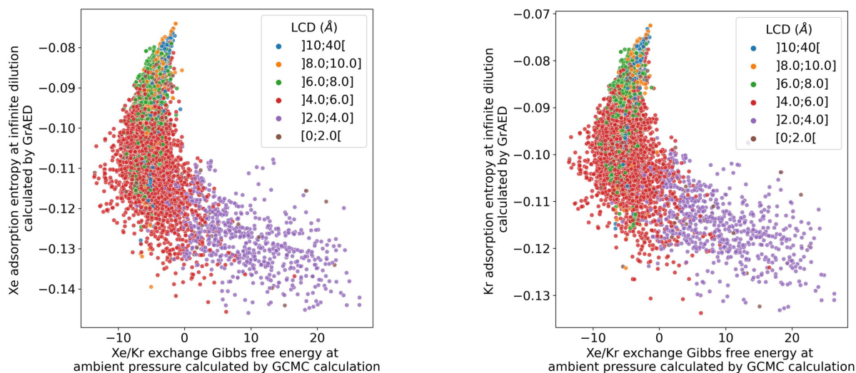
Figure 3.30 – Comparison of the ambient-pressure Xe/Kr exchange Gibbs free energy calculated by GCMC simulations of RASPA2 with 100,000 cycles and the low-pressure adsorption entropies of xenon (left) and krypton (right) in \text{kJ mol}^{-1} \text{K}^{-1} calculated by the GrAED algorithm (same parameters).
