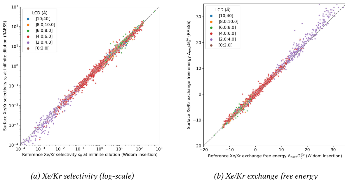
Figure 3.17 – (a) Scatterplot comparison of the Xe/Kr selectivity calculated by RAESS algorithm and the one calculated by the Widom insertion (in log scale). (b) Scatterplot comparison of the exchange Gibbs free energy \Delta_{\text{exch}}G_0^{\text{Xe/Kr}} calculated by the Widom insertion compared to the final implementation of RAESS (RMSE=0.36 kJ mol -1 and MAE=0.23 kJ mol -1 ). Both graphs are color-coded by the cavity size (LCD).
