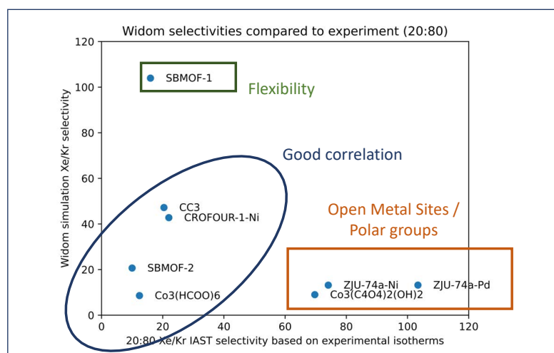
Figure 6.5 – Comparison between the selectivity values obtained experimentally and computationally. The structures are split into three categories depending on the difference between experiments and theory. The case of SBMOF-1 can be attributed to its flexibility. The discrepancies between the materials in the lower right correspond to the ones introduced by Li et al. and Pei et al., 7,8 and the difference can be explained by the polarization that is not included in the level of theory considered.
