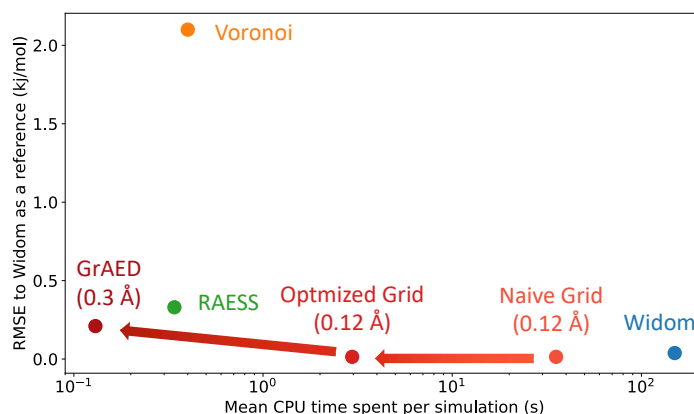
Figure 3.22 – Comparison of the RMSE on Xe adsorption enthalpy and the average CPU time required to run a simulation on a structure of CoRE MOF 2019 ( \text{LCD}_{\text{CCDC}} \geq 3.7 \text{ \AA} ) for different sampling techniques (Widom, Voronoi, RAESS and GrAED). The values are reported in Table 3.3.
