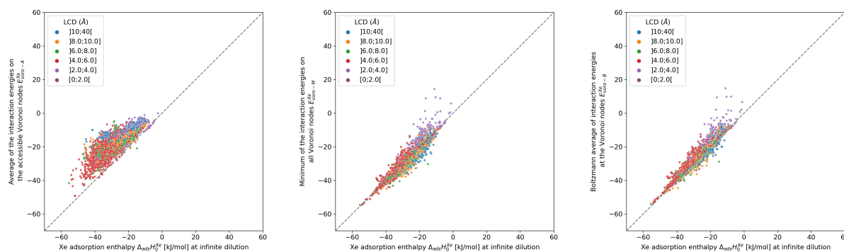
Figure 3.3 – Scatterplots of the energy descriptors E_{\text{voro-A}}^{\text{Xe}} , E_{\text{voro-M}}^{\text{Xe}} and E_{\text{voro-B}}^{\text{Xe}} calculated by a Voronoi sampling compared to the enthalpies calculated by a 100k-step Widom insertion simulation of xenon in structures of CoRE MOF 2019. The points are labeled according to the largest cavity diameter ( \text{LCD}_{\text{CCDC}} ) belonging to one of the intervals.
