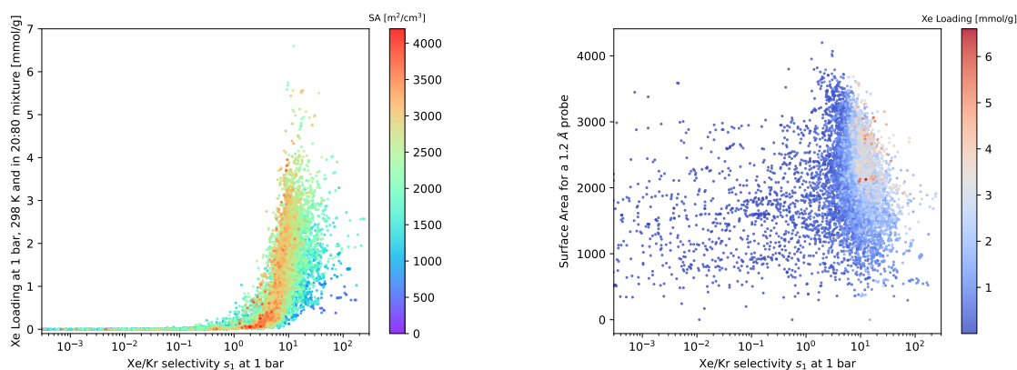
Figure 2.5 – On the left: scatterplot of the xenon uptake as a function of the selectivity and labeled by the values of the surface area (in \text{m}^2 \text{ cm}^{-3} ). On the right: scatterplot of the selectivity and the surface area labeled by the quantity of xenon adsorbed. The selectivity and uptake are calculated by a GCMC simulation of a 20:80 Xe/Kr mixture.
