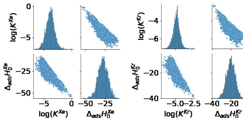
Figure 2.16 – For 8401 MOFs with favorable thermodynamic Xe/Kr selectivity ( s_0 > 1 ), pair plots of \log(K_H^i) and \Delta_{ads}H_0^i in the off-diagonal subplots for both i=Xe and i=Kr and the distribution of each quantity are on the diagonal.
