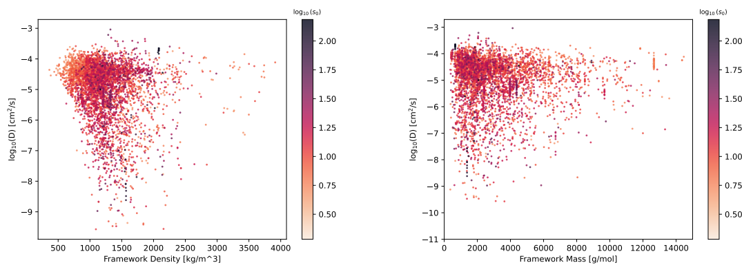
Figure 5.12 – Xenon diffusion coefficient at infinite dilution as a function of the density (left) and the mass (right) of the frameworks.
