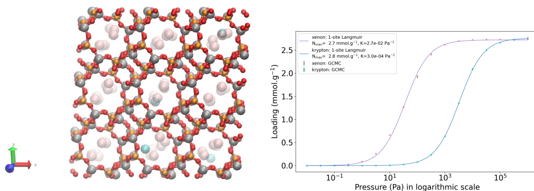
Figure 2.30 – GOMREG: Representation of a clean version (all solvent removed) of this aluminophosphate \text{AlPO}_4\text{-}n that has a zeolite LAU topology with one-dimensional 10-ring channels loaded with xenon and krypton obtained by GCMC calculations. Color code: Al in silver, P in orange, O in red; Xe in transparent pink and Kr in cyan for the adsorbates. The mono-component isotherms fitted with a 1-site Langmuir model (equation 2.33) for both xenon and krypton at 298 K is represented on the right side.
