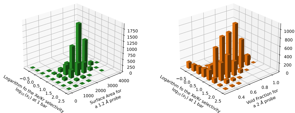
Figure 2.6 – 3D histograms of in a bidimensional space formed by the Xe/Kr selectivity and the surface areas (on the left) and formed by the Xe/Kr selectivity and the pore void fractions (on the right). A base 10 logarithm has been applied to the selectivity values. Bin size increased by 2.4 (on log scale) for the selectivity, by about 500 \text{ m}^2 \text{ cm}^{-3} for the surface areas and by 0.125 for the void fraction.
