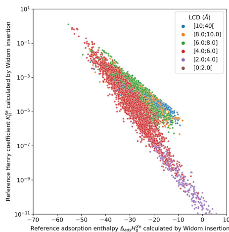
Figure 2.17 – Comparison between the Xe Henry constant and Xe adsorption enthalpy labeled by categories of LCD_{UFF} values for the CoRE MOF structures.
