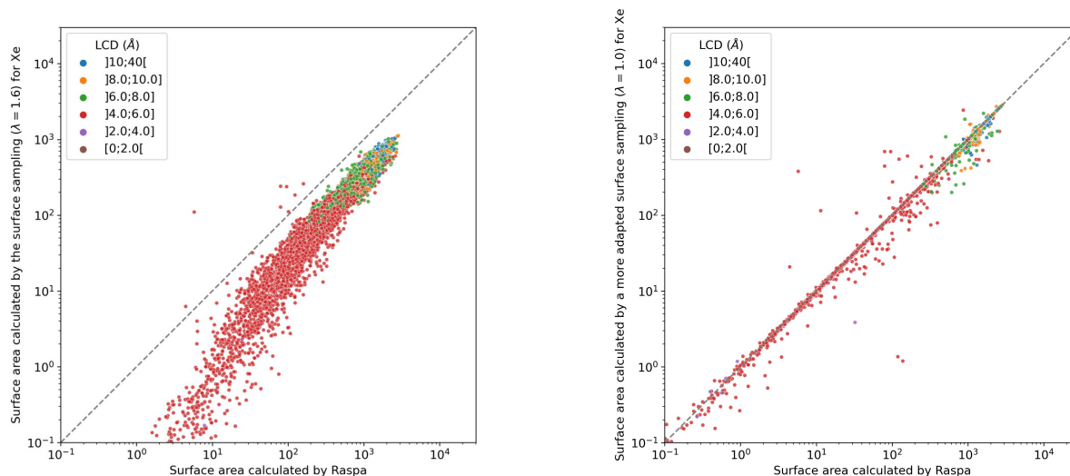
Figure 3.16 – Scatterplots of the surface areas calculated by the RAESS algorithm with two different parameterizations compared to the surface area given by a RASPA2 surface area calculation. The left plot corresponds to the surface sampling described in the section 3.2.3 with \lambda = 1.6 and \mu = 0.85 , while the right plot uses a sampling sphere near \sigma with \lambda = 1.0 . The second parameterization is much closer to what a RASPA2 sampling based on the \sigma parameter of a Lj potential does, hence explaining the much better accordance.
