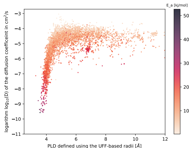
Figure 5.25 – Scatterplot of the \log_{10} of the diffusion coefficient (in \text{cm}^2 \text{s}^{-1} ) as a function of the PLD values and labeled by the barrier activation energy. The higher barriers seem to correspond to lower diffusion coefficients, thus echoing the correlation observed in the previous figure 5.24.
