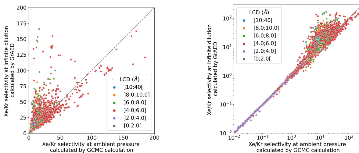
Figure 3.27 – Comparison of the low-pressure Xe/Kr selectivity calculated by the GrAED algorithm (same parameters) and the ambient-pressure selectivity calculated by GCMC simulations of RASPA2 with 100,000 cycles. On the left, the axes are in linear scale, whereas the log scale has been used on the right.
