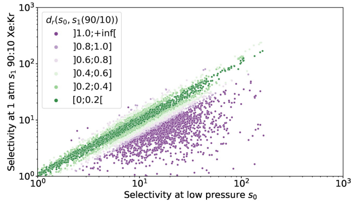
Figure 2.20 – Difference of selectivity between low pressure and at a 1013 hPa pressure for a 90:10 xenon/krypton composition. The relative difference between the low-pressure selectivity and the ambient pressure is particularly high for the points labeled in purple.
