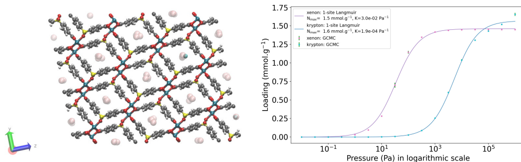
Figure 2.28 – KAXQIL: On the left side, an illustration of a clean version (all solvent removed) of the calcium coordination framework [Ca(SDB)] \cdot H_2O , where SDB = 4,4'-sulfonyldibenzoate loaded with xenon and krypton obtained by GCMC calculations. Color code: Ca in dark cyan, C in gray, O in red, H in white, S in yellow; Xe in transparent pink and Kr in cyan for the adsorbates. The mono-component isotherms fitted with a 1-site Langmuir model (equation 2.33) for both xenon and krypton at 298 K is represented on the right side.
