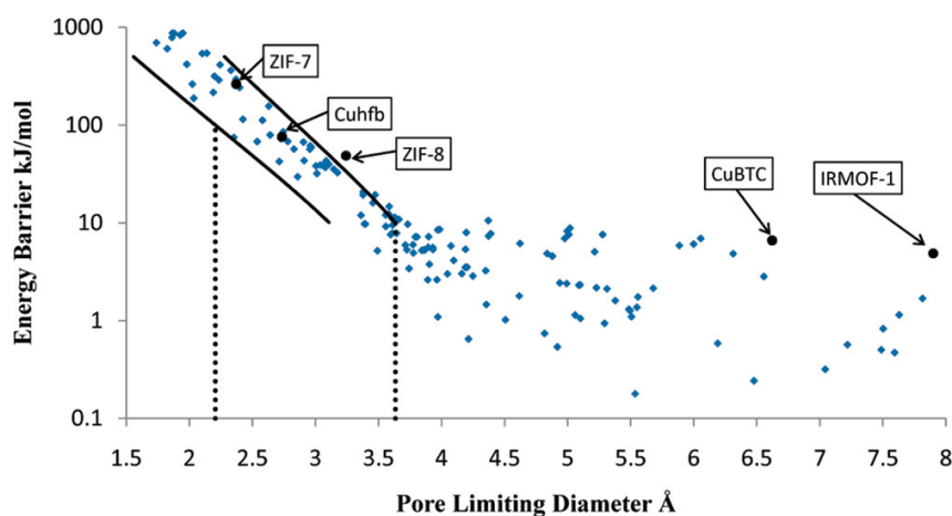
Figure 1.6 – Calculated energy barrier for the diffusion of \text{CH}_4 in 216 metal–organic frameworks (MOFs), shown as a function of the pore-limiting diameter. The solid lines represent statistical upper and lower bounds on the energy barrier, in a transition state theory approach. Reprinted with permission from Ref. [127]. Copyright © 2010 American Chemical Society.
