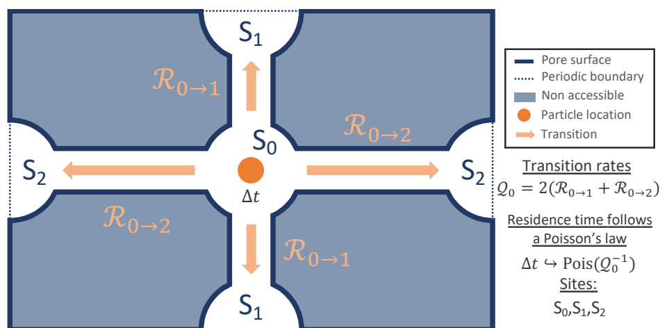
Figure 5.3 – Illustration of the core principle of lattice kinetic Monte Carlo in a periodic system. Within the periodic system, the movement of particles is governed by transition probabilities from one site to another. The transition rates are determined using the activation energy needed to move to the transition state between the two stable adsorption sites, as shown in equations 5.6 and 5.7.
