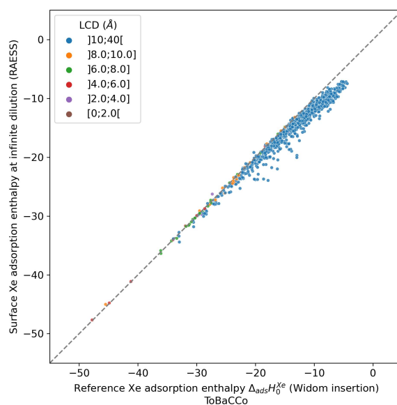
Figure 3.19 – Scatterplot comparison of the xenon adsorption enthalpy calculated by the RAESS algorithm and the Widom insertion (RASPA2) on the ToBaCCo database. RMSE = 1.79 \text{ kJ mol}^{-1} and MAE = 1.48 \text{ kJ mol}^{-1} . It can be noted that 915 structures have the LCD_{CCDC} greater than 10 Å.
