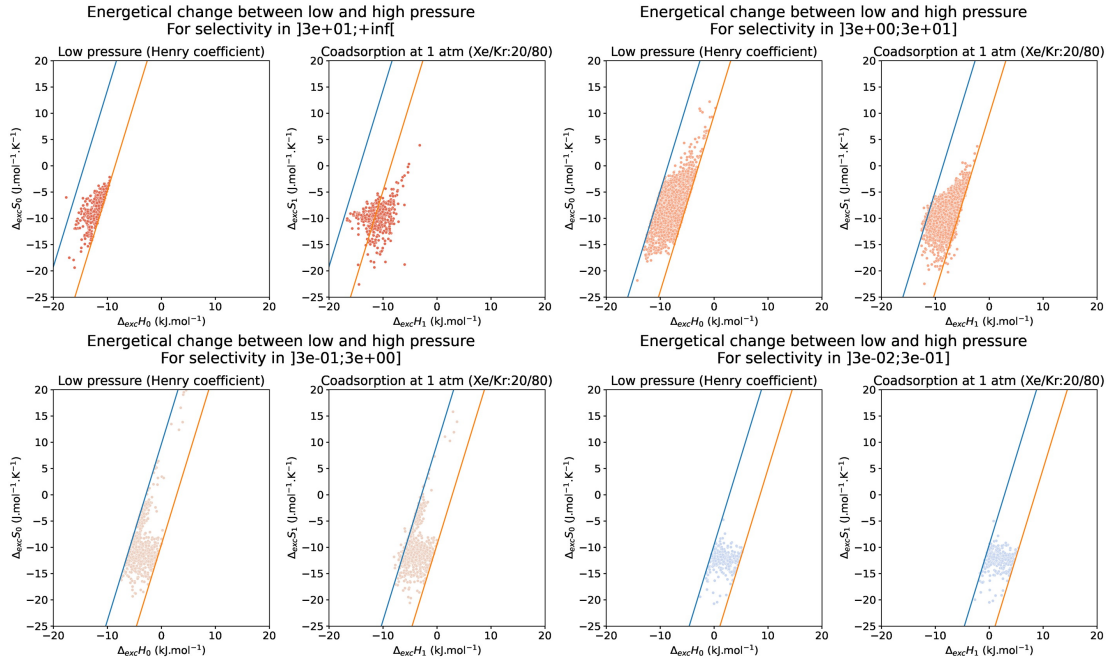
Figure 2.24 – Split view of Figure 2.21 and 2.23. The iso-selectivity lines for the limit considered are represented with blue and orange lines. It seems that the shift in exchange enthalpy for the structures with a selectivity higher than 30.
