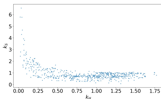
Figure 2.26 – Scatterplot of the enthalpic contribution k_H and entropic contribution k_S for the 630 materials with s_0 > 30 . The entropic compensation occurs when the enthalpic contribution is around 0.1, else its value is around 1 and has little effect on the selectivity change.
