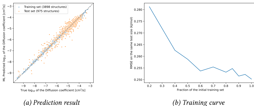
Figure 5.26 – (a) Comparison of the \log_{10} of the diffusion coefficient predicted by an ML model and the true values. (b) Root mean squared errors on the same test set (20% of all data) as a function of the fraction of the training set used to train smaller models. The error decreases as the amount of data increases and seems to stabilize near 0.25.
