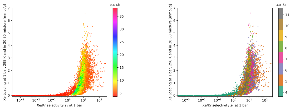
Figure 2.8 – Scatterplot of the xenon uptake as a function of the selectivity (20:80) and labeled by the values of LCD_{UFF} (left). The same scatterplot restricted to values of D_i between (3.6 and 11.6 Å) and labeled using a different color code to distinguish the most selective materials from the least selective ones. The most selective materials are colored in orange corresponding to a pore size adapted for xenon adsorption (around 5 Å). The least selective ones are in green, with a pore lower than the size of a xenon hence preventing its adsorption.
