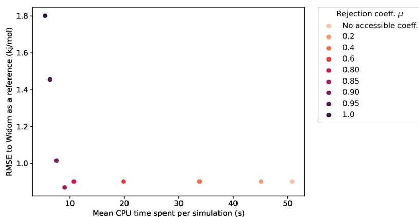
Figure 3.11 – Influence of the rejection coefficient \mu on the average CPU time required for a simulation of 100k sampling points and the RMSE compared to the reference adsorption enthalpy. The averaging is done only on the structures with the largest cavity diameter ( LCD_{CCDC} ) superior to 3.7 Å.
