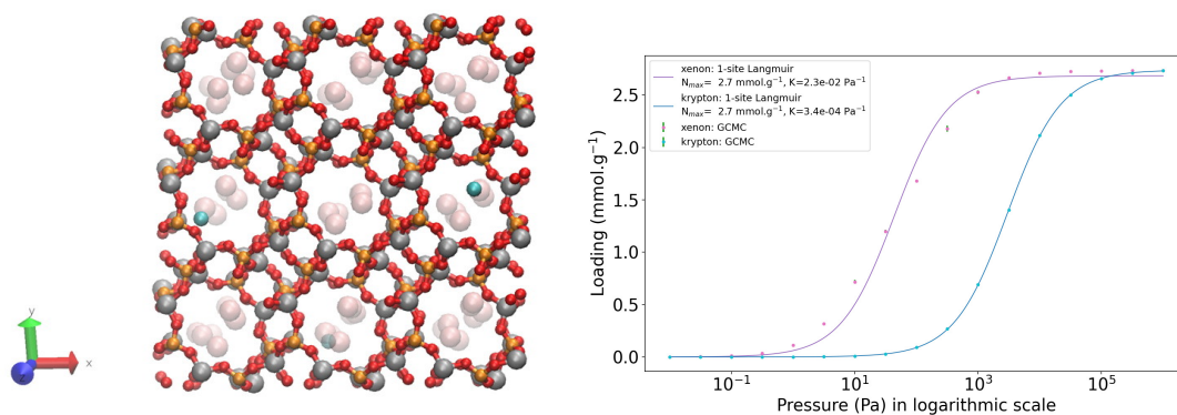
Figure 2.31 – GOMRAC: Representation of a clean version (all solvent removed) of this aluminophosphate ALPO_4-n that has a zeotype LAU topology with one-dimensional 10-ring channels loaded with xenon and krypton obtained by GCMC calculations. Color code: Al in silver, P in orange, O in red; Xe in transparent pink and Kr in cyan for the adsorbates. The mono-component isotherms fitted with a 1-site Langmuir model (equation 2.33) for both xenon and krypton at 298 K is represented on the right side. It seems that this aluminophosphate is just a smaller version of GOMREG.
