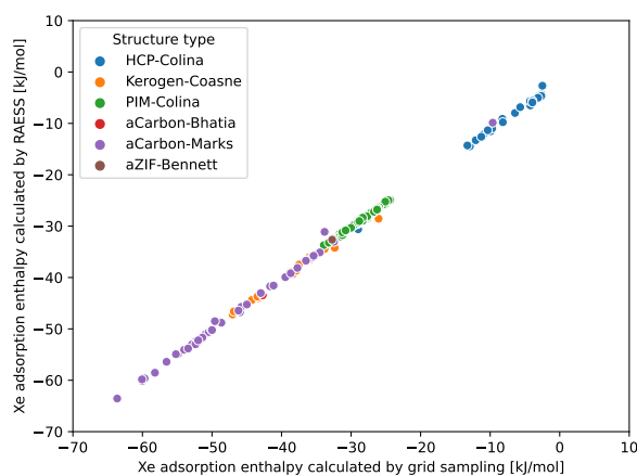
Figure 3.20 – Scatterplot comparison of the xenon adsorption enthalpy calculated by the RAESS algorithm and the one calculated by a grid sampling (presented in the next section) on a database of porous rigid amorphous materials. 56 RASPA2 simulation could not be run on this database. Only the 175 structures computed by both methods are presented here.
