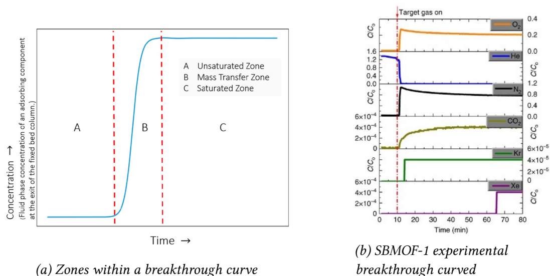
Figure 6.1 – (a) Different zones in a breakthrough curve reprinted from the open-access article [294]. (b) Experimental breakthrough curves in SBMOF-1 for a gas mixture with 400 ppm Xe and 40 ppm Kr balanced with dry air. Reprinted with permission from Ref. [41] copyright © 2016 Springer Nature.
