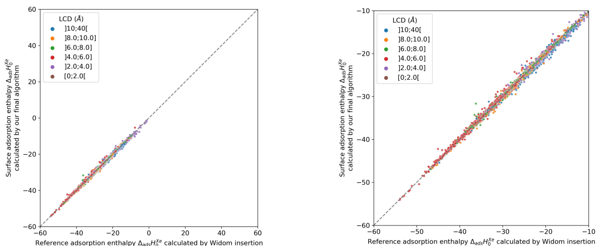
Figure 3.12 – Scatterplots of the xenon surface adsorption enthalpy calculated by the final RAESS algorithm ( \lambda = 1.6 and \mu = 0.85 ) as a function of the xenon adsorption enthalpy calculated by a 100k-step Widom insertion simulation using two value windows, in structures of CoRE MOF 2019 with LCD_{CCDC} \geq 3.7 Å at 298 K. The second plot zooms on the negative values corresponding to the most selective materials.
