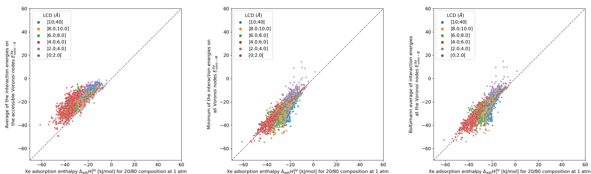
Figure 3.5 – Scatterplots of the energy descriptors E_{\text{voro-A}}^{\text{Xe}} , E_{\text{voro-M}}^{\text{Xe}} and E_{\text{voro-B}}^{\text{Xe}} calculated by a Voronoi sampling compared to the enthalpies calculated by a 100k-step GCMC simulation of xenon in structures of CoRE MOF 2019. The points are labeled according to the largest cavity diameter ( \text{LCD}_{\text{CCDC}} or D_i ) belonging to one of the intervals.
