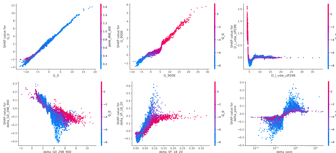
Figure 4.12 – Some relevant SHAP dependence plots that are provided here. A SHAP dependence plot corresponds to the Shapley values as a function of the feature values for all structures of the dataset. These SHAP plots show the contribution of the features to the prediction given by the ML model. Each Shapley value depends not only on the value of the feature itself but also on the values of other features. For this reason, the plots are labeled by a relevant second feature.
