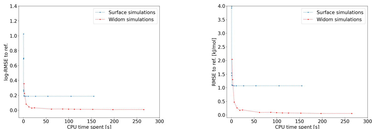
Figure 3.15 – Left: convergence plot of the log-RMSE on the xenon Henry constants for both the surface sampling and the Widom insertion. Right: convergence plot of the RMSE on the xenon adsorption Gibbs free energy for the final implementation of the surface sampling and the Widom insertion.
