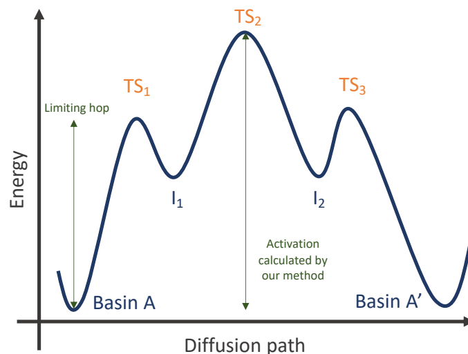
Figure 5.23 – Multistep diffusion from a basin A to a basin A'. The diffusion process is modeled by transition states TS_1 , TS_2 and TS_3 and intermediate steps I_1 and I_2 . In this particular case, there is a difference between the real limiting activation energy and the activation energy calculated by the simplified method.
