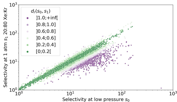
Figure 2.19 – Difference of selectivity between low pressure and at a 1013 hPa pressure for a 20:80 xenon/krypton composition. The relative difference between the low-pressure selectivity and the ambient pressure is particularly high for the points labeled in purple.
