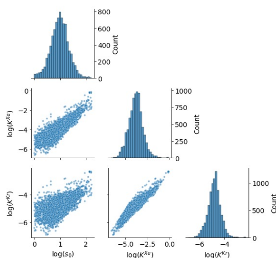
Figure 2.12 – For 8 401 MOFs with favorable thermodynamic Xe/Kr selectivity ( s_0 > 1 ), pair plots of \log_{10}(s_0) , \log_{10}(K^{\text{Xe}}) and \log_{10}(K^{\text{Kr}}) (the Henry constants are in \text{mmol g}^{-1} \text{Pa}^{-1} ) in the off-diagonal subplots (note that the y-axis is displayed on the right side) and the distribution of each quantity are on the diagonal (note that the y-axis displayed on the right side corresponds to the count and the x-axis is correctly labeled below each subplot).
