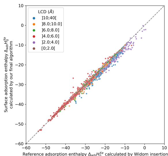
Figure 3.18 – Scatterplot of the enthalpies calculated by our final algorithm ( \lambda = 1.6 and \mu = 0.85 ) compared to the enthalpies calculated by a 12k step Widom insertion simulation of xenon in structures of CoRE MOF 2019 with LCD_{CCDC} \geq 3.7 \text{ \AA} at 600 K.
