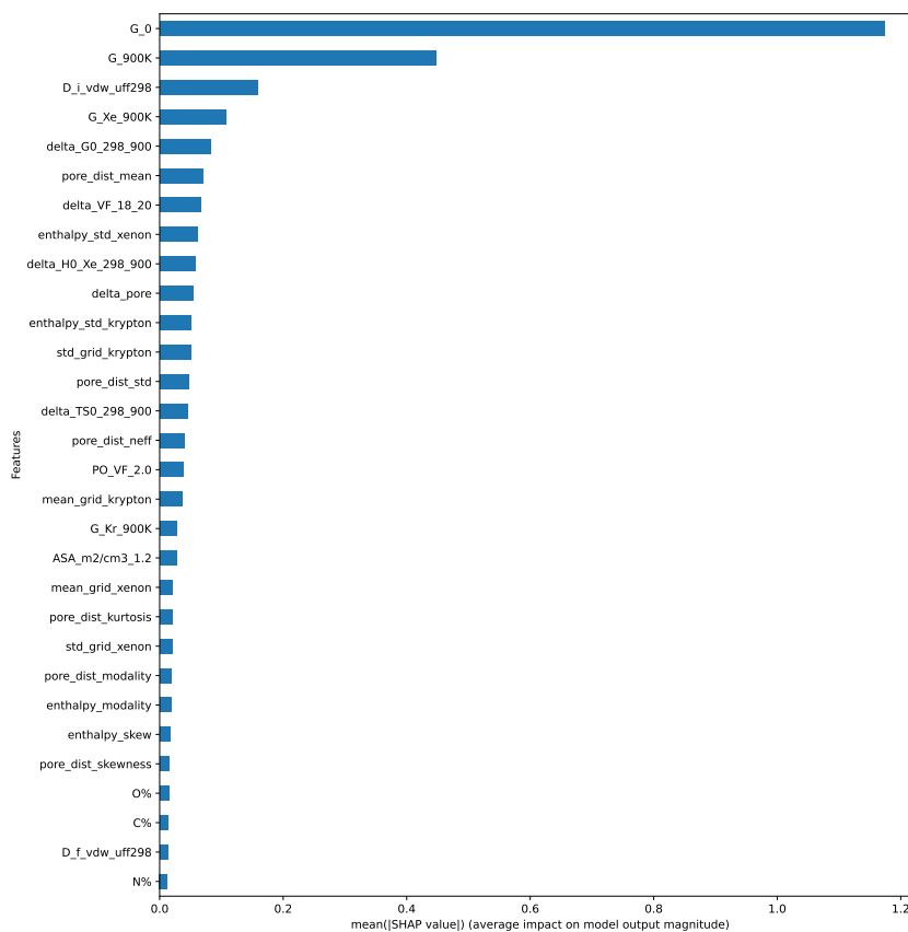
Figure 4.11 – Barplot of the feature importance for all the descriptors of our final model. The descriptor labels used in this section are explained in more detail in Tables 4.2 and 4.3.
