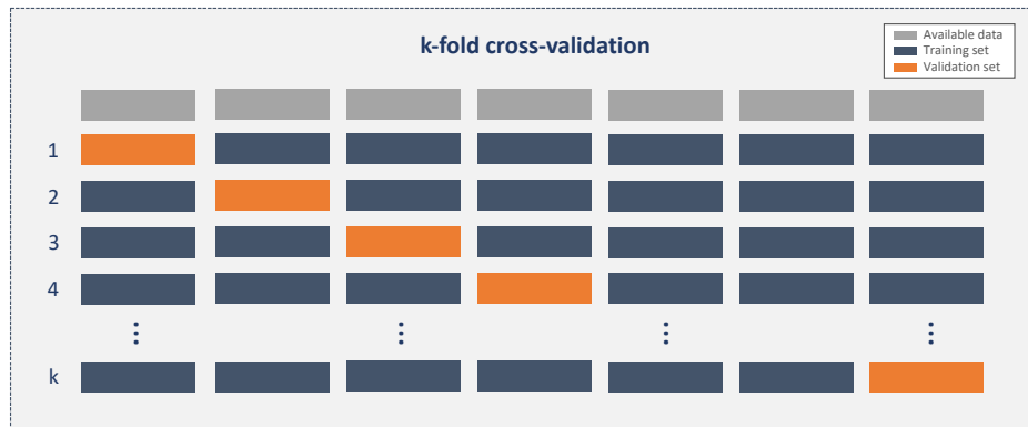
Figure 4.4 – Illustration of a k -fold cross-validation. At each step, the machine learning model learns from the training set and is tested on the validation set. The average performance on all validation sets gives an approximation of the generalization error.
