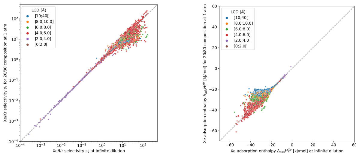
Figure 3.4 – Comparison of the ambient-pressure and low-pressure case through two thermodynamic quantities: the Xe/Kr selectivity (left) and the xenon adsorption enthalpy (right).
