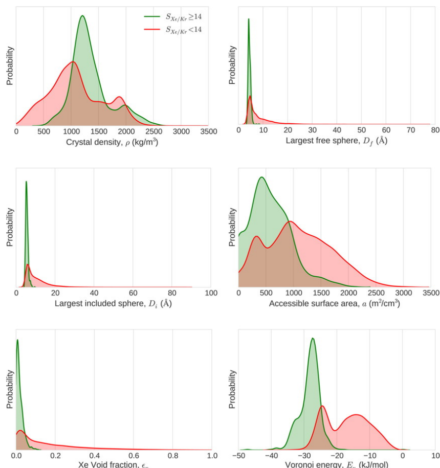
Figure 1.11 – Statistical analysis of the adsorption separation of xenon/krypton mixtures by nanoporous materials. The graphs represent the distributions of structural descriptors explored by highly selective (green) and poorly selective (red) materials separately. Reprinted with permission from Ref. [18]. Copyright © 2015 American Chemical Society.
