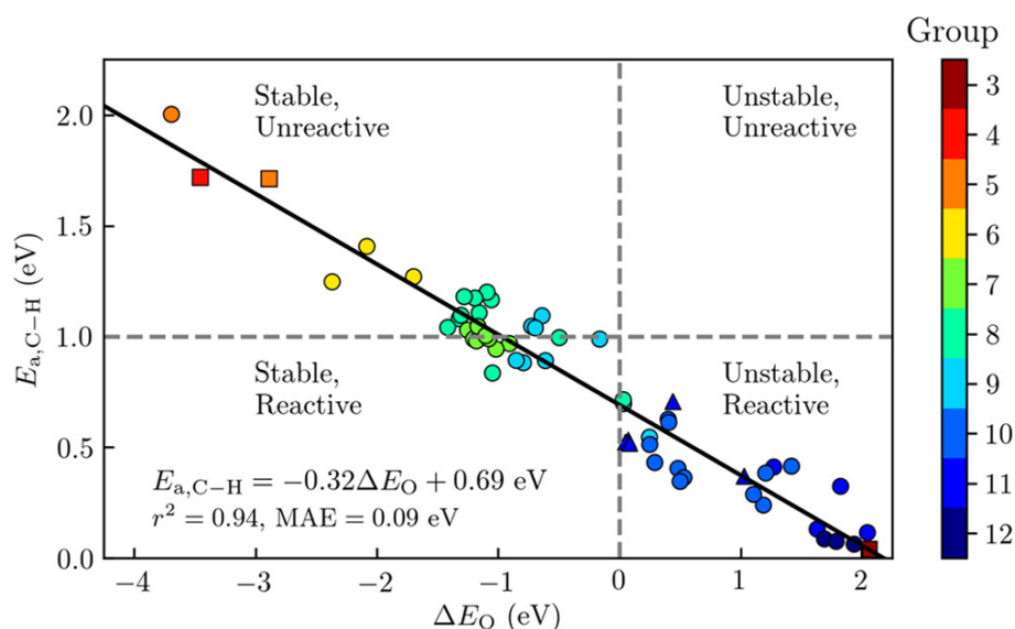
Figure 1.4 – Analysis of a diverse set of experimentally derived metal–organic frameworks (MOFs) with accessible metal sites for the oxidative activation of methane. The graph shows the predicted barrier for the C–H bond activation of methane, E_a , as a function of the metal-oxo formation energy, \Delta E_O . For each material, the symbol color refers to the group number of the metal in the periodic table. The best-fit line has been plotted in black, and has a mean absolute error (MAE) of 0.09 eV. MOFs with E_a < 1 eV are classified as being reactive towards C–H bond activation and MOFs with \Delta E_O < 0 as having thermodynamically favored active sites when using \text{O}_2 as the reference state. Reprinted with permission from Ref. [106]. Copyright © 2019 American Chemical Society.
