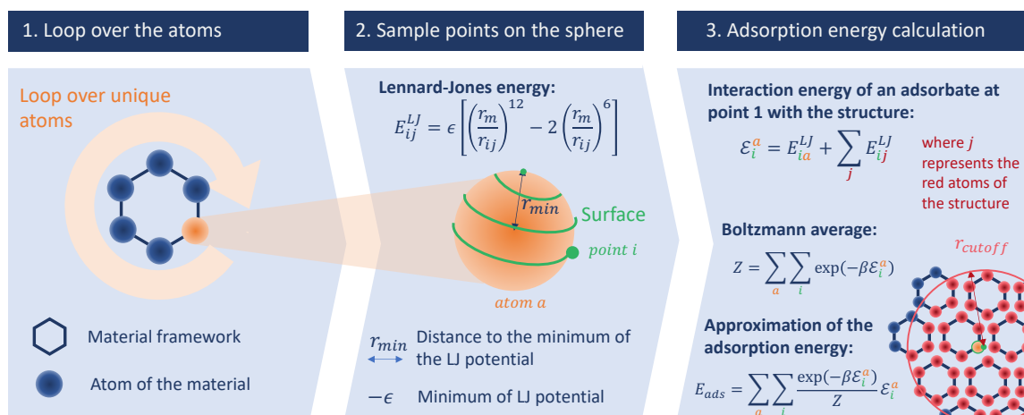
Figure 3.6 – Schematic description of the surface sampling based on the three main steps of the algorithm: the loop over the unique atoms, the spiral sampling around each atom, and the energy averaging. The adsorbate is represented by the point i and is moved across all the points around the unique atoms of the structure.
