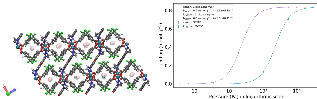
Figure 2.29 – JUFBIX: Representation of a clean version (all solvent removed) of the cobalt(II) coordination framework [Co_2(L)(ppda)_2]_2 \cdot H_2O , where the ligand L is 2,8-di(1H-imidazol-1-yl)dibenzofuran and the carboxylic acid ligand H_2ppda is 4,4'-(perfluoropropane-2,2-diyl)dibenzoic acid loaded with xenon and krypton obtained by GCMC calculations. Color code: Co in dark cyan, C in gray, O in red, H in white, N in blue, F in green; Xe in transparent pink and Kr in cyan for the adsorbates. The mono-component isotherms fitted with a 1-site Langmuir model (equation 2.33) for both xenon and krypton at 298 K is represented on the right side.
