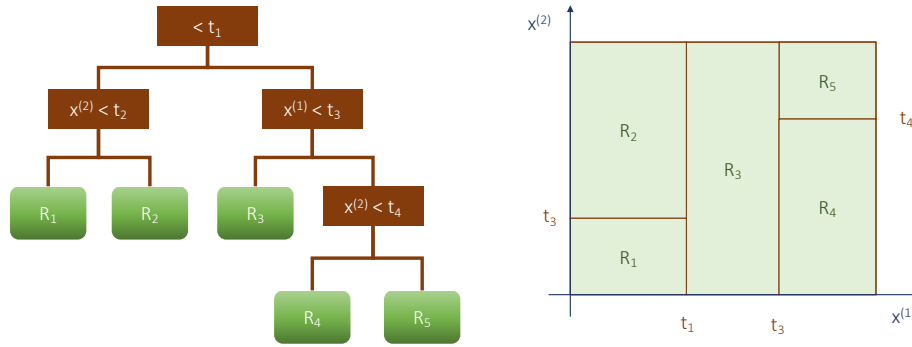
Figure 4.5 – Illustration of the decision tree and the region splitting performed by a CART 241 algorithm. Adapted from an illustration of the book “Elements of Statistical Learning” [239].
