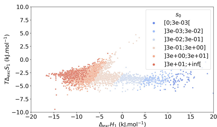
Figure 2.23 – The energetic equivalent of exchange entropy T\Delta_{exc}S_1 and enthalpy \Delta_{exc}H_1 at ambient pressure (for a 20:80 xenon/krypton composition) labeled using the selectivity s_0 at low pressure. The points are layered so that the points with higher s_0 are always above. To see a split version of this plot, please refer to Figure 2.24.
