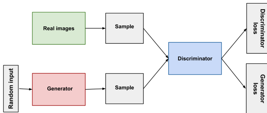
Figure 2.3: The GAN architecture [51]
