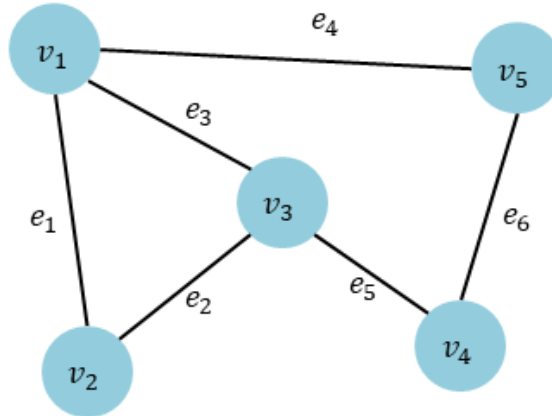
Figure 4.1: Example of a graph with 5 nodes and 6 edges.
