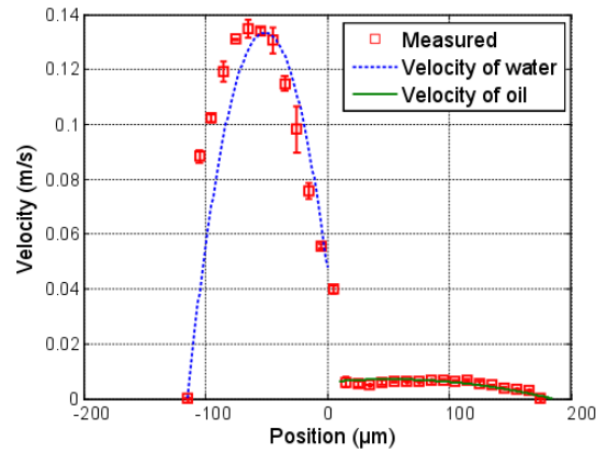
Fig. 4.20. Measured maximum velocity profile with the dual lens configuration and theoretical fitting for water pumped at 60 \mu\text{L}/\text{min} and oil pumped at 4.5 \mu\text{L}/\text{min} . Reference image is shown in Fig. 4.20(b).
