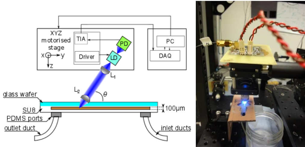
Fig. 4.14. Scheme of the experimental setup incorporating a blue-violet laser (left). Real OFI sensor (right).
