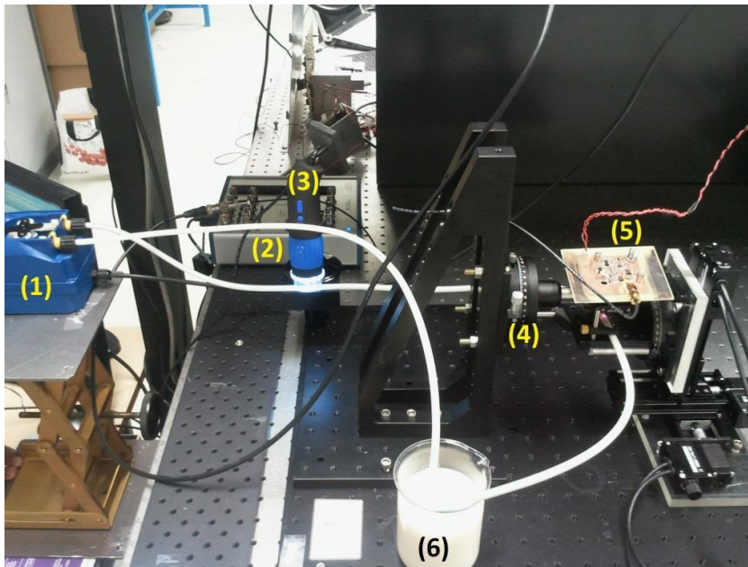
Fig. 3.29. Experimental setup: (1) peristaltic pump, (2) acquisition card, (3) camera, (4) goniometer, (5) laser and associated electronics, (6) fluid.
