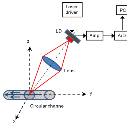
Fig. 3.2. Schematic representation of the sensing system. The laser is located at twice the focal distance from the lens and focalized in the center of the cylindrical channel.
