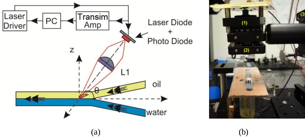
Fig. 4.6. Simplified set-up configuration using single lens optics for optical feedback velocity measurement of parallel oil-water flows (a). Real set-up used during the measurements (b): (1) Laser, (2) Lens, (3) Goniometer and (4) SU8 Y-shaped microreactor.
