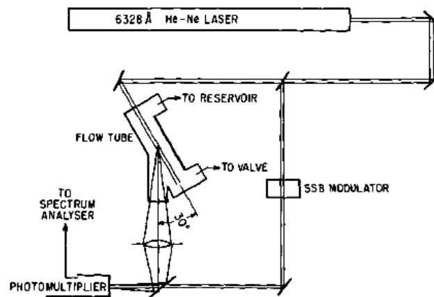
Fig. 1.1. Original Laser Doppler velocimeter set-up proposed by Yeh and Cumins in 1964.
