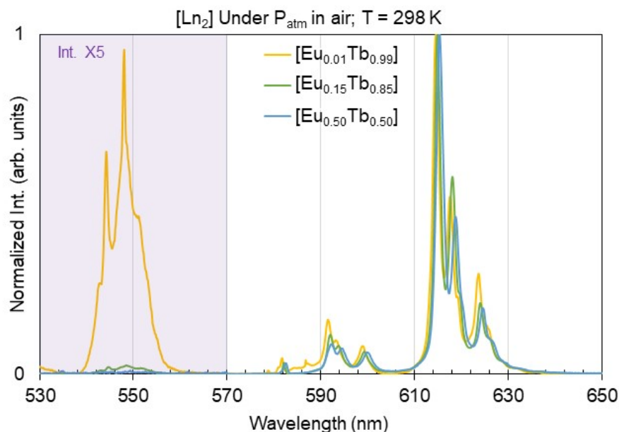
Figure 4.13: Emission spectra of [\text{Ln}_2] complexes at [\text{Eu}_{0.01}\text{Tb}_{0.99}] , [\text{Eu}_{0.15}\text{Tb}_{0.85}] and [\text{Eu}_{0.50}\text{Tb}_{0.50}] shown in yellow, green, and blue, respectively (Emission intensity is normalized by the most intense peak).
