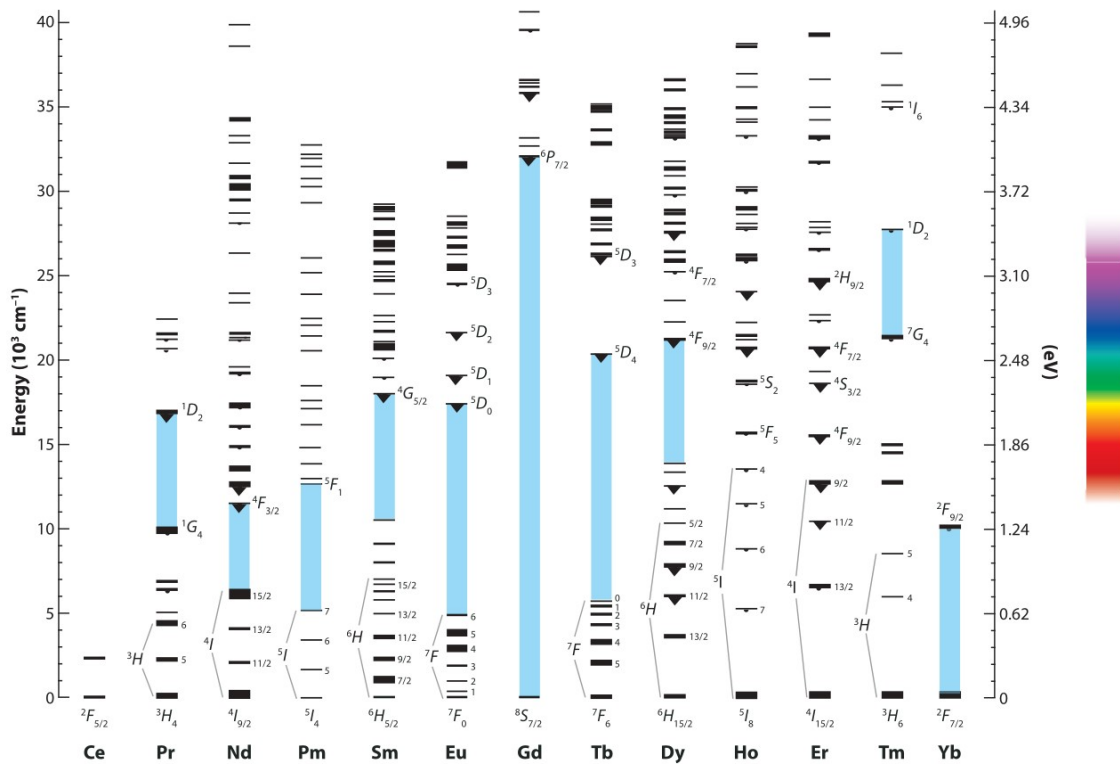
Figure 1.7: Dieke energy diagram for trivalent lanthanide ions, the largest energy gaps are shaded in blue. (Scheme from ref. 74 , M.D. Chambers and D. R. Clarke, 2009. Copyright © Annual Review of Materials Research)
