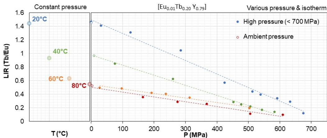
Figure 4.28: The variation of LIR in complex [\text{Eu}_{0.01}\text{Tb}_{0.20}\text{Y}_{0.79}(\text{acac})_3(\text{phen})] under constant pressure (ambient pressure outside DAC) and under various pressures in isotherm medium at 20 °C (293 K) in blue, 40 °C (313 K) in green, 60 °C (333 K) in orange, and 80 °C (353 K) in red (in DAC).
