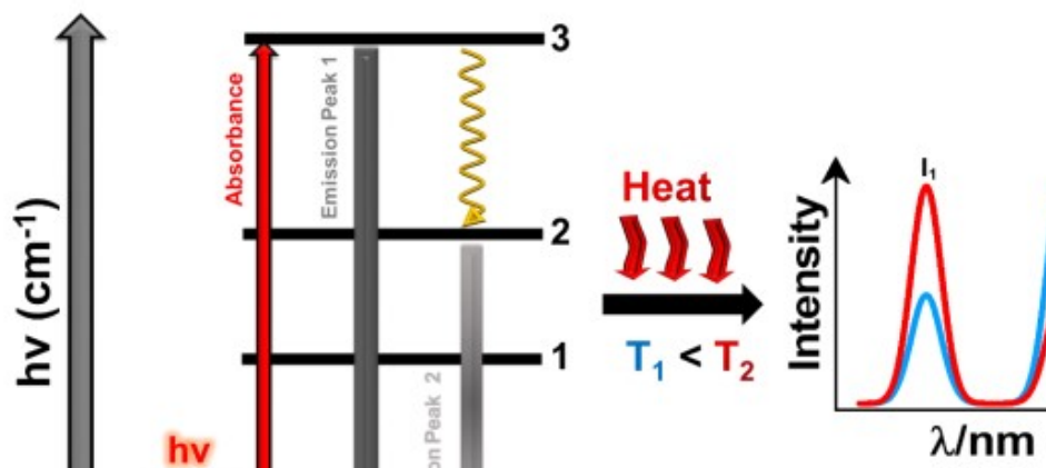
Figure 1.16: Temperature-induced photons promotion according to the Boltzmann distribution (Scheme from ref. 186 , A. Nexha. Thesis in 2020. Copyright © Hal. Universitat Rovira I Virgli)
