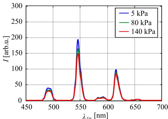
Figure 1.24: Effect of pressure on the emission spectrum of [\text{Tb}_{0.99}\text{Eu}_{0.01}(\text{hfa})_3(\text{dpbp})]_n (hfa: hexafluoroacetylacetonate, dpbp: 4,4'-bis(biphenylphosphoryl)biphenyl), respectively) in the polymer. (Scheme from ref. 116 , M. Kasai et al. 2020. Copyright © Sensors)
