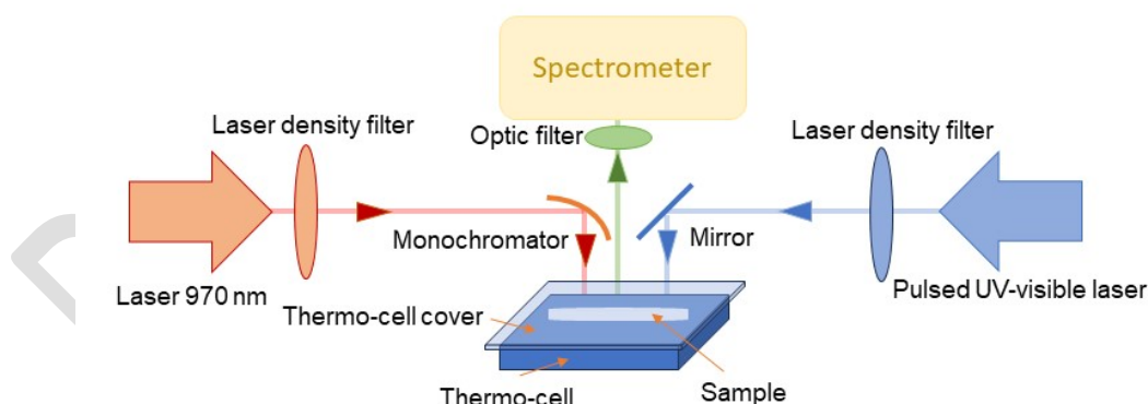
Scheme 3.1: Experimental set-up for photoluminescent temperature calibration.
