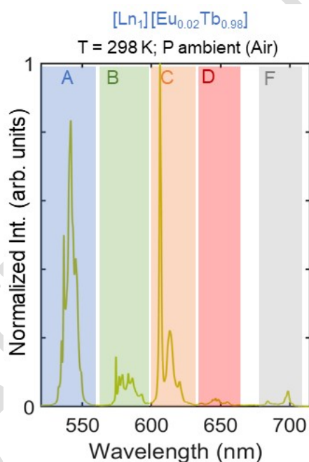
Figure 4.20: Distribution of the emission peak in the complex [Eu_{0.02}Tb_{0.98}(acac)_3(phen)] : A for {}^5D_4 to {}^7F_5 ( Tb^{3+} ), B for {}^5D_0 to {}^7F_{0\&1} ( Eu^{3+} ) and {}^5D_4 to {}^7F_4 ( Tb^{3+} ), C for {}^5D_0 to {}^7F_2 ( Eu^{3+} ) and {}^5D_4 to {}^7F_3 ( Tb^{3+} ), D for {}^5D_0 to {}^7F_3 ( Eu^{3+} ) and {}^5D_4 to {}^7F_{2\&1} ( Tb^{3+} ), and F for {}^5D_0 to {}^7F_4 ( Eu^{3+} ).
