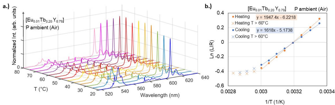
Figure 4.27: The [\text{Eu}_{0.01}\text{Tb}_{0.20}\text{Y}_{0.79}] complex under ambient pressure: a) Emission spectra under 405 nm excitation at different temperatures, b) temperature calibration curve for the luminescent intensity ratio (LIR) Tb/Eu.
