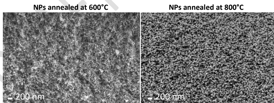
Figure 2.7: SEM images of NPs \text{GdVO}_4: \text{Yb}^{3+}/\text{Er}^{3+} powder annealed at 600^\circ\text{C} and 800^\circ\text{C} .
