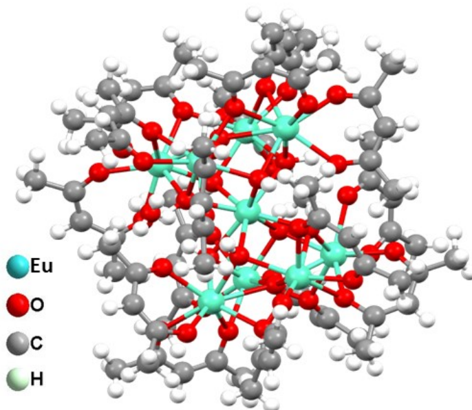
Figure 4.3: Structure of the [Ln_9] complex [Eu_9(acac)_{16}(\mu_3-OH)_8(\mu_4-O)(\mu_4-OH)] .
