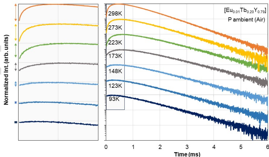
Figure 4.29: Decay time of ^5D_0 ( Eu^{3+} ) in [Eu_{0.01}Tb_{0.2}Y_{0.79}(acac)_3(phen)] at different temperatures. Insert: zoomed graph in the range of 0–0.5 ms (excitation at 486 nm; Eu^{3+} emission at 612 nm).
