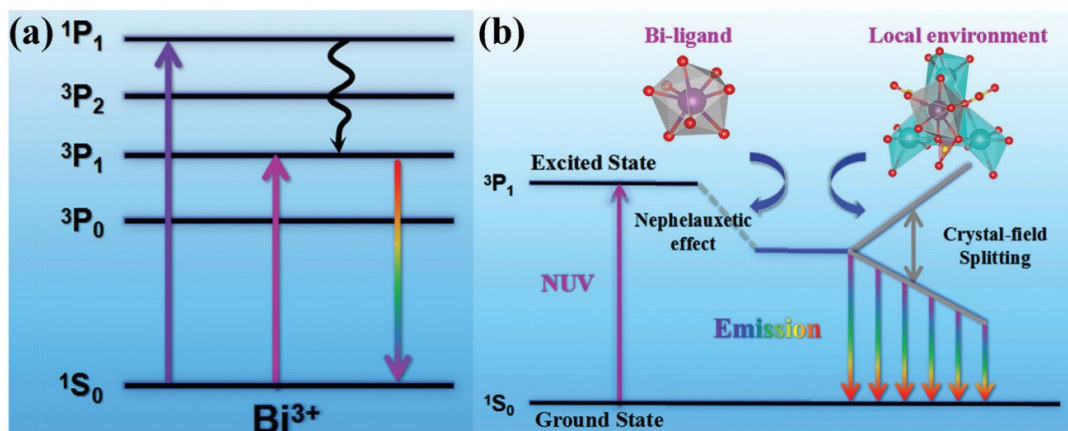
Figure 1.21: a.) Energy level scheme of \text{Na}_2\text{Y}_2\text{B}_2\text{O}_7:\text{Bi}^{3+} ions. (b) Both the nephelauxetic effect and crystal-field splitting control the \text{Bi}^{3+} emission. (Figure from ref. 229 , S. Wu, et al. 2020. Copyright © Journal of Materials Chemistry C)
