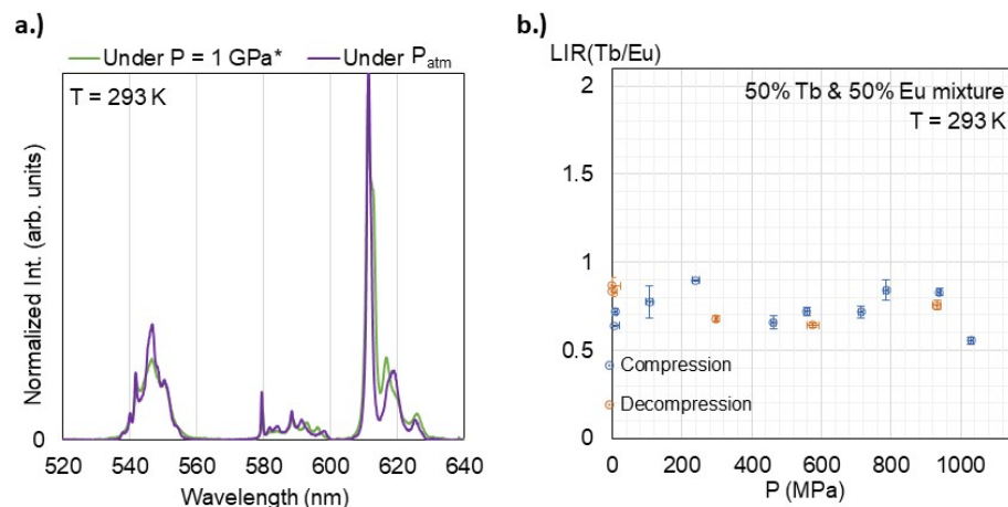
Figure 4.23: a) Emission spectra under hydrostatic pressure (in DAC) up to 1030 MPa* for a physical mixture of [\text{Eu}(\text{acac})_3(\text{phen})] and [\text{Tb}(\text{acac})_3(\text{phen})] . b) The calibration curve of the calculated LIR as a function of pressure (MPa). (LIR values are the averages of three subsequent measurements, the error bar is calculated by the standard deviation).
