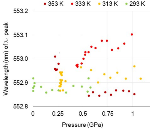
Figure 3.15: \text{GdVO}_4:\text{Yb}^{3+}/\text{Er}^{3+} suspended at 0.5 wt.% in DAC upon NIR laser at 13.5 \text{ W/cm}^2 , corrected position of \text{Er}^{3+} emission peak (transition ^4\text{S}_{3/2} \rightarrow ^4\text{I}_{15/2} ) under pressure at different temperatures.
