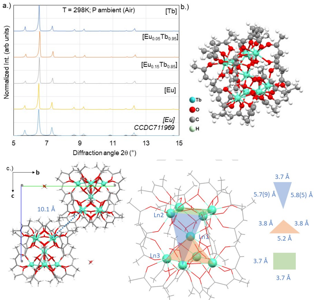
Figure 2.17: a) X-Ray diffraction patterns of [Ln 9 (acac) 16 (μ 3 -OH) 8 (μ 4 -O)(μ 4 -OH)] with different compositions, reference [Eu 9 (acac) 16 (μ 3 -OH) 8 (μ 4 -O)(μ 4 -OH)] (CCDC 711969). b)
