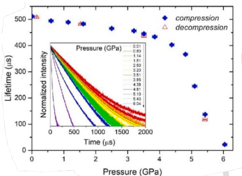
Figure 1.23: Determined luminescence lifetimes as a function of pressure, for \text{Eu}^{3+} in \beta -diketonate halogen-substituted complexes ( \lambda_{\text{exc}} = 355 \text{ nm} , \lambda_{\text{em}} = 613 \text{ nm} ). Inset shows the luminescence decay curves recorded at different pressure values. (Scheme from ref. 108 , H. Wong et al. 2022. Copyright © Chemical Engineering Journal Advances)
