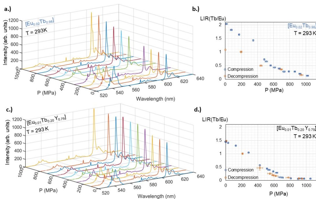
Figure 4.22: Emission spectra under hydrostatic pressure (in DAC) up to 1000 MPa for a) [Eu_{0.02}Tb_{0.98}(acac)_3(phen)] and c) [Eu_{0.01}Tb_{0.20}Y_{0.79}(acac)_3(phen)] , and their calibration curve of calculated LIR as a function of pressure (MPa) in b) and d), respectively. (LIR values are the averages of three subsequent measurements, the error bar is calculated by the standard deviation).
