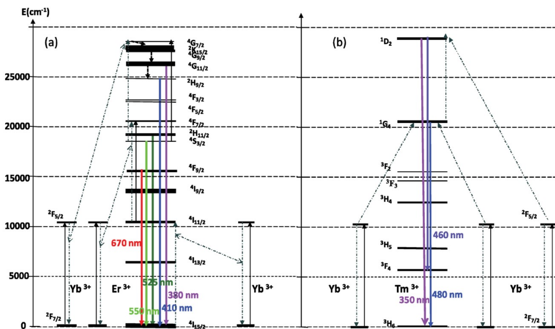
Figure 1.15: Schematic energy level diagrams showing cooperative sensitization and energy transfer up-conversion for the \text{Yb}^{3+}/\text{Er}^{3+} and \text{Yb}^{3+}/\text{Tm}^{3+} systems. (Scheme from ref. 128 , S. Mishra et al. 2012. Copyright © Dalton Transactions)
