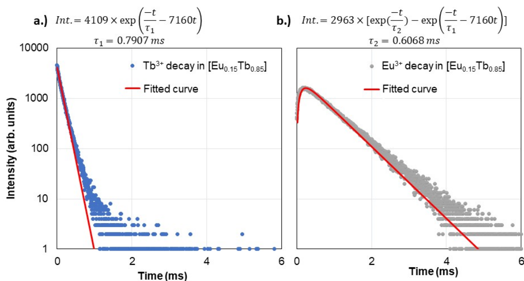
Figure 4.15: Experimental curve and fitted curve of lifetime measurements of a) \text{Tb}^{3+} and b) \text{Eu}^{3+} in the [\text{Eu}_{0.15}\text{Tb}_{0.85}] complex in air, \text{Tb}^{3+} emission at 550 nm and \text{Eu}^{3+} emission at 612 nm under 405 nm excitation.
