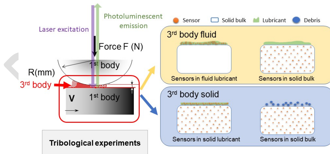
Figure 1.3: Conception of PL temperature and pressure sensing materials and their application in tribological contact.
