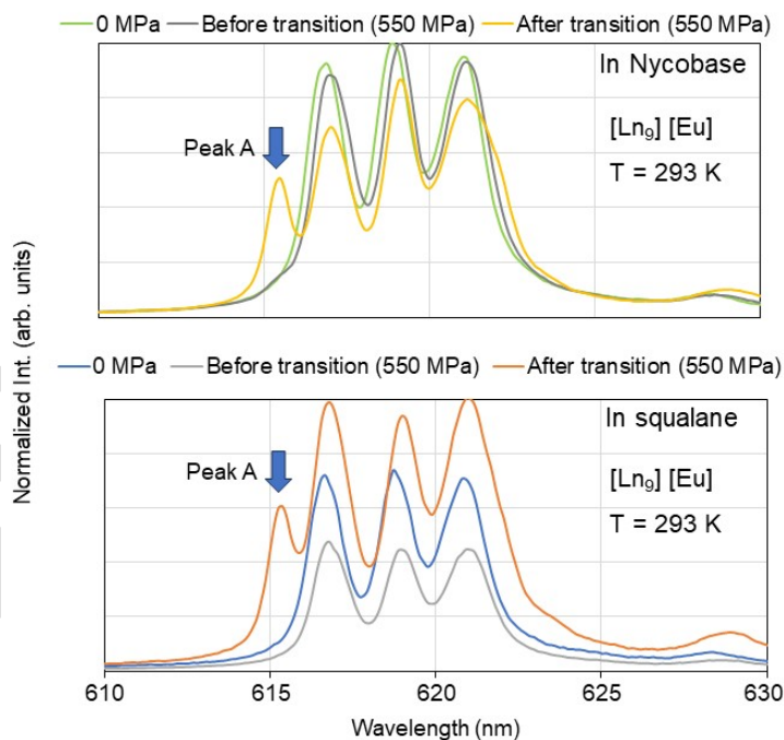
Figure 4.5: Zoomed emission spectra of [\text{Eu}_9(\text{acac})_{16}(\mu_3\text{-OH})_8(\mu_4\text{-O})(\mu_4\text{-OH})] at 550 MPa in Nycobase (on the top) and in Squalane (on the bottom) (Emission intensity is normalized by the most intense peak, peak positions are not corrected by the intensity reference).
