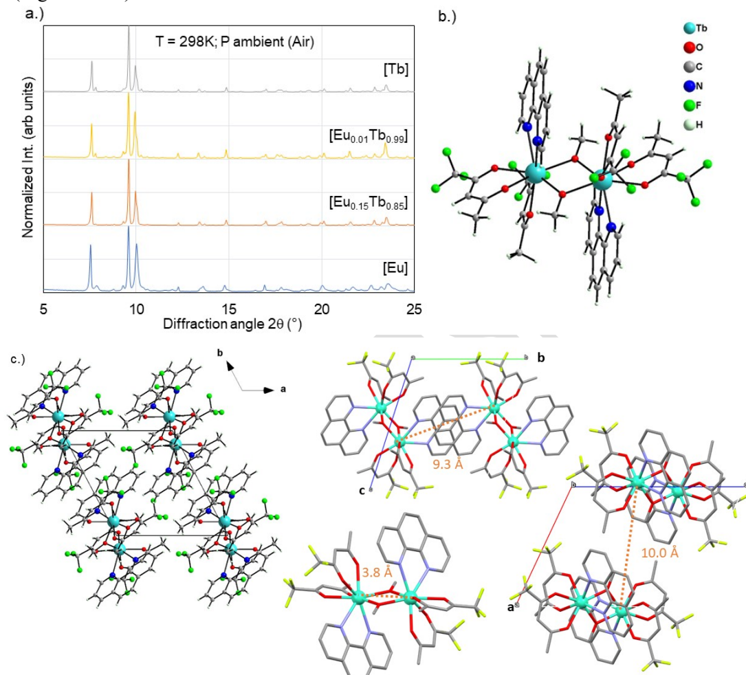
Figure 2.16: a) X-Ray diffraction patterns of [Ln_2(\mu\text{-OMe})_2(\text{tfa})_4(\text{phen})_2] with different compositions. b) Molecular structure of [Tb_2(\mu\text{-OMe})_2(\text{tfa})_4(\text{phen})_2] . c) Distances between the Ln atoms in the complex [Tb_2(\mu\text{-OMe})_2(\text{tfa})_4(\text{phen})_2] .
