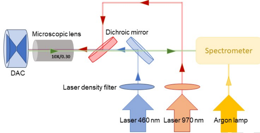
Scheme 3.2: Experimental set-up of DAC-coupled to the spectrometer
