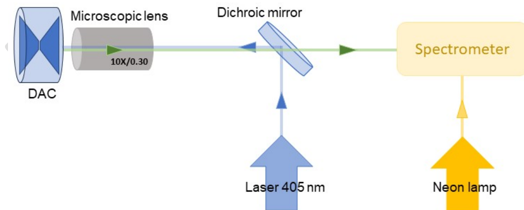
Figure 4.1: Schematic description of pressure coupling spectrometer.
