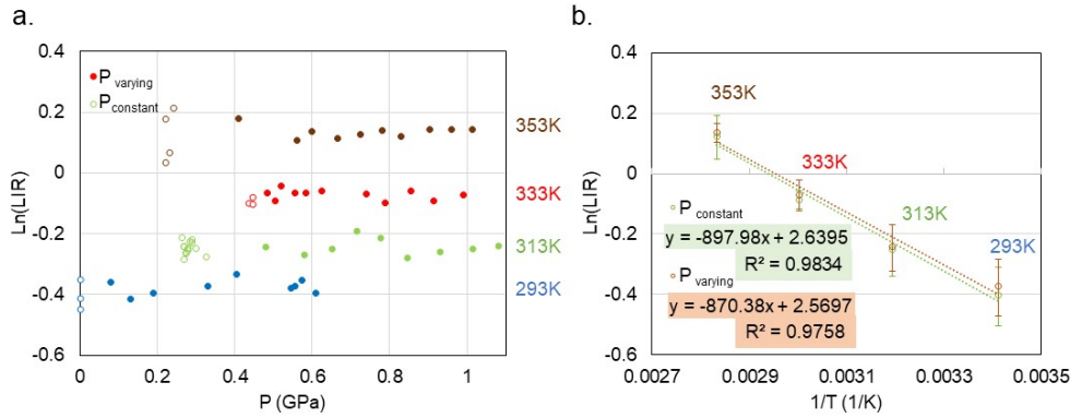
Figure 3.16: \text{GdVO}_4:\text{Yb}^{3+}/\text{Er}^{3+} suspended at 0.5 wt.% upon NIR laser at 13.5 \text{ W}/\text{cm}^2 : a) Distribution of \text{Ln}(\text{LIR}) values at four temperature (293 to 353 K) under constant pressure (hollow point) and pressure varying up to 1.1 GPa (solid point). b) Temperature calibration curve and the fitted trendline equations under constant pressure (green) and pressure varying (brown), error bars determined by the standard deviation of overall data.
