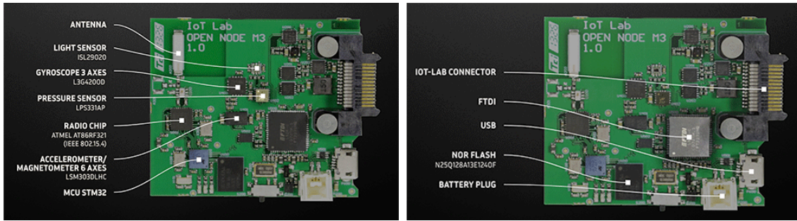
Figure 6.5: M3-board Micro-Controller Components [99].
