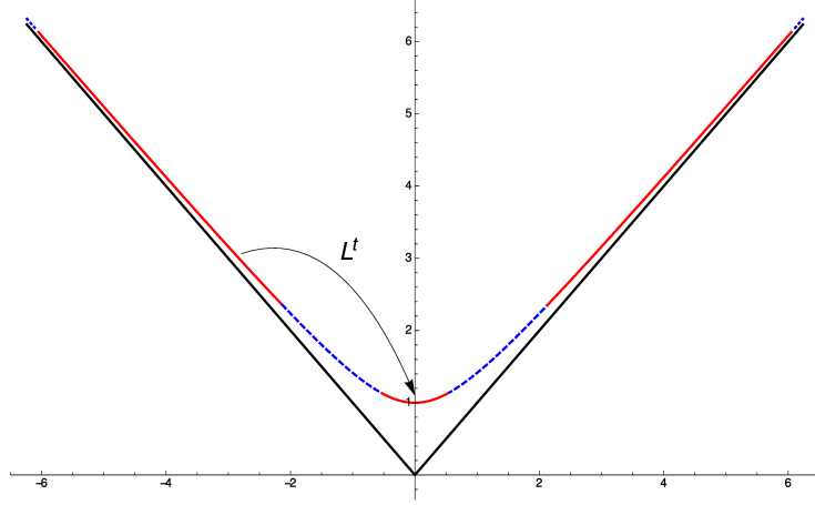
FIGURE 6. The one-dimensional cap movement: a carefully chosen Lorentz boost L^t : (\tau, \xi) \mapsto (1 - t^2)^{-1/2}(\tau + t\xi, \xi + t\tau) interchanges the caps. Here, L^t(\mathcal{C}_{-2}) = \mathcal{C}_0 for t = \tanh(2) .
