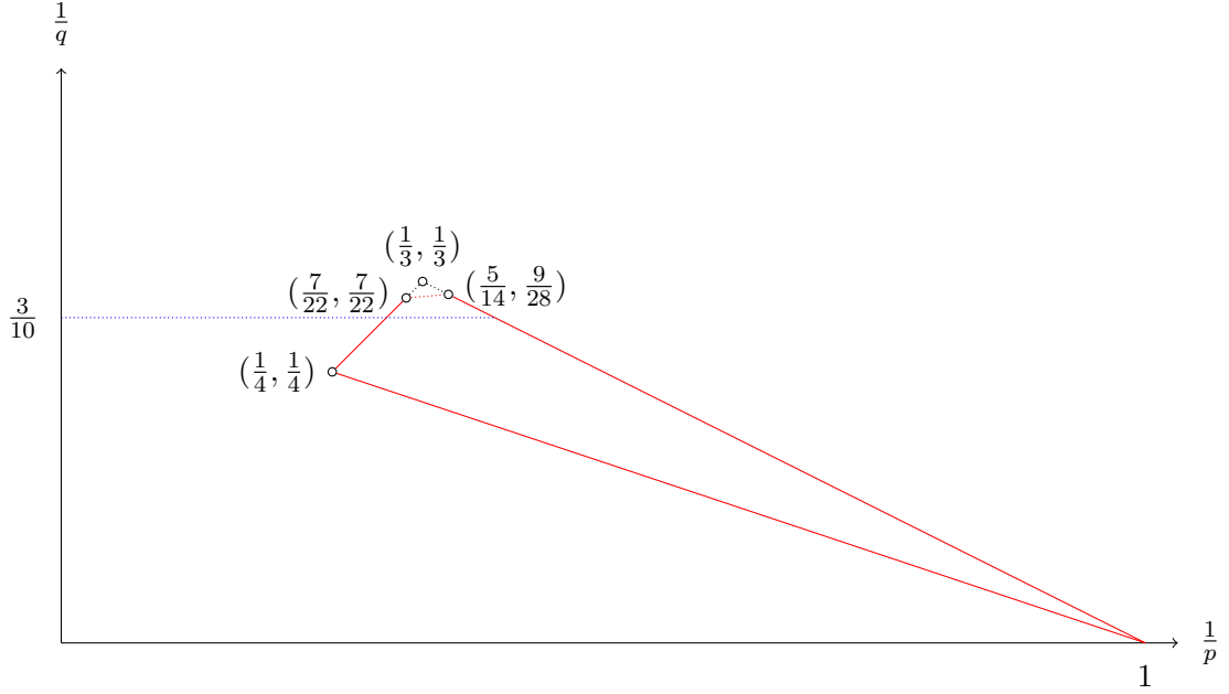
FIGURE 7. By Theorem 39, the full restriction conjecture for the low frequency region would imply global restriction estimates for exponent pairs (p^{-1}, q^{-1}) within the red quadrilateral. Unconditional estimates hold in the bilinear range q > \frac{10}{3} .
