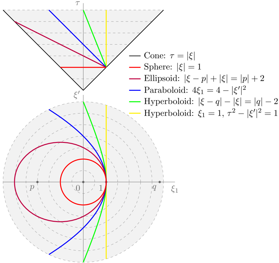
FIGURE 1. Spheres (§5), paraboloids (§6.2), cones (§6.3), and hyperboloids (§7) can all be obtained as conic sections.
