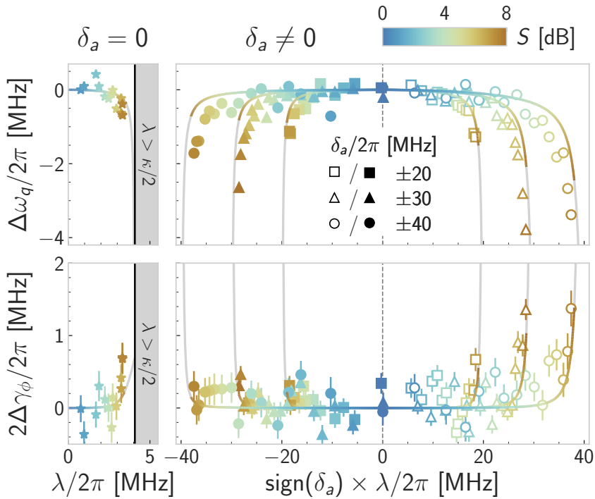
Figure 3.13 Spectral response of a qubit interacting with a DPO. Left: The pump frequency is set to \omega_p = 2\omega_a . Top (Bottom): qubit frequency shift (induced dephasing) versus pump amplitude (x-axis). The data (stars) are fitted with analytical expressions (solid lines) adapted from [Eddins 2019] (section 3.3). The shaded area marks the instability region. Right: same as left panels with the pump frequency set to \omega_p = 2\omega_a - 2\delta_a , where \delta_a/2\pi \in \{\pm 20, \pm 30, \pm 40\} MHz. The solid lines correspond to Eqs. 3.64a and 3.65a with not fit parameter. A common colormap for the left and right panels maps the pump amplitude to an equivalent squeezing (steady-state anti-squeezing) for \delta_a \neq 0 ( \delta_a = 0 ) in decibels.
