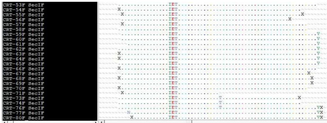
Figure 4. Alignment of pfert gene sequences (2).
