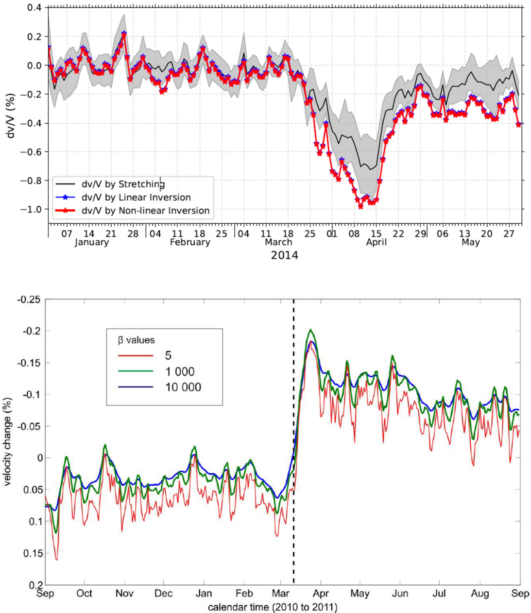
Fig. 2-16: (top) Comparison of an inverted dv/v time series with the standard stretching method, and (bottom) different time series obtained, depending on \beta the characteristic length of correlation between the model parameter \delta v . From (Machacca et al., 2017) and (Brenquier et al., 2014, supp. material), respectively.
