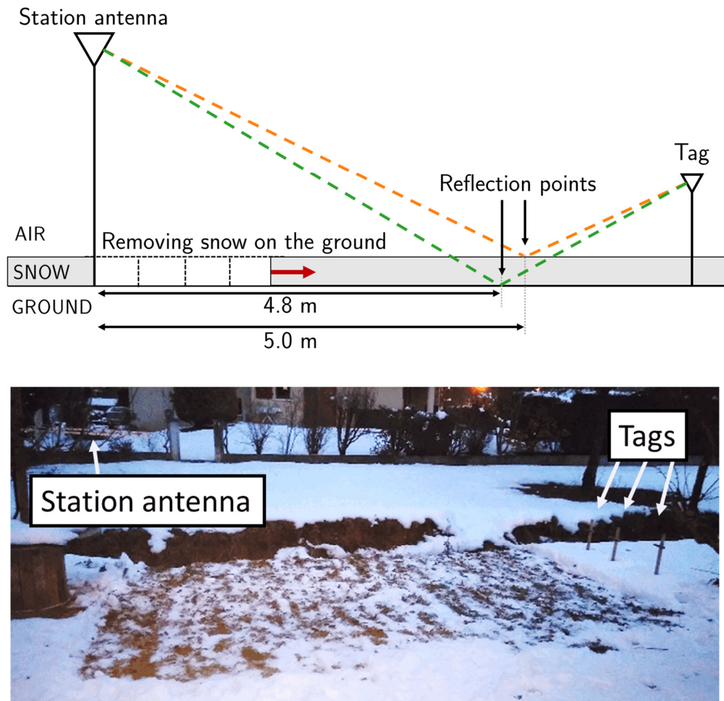
Fig. 5-24: (top) sketch and (bottom) picture of the experiment of removing snow on the ground
