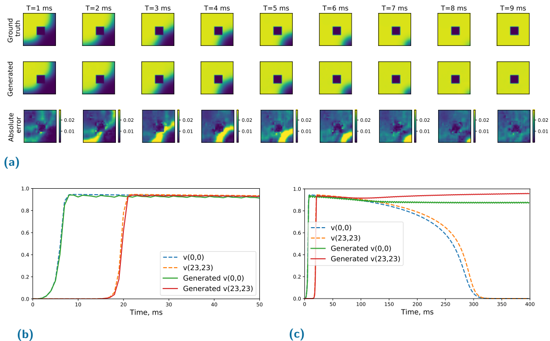
Fig. 2.4: (a) Representative results for the trained EP-Net 2.0 model (9 ms of forecast, conductivity of the cardiac slab tissue \sigma = 2 ). (b,c) Plots of the transmembrane potential at the leftmost upper point (0,0) and the rightmost bottom point (23,23) in the slab with different forecasting horizons.
