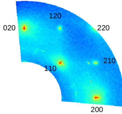
Figure 2.15: Example of in-plane GIXRD
