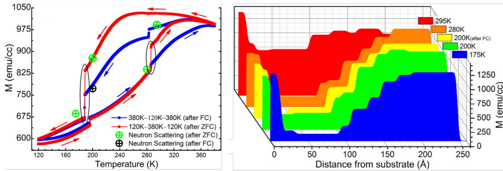
Figure 1.23: FeRh magnetic moment at different depth and temperature
