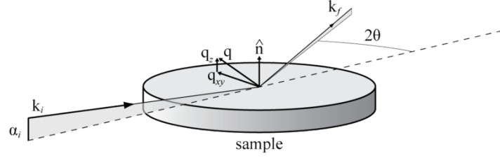
Figure 2.14: Scheme of GIXRD
