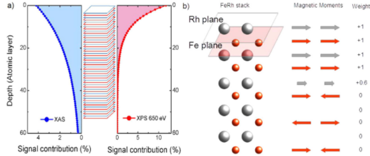
Figure 1.7: FeRh(001) magnetization at different depths
