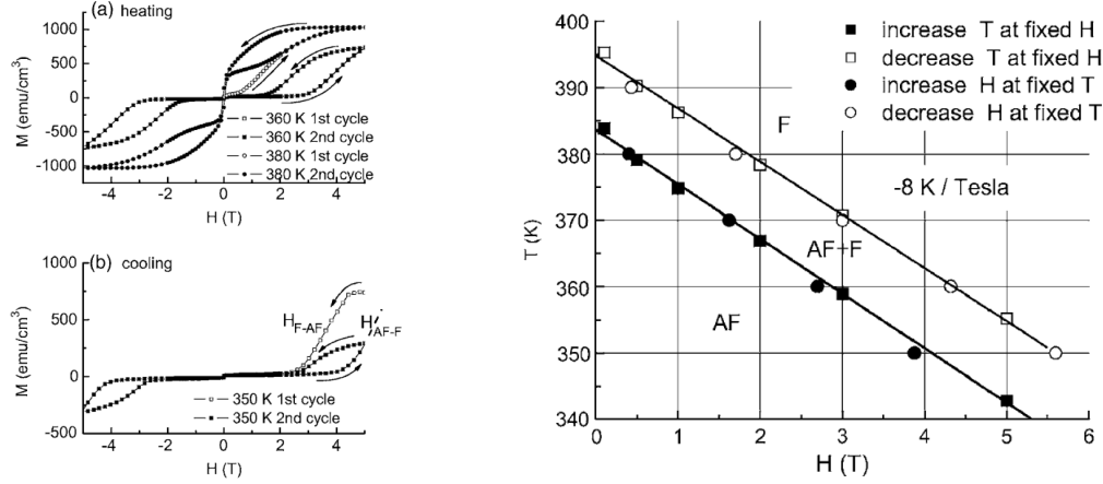
Figure 1.6: Magnetization for 110 nm FeRh film over MgO.
