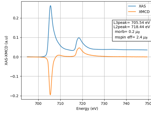
Figure D.2: XMCD for FeRh embeded in carbon matrix in grazing incidence configuration.
