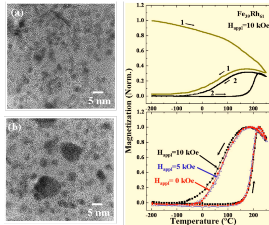
Figure 1.16: FeRh nanoparticles and metamagnetic transition
