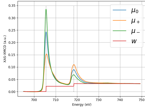
Figure 2.12: Spectres used for XAS/XMCD at Fe edge
