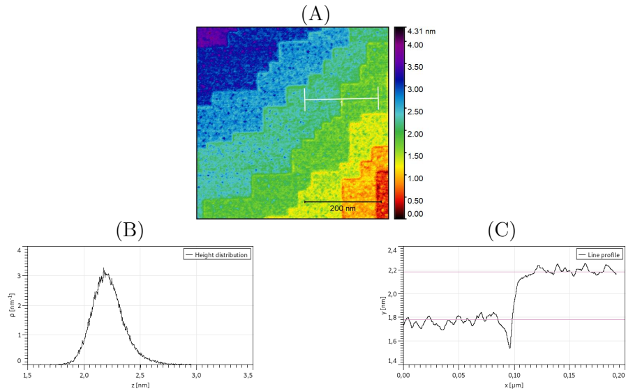
Figure 5.2: Atomic force microscopy image of a STO substrate after pre-annealing at PLRYA.
