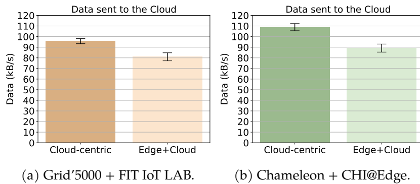
Figure 7.6 – Amount of data sent to the Cloud regarding the Cloud-centric and Edge + Cloud processing approaches.
