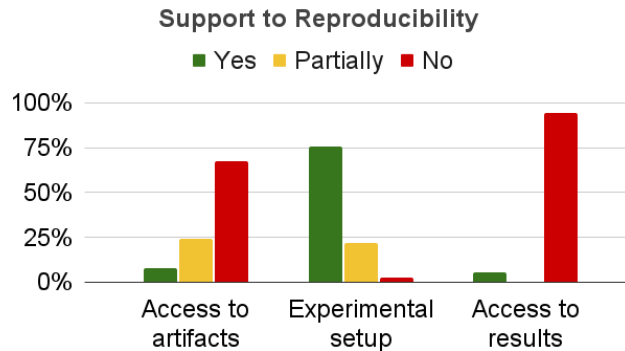
Figure 7.2 – Support to the reproducibility of Edge-to-Cloud experiments provided by the selected studies in our survey [175].
