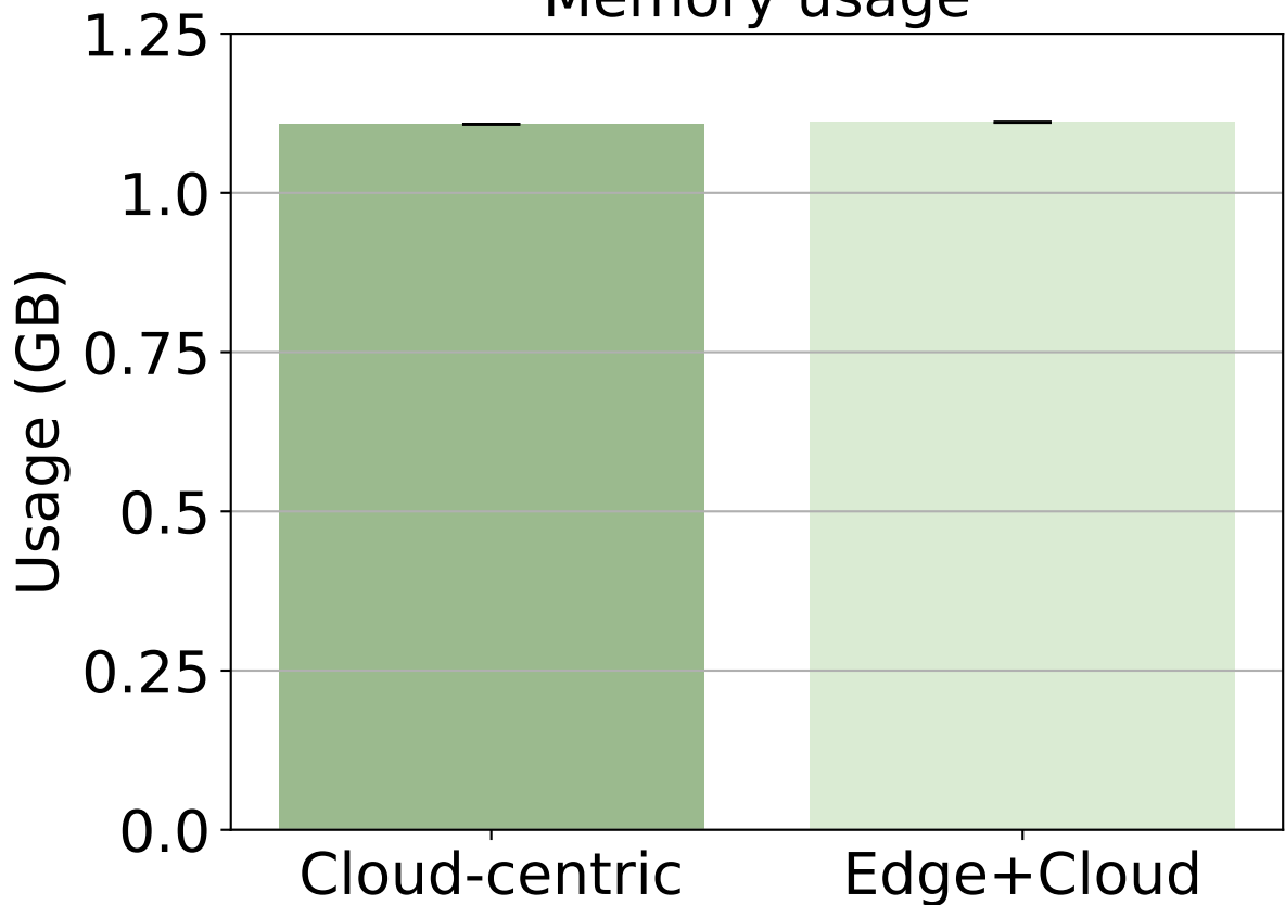
Memory usage
