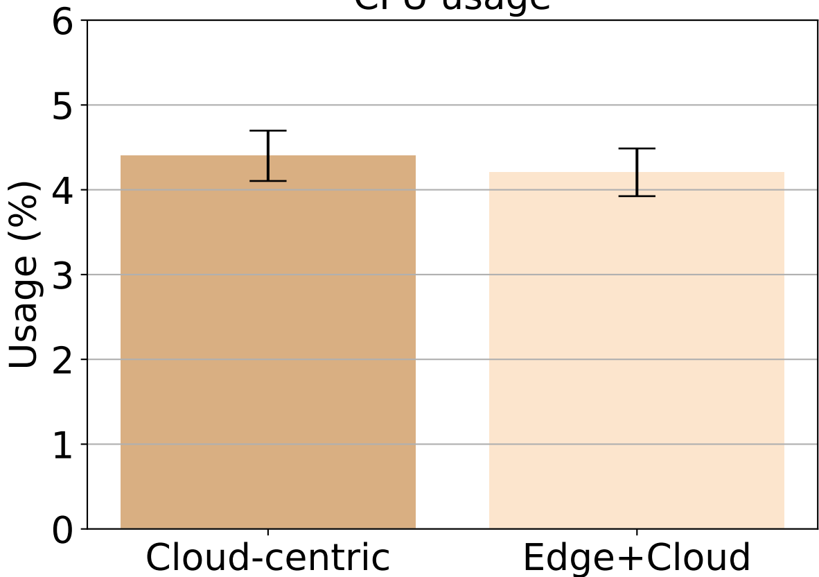
CPU usage
