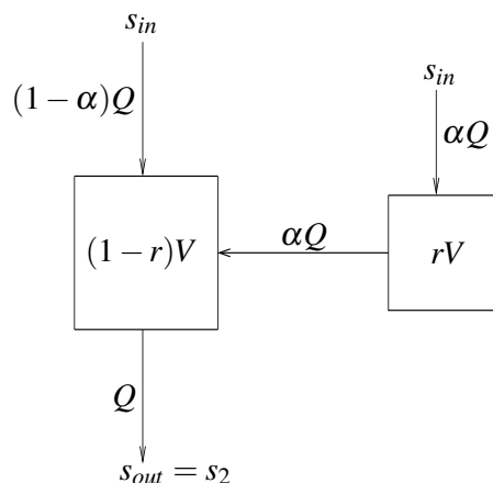
Figure 3.4: The buffered chemostat.
