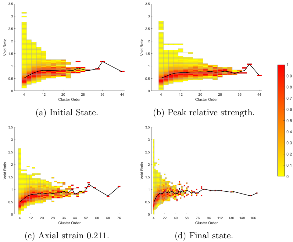
Figure B.10: Void ratio density map in function of cluster order for the test U100 a the initial state, peak relative strength, and final state. Point density is calculated in relation to the rectangle containing the maximum number of points for each order. The black curve represents the mean value.
