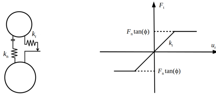
(a) Illustration of contact springs. (b) Limitation of tangential spring force.
