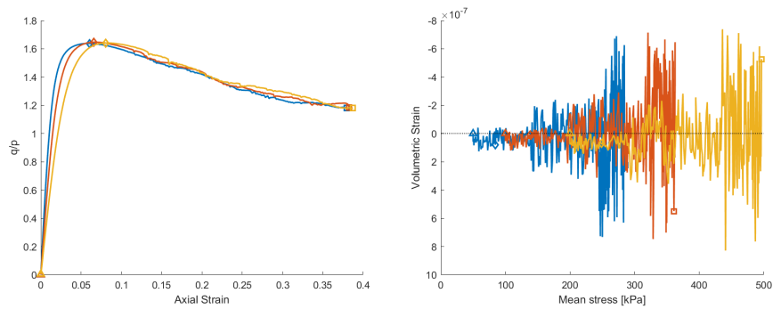
(d) Relative strength vs axial strain. (e) Volumetric strain vs mean stress.
