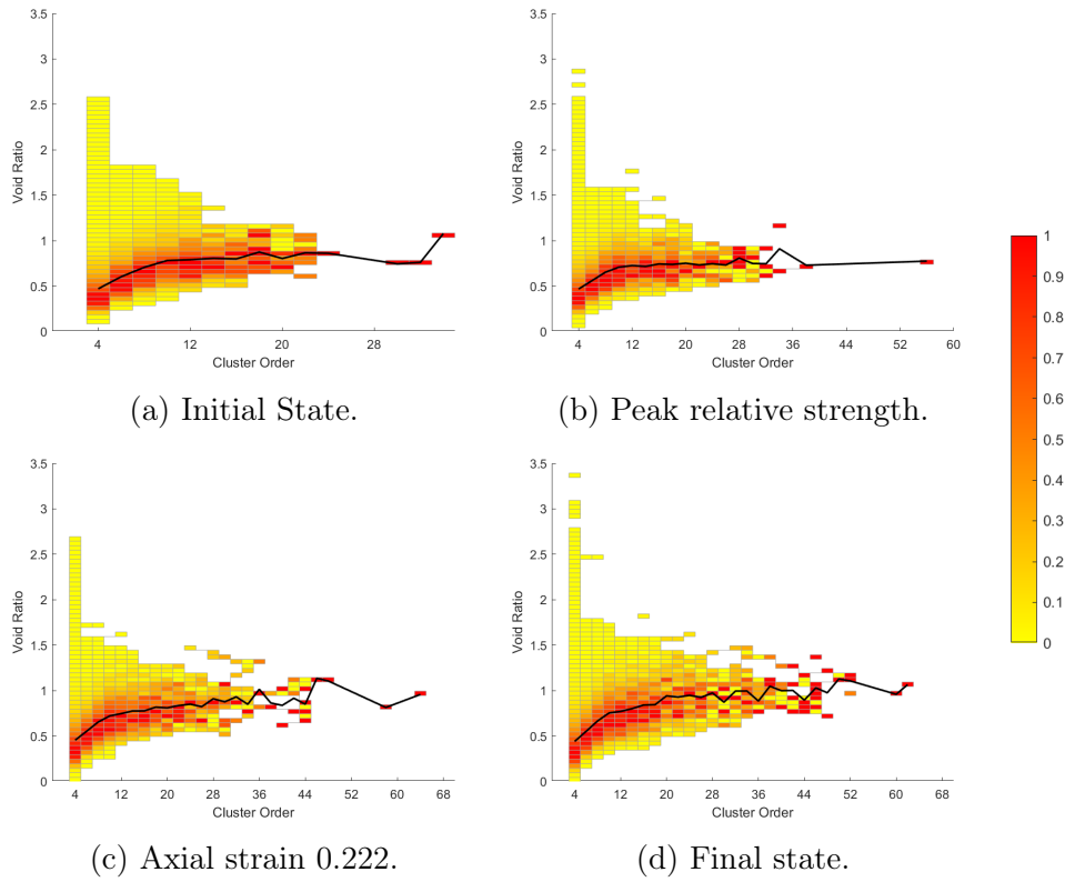
Figure B.11: Void ratio density map in function of cluster order for the test U200 a the initial state, peak relative strength, and final state. Point density is calculated in relation to the rectangle containing the maximum number of points for each order. The black curve represents the mean value.
