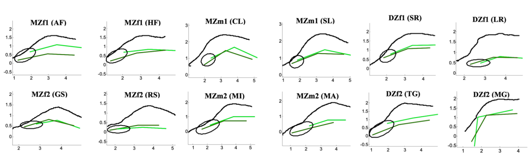
Figure 2.4: Figures 4 and 5 from [Weirich and Fuchs, 2013] combined. Mean articulatory target positions of /s/ (dark green) and /ʃ/ (light green). Different plots show different speakers. Ellipses visualise the amount of (horizontal and vertical) variation of the tongue tip. No ellipse is drawn for speaker DZf2 since she did not seem to use the tongue tip.
