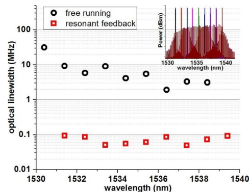
Figure 25: Optical linewidth as a function of wavelength. Inset : Optical spectrum measurement values below 100 kHz. This first demonstration opened the way for several other investigations
