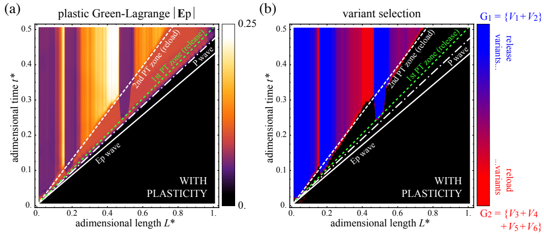
FIGURE 2.14: (a) Slice-averaged magnitude of the plastic Green-Lagrange strain tensor \mathbf{E}_p in the Lagrangian adimensional position-time (L^*, t^*) diagram from simulation with plasticity. The elastic and plastic wave fronts with constant velocities are shown using different line types as well as two (primary and secondary) phase-transition zones that are associated with specific nucleation of release and reload variants (see text for details). (b) The corresponding selection of hcp variants, categorized into two groups, so-called G_1 = \{V_1 + V_2\} (in blue) and G_2 = \{V_3 + V_4 + V_5 + V_6\} (red).
