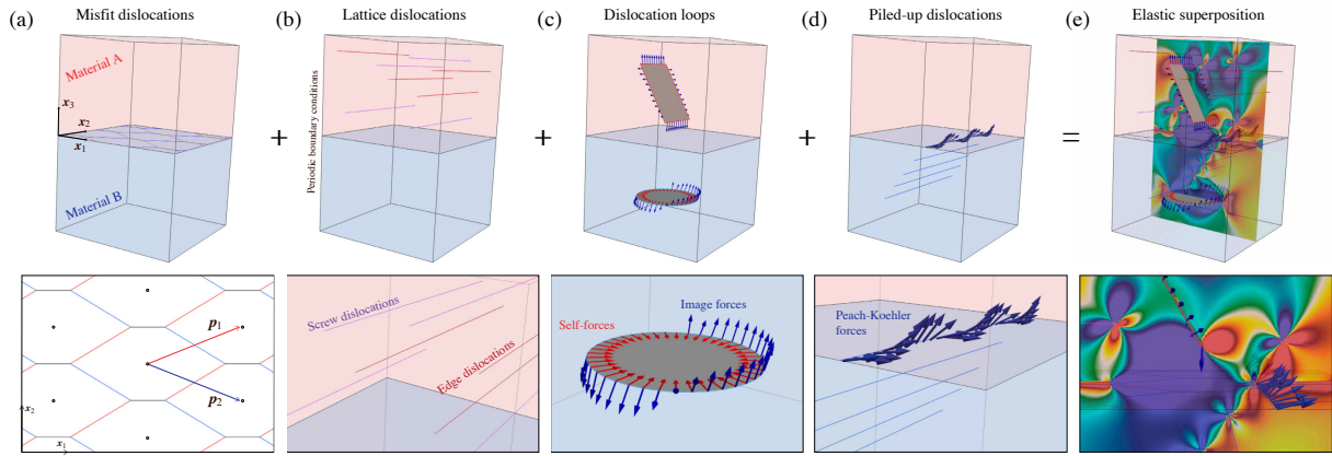
FIGURE 3.34: Linear superposition scheme of elastic field solutions in dissimilar anisotropic materials due to the presence of (a) misfit dislocation patterns at the heterophase interfaces, (b) infinite long straight lattice dislocations in the upper material A, (c) arbitrary polygonal and elliptical dislocation shear or prismatic loops in both crystals, (d) piled-up dislocation arrays onto specific glide planes in the lower material B. For each dislocation problem, the insets show particular features that are explained in the text. The three-dimensional applied stresses, internal stresses, image as well as self-stresses are superposed in (e) to compute some interaction force distributions on defects, as illustrated in the insets of (c) and (d).
