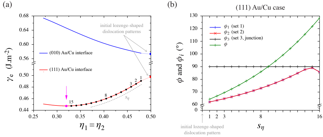
FIGURE 3.28: (a) Dependence on \eta_1 = \eta_2 of the elastic energy \gamma_e in \text{J}\cdot\text{m}^{-2} , i.e. along the bisecting lines of the admissible triangular domains \mathcal{T}_{ABC} , as displayed in Figs. (3.27). The blue and the red curves correspond to the mismatched (010) and (111) Au/Cu interfaces, respectively. The latter exhibits black dots, indexed by s_\eta = 1, \dots, 16 , which represent the minimum-energy path from Fig. (3.27b). The large points at \eta_1 = \eta_2 = 1/2 are related to the initial lozenge-shaped patterns with two crossing sets of dislocations, whereas the vertical arrow shows the minimum-energy configuration associated with the (111) semicoherent interface. (b) Dependence on s_\eta of the dislocation characters \phi_i for the three sets and the angle \phi between the two parent dislocations for the corresponding (111) Au/Cu case. All these quantities are expressed in ^\circ .
