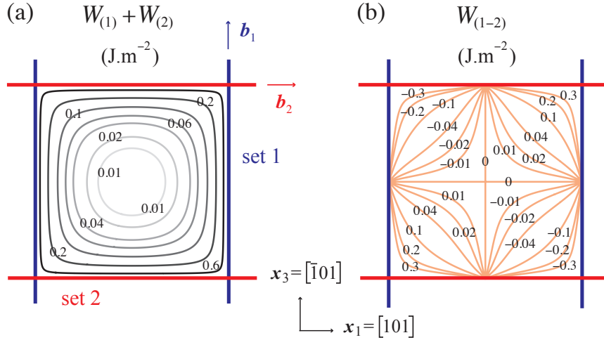
FIGURE 3.8: Local (a) self- \{W_{(1)} + W_{(2)}\} and (b) interaction W_{(1-2)} elastic energies arising from two sets of orthogonal screw dislocations in a 2^\circ twist boundary on a (010) plane in Cu.
