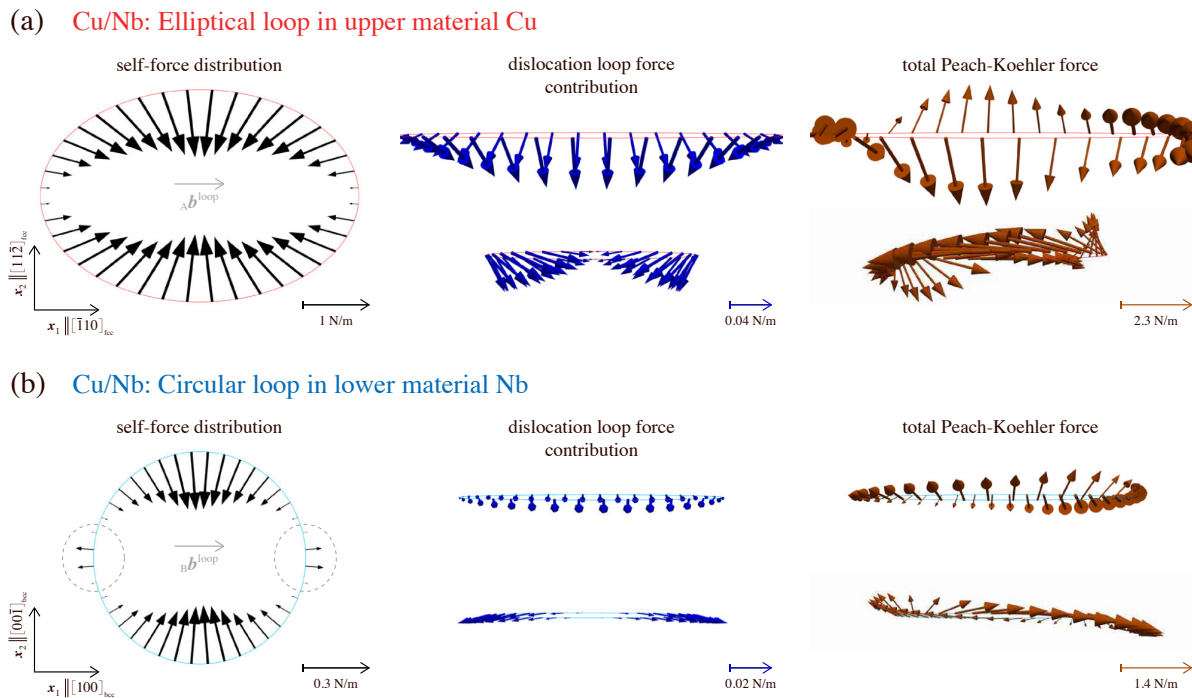
FIGURE 3.39: Discrete distribution of the local forces (black arrows), of the dislocation loop forces (blue) that include the corresponding full-space solutions and complementary (image) contributions of the loops, and of the complete Peach-Koehler forces (orange), which act along both shear dislocation loops. These force distributions are exerted on the elliptical dislocation loop in Cu (a) and on the circular loop in Nb (b). For both shear dislocation loops, the associated fcc and bcc Burgers vectors lie along the x_1 -axis. The dotted two small circles in (b) illustrates the local self-stress expansion of the loop in the lower material Nb by the near-edge (since the local character between the Burgers vector and the local tangent is characterized by \alpha in Fig. (3.38)) character elements.
