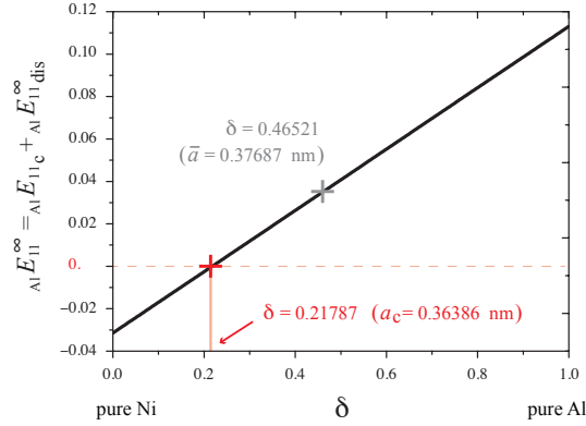
FIGURE 3.10: Dependence of the total far-field strain component \text{Al} \mathbf{E}_{11}^\infty in Al on \delta for a Al/Ni heterophase interface. The red dotted line gives the unique reference state, for which the far-field decay to zero and the coherent parameter a_c is defined. The lattice parameter \bar{a} = 2a_{\text{Al}} a_{\text{Ni}} / (a_{\text{Al}} + a_{\text{Ni}}) , which is a good approximation for an interface between crystals of different lattice parameters but identical elastic constants [93, 131], is marked by a grey cross symbol.
