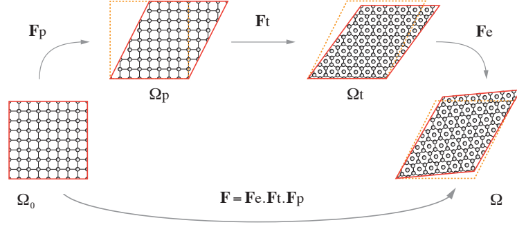
Figure 2.1: Schematics of the reference \Omega_0 , intermediate, \Omega_p and \Omega_t , and, current \Omega configurations, for which the total deformation gradient tensor \mathbf{F} is decomposed multiplicatively into plastic \mathbf{F}_p , transformational \mathbf{F}_t and elastic \mathbf{F}_e distortions.
