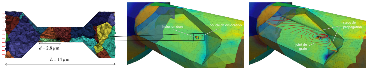
Figure 4.4: From the initial dislocation loop embedded in a given grain of the polycrystalline copper micropillar with \sim 193\text{k} degrees of freedom in (a) to the various propagation steps followed by the shear dislocation loop in (b), thus leaving residual dislocation edges around the bypassed heterophase precipitate. The final computational mesh involves \sim 1007\text{k} degrees of freedom.
