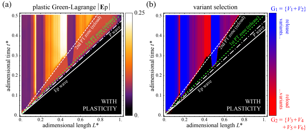
Figure 2.14: (a) Slice-averaged magnitude of the plastic Green-Lagrange strain tensor \mathbf{E}_p in the Lagrangian adimensional position-time ( L^* , t^* ) diagram from simulation with plasticity. The elastic and plastic wave fronts with constant velocities are shown using different line types as well as two (primary and secondary) phase-transition zones that are associated with specific nucleation of release and reload variants (see text for details). (b) The corresponding selection of hcp variants, categorized into two groups, so-called G_1 = \{V_1 + V_2\} (in blue) and G_2 = \{V_3 + V_4 + V_5 + V_6\} (red).
