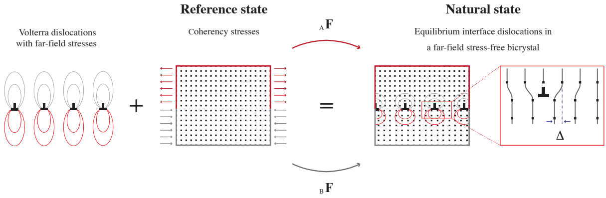
Figure 3.1: Mapping from a coherent reference state to the natural state using displacement gradients {}_A\mathbf{F} and {}_B\mathbf{F} . Volterra dislocations introduced into the reference state remove coherency stresses and may change the misorientation of the neighboring crystals.
