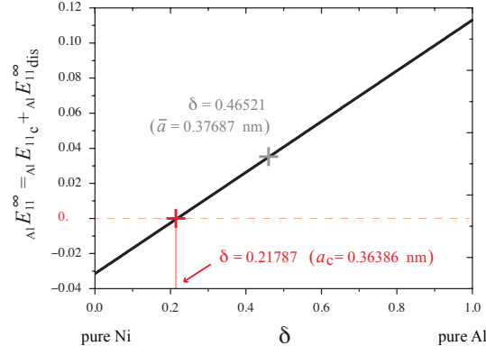
Figure 3.10: Dependence of the total far-field strain component {}_{\text{Al}}E_{11}^{\infty} in Al on \delta for a Al/Ni heterophase interface. The red dotted line gives the unique reference state, for which the far-field decay to zero and the coherent parameter a_c is defined. The lattice parameter \bar{a} = 2a_{\text{Al}}a_{\text{Ni}} / (a_{\text{Al}} + a_{\text{Ni}}) , which is a good approximation for an interface between crystals of different lattice parameters but identical elastic constants [94, 135], is marked by a grey cross symbol.
