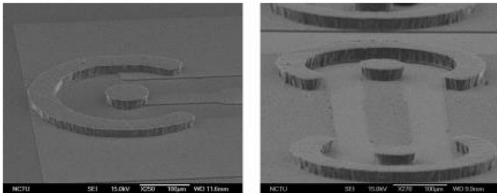
Figure 20. Coaxial flip-chip structure as presented in [21] ©2010 IEEE
