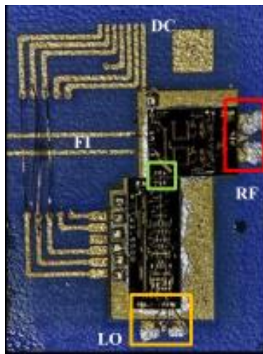
Figure 62. D-band receiver module containing MMICs from Gotmic
